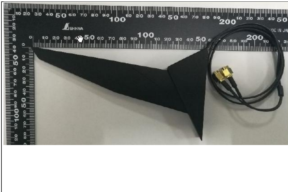
Antenna (Brand: INPAQ, Model No.: DAM-J7-H-DL-065-10-34)
