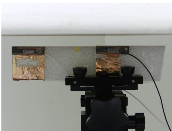
Bottom Side, Test Separation 0.98 cm
