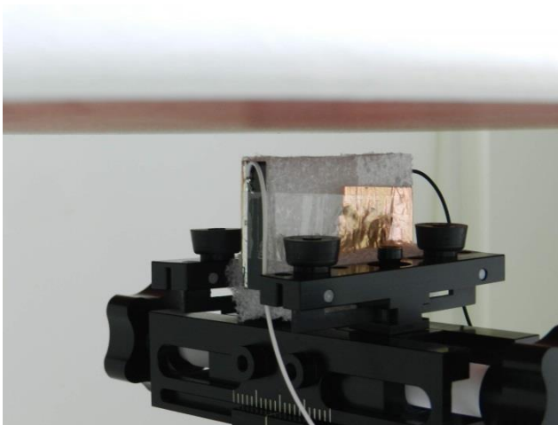
Right Side Test Separation 0.98 cm
