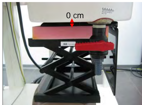
Fig.3 EUT Laptop mode to flat phantom
