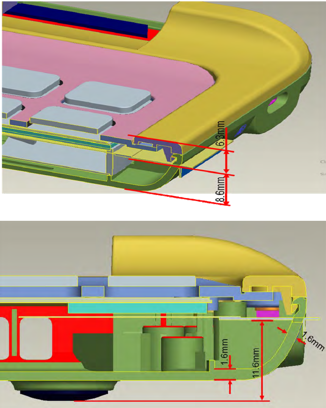
Fig.8 Aux Antenna position of EUT
