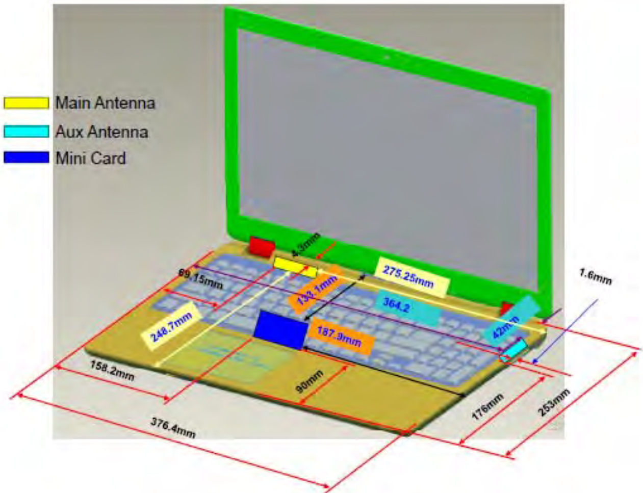
Fig.6 Antenna position of EUT
