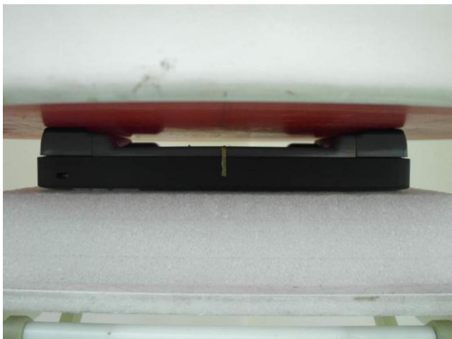
Bottom Face with Phantom 0 cm Gap (DUT with Battery 1)
