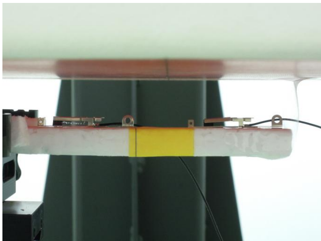
Antenna Horizontal Up with Phantom 2 cm Gap
