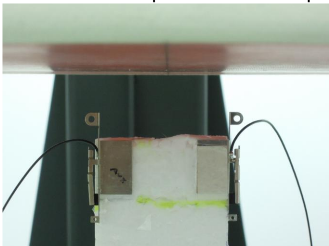
Antenna Vertical Up with Phantom 2 cm Gap
