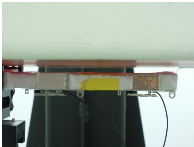
Antenna Horizontal Down with Phantom 2 cm Gap
