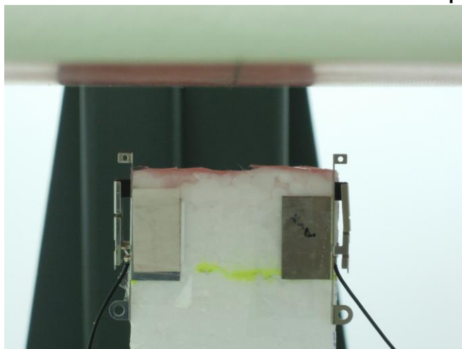
Antenna Vertical Down with Phantom 2 cm Gap
