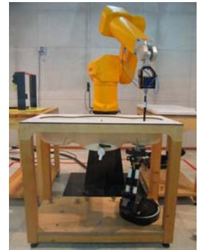
Figure 1. SAR System
