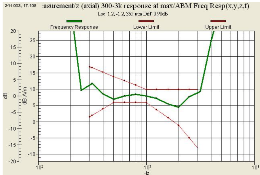
Graph 4 : PCS 1900 (CH 25) Frequency Response (Keypad)
