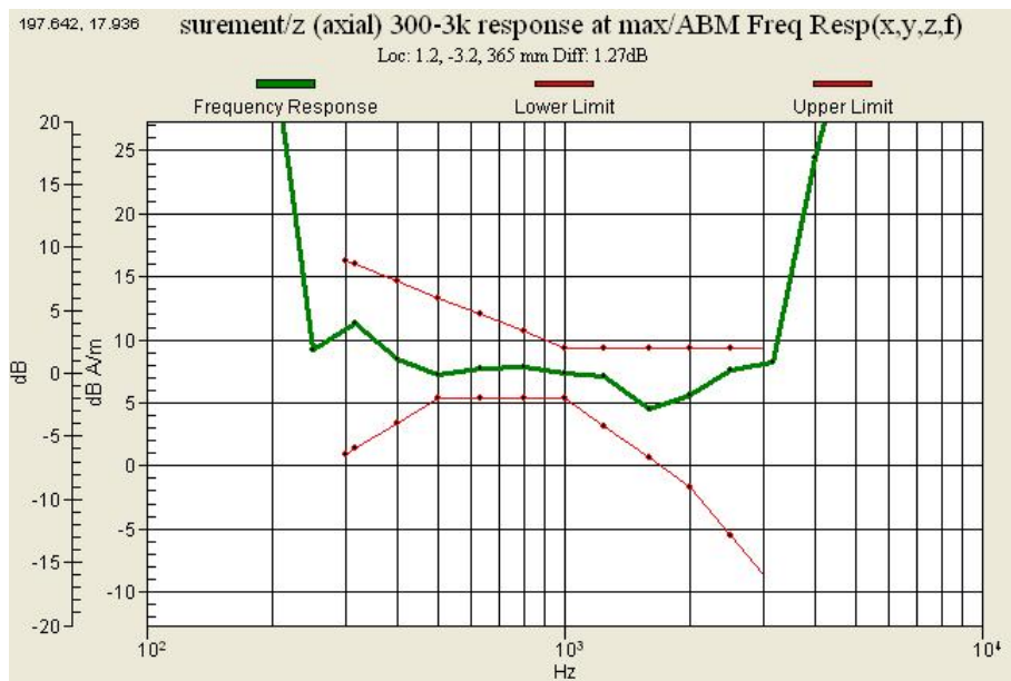
Graph 8 : CDMA 800 (CH 384) Frequency Response (Speaker)
