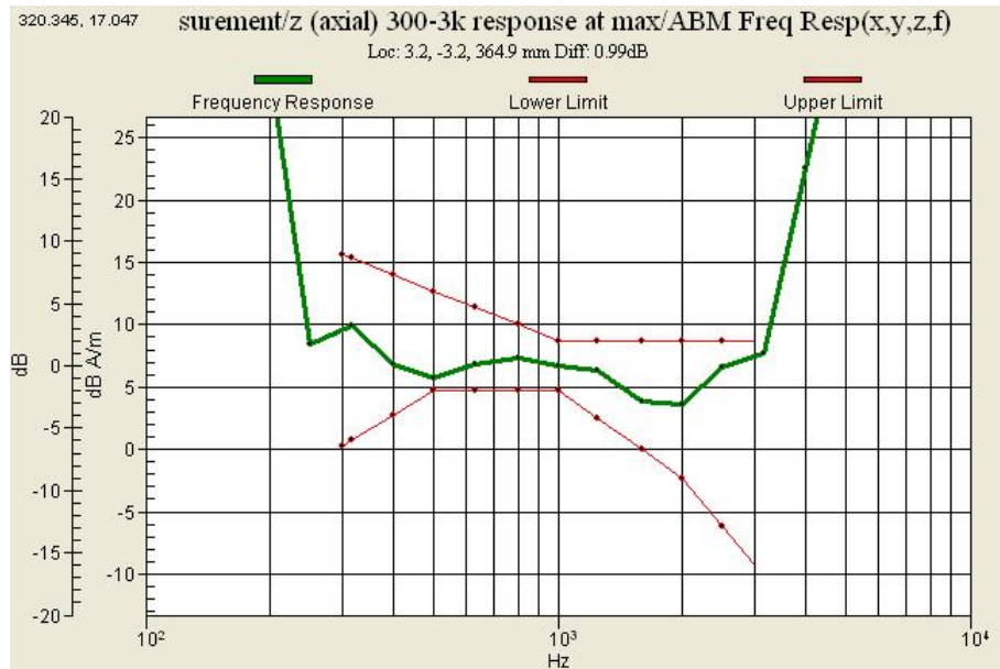
Graph 6 : PCS 1900 (CH 1175) Frequency Response (Keypad)
