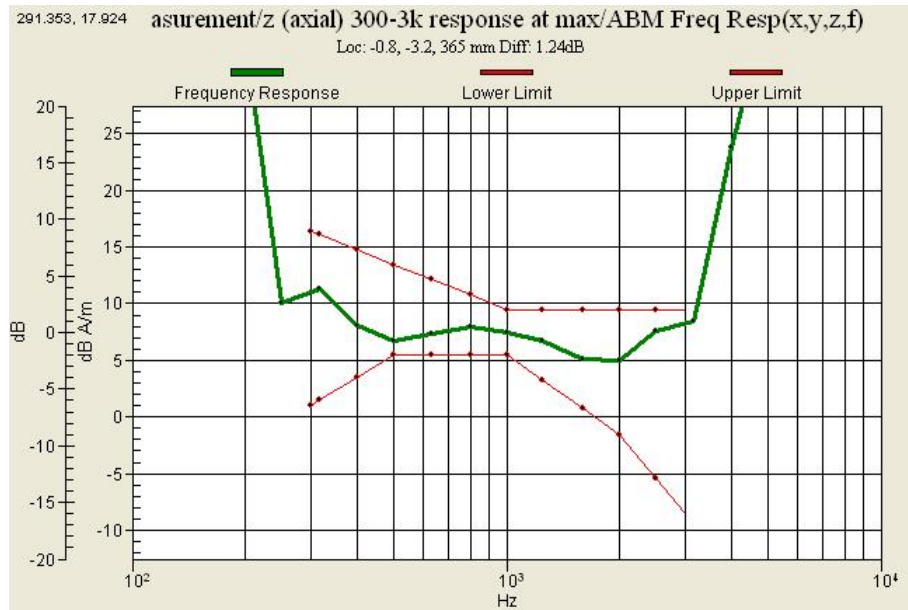
Graph 5 : PCS 1900 (CH 600) Frequency Response (Keypad)
