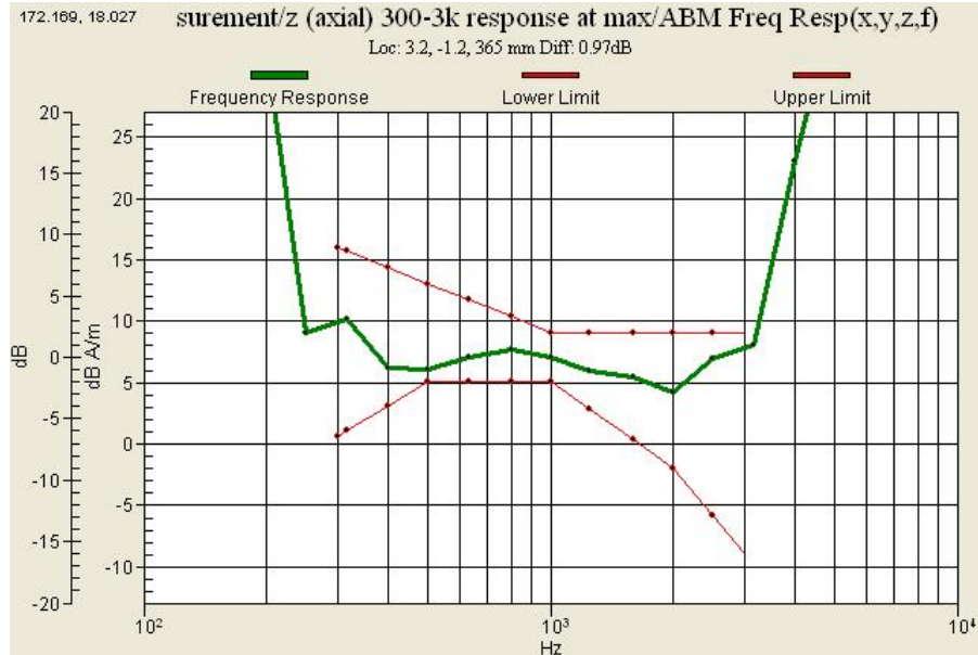
Graph 1 : CDMA 800 (CH 1013) Frequency Response (Keypad)
