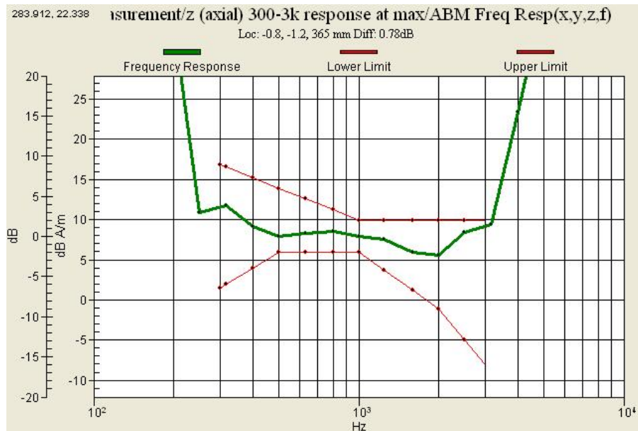
Graph 10 : PCS 1900 (CH 25) Frequency Response (Speaker)
