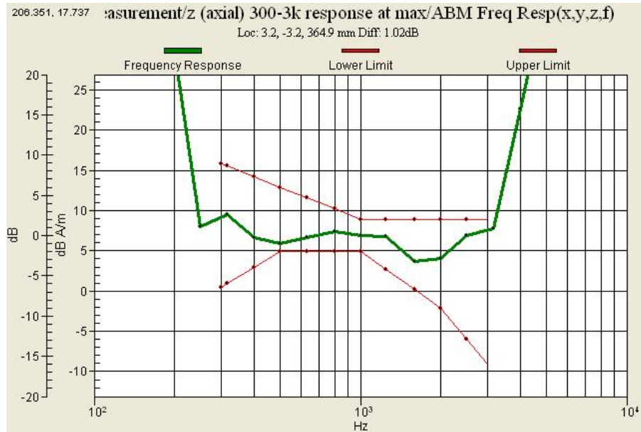
Graph 3 : CDMA 800 (CH 777) Frequency Response (Keypad)
