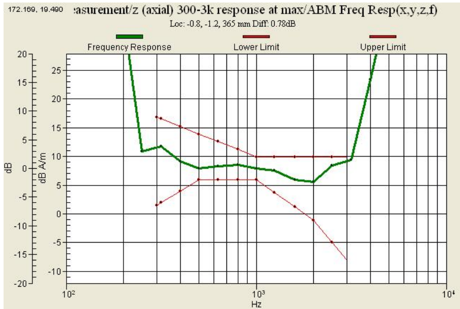
Graph 12 : PCS 1900 (CH 1175) Frequency Response (Speaker)
