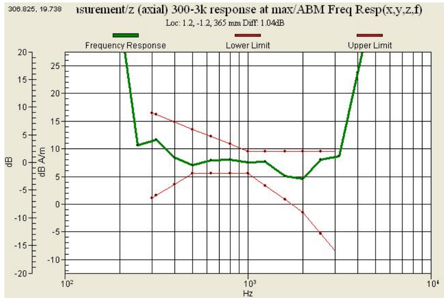
Graph 7 : CDMA 800 (CH 1013) Frequency Response (Speaker)
