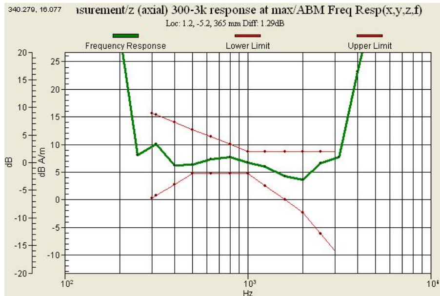
Graph 2 : CDMA 800 (CH 384) Frequency Response (Keypad)
