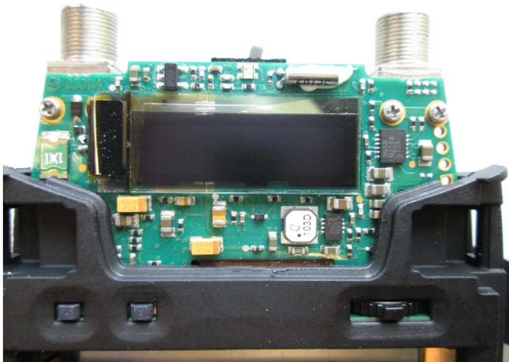
Main board of EUT #T1541593, top
