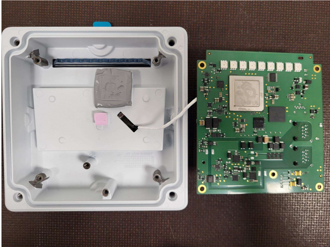
Back view of EUT and main PCB other side.
