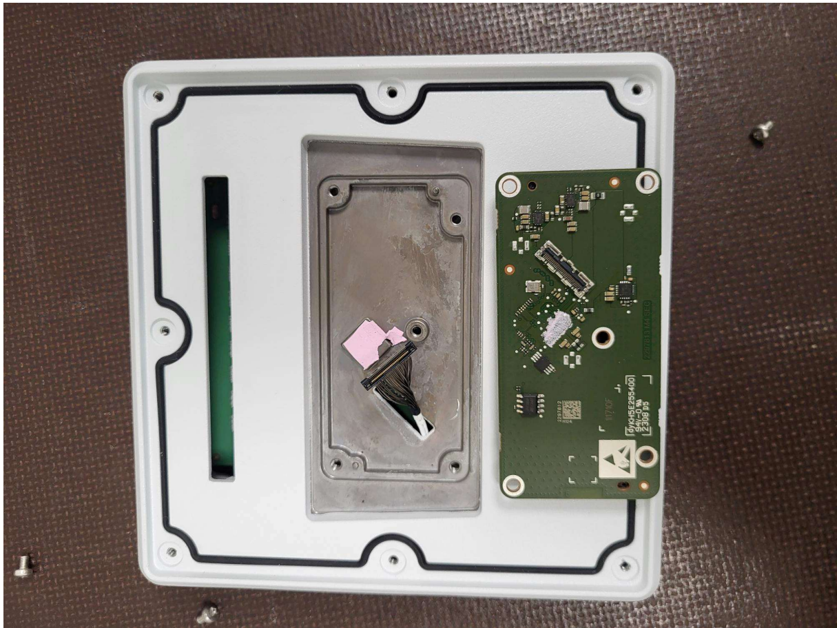
Front view of EUT and back view of RF PCB without radome
