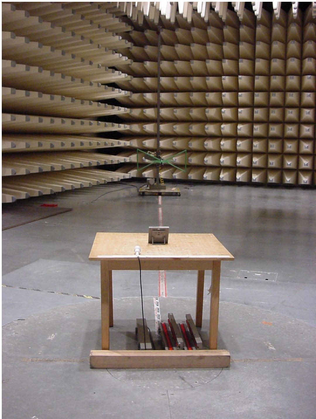
Photo 1 (Radiated Emissions):
