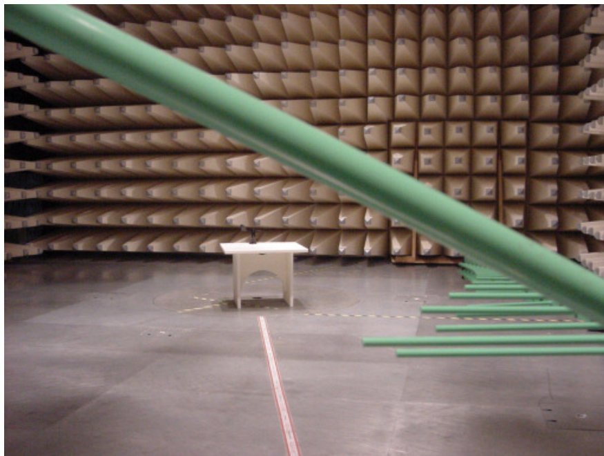
Photo 6 (Radiated Emissions):
