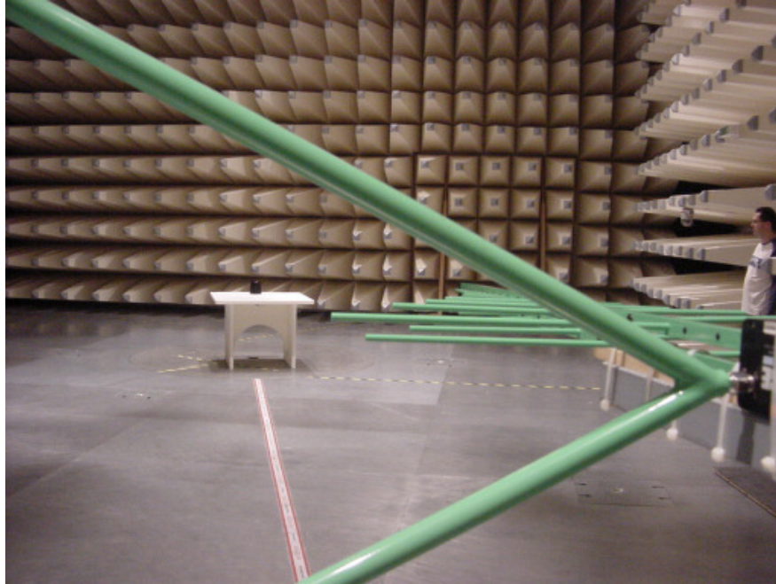
Photo 4 (Radiated Emissions):
