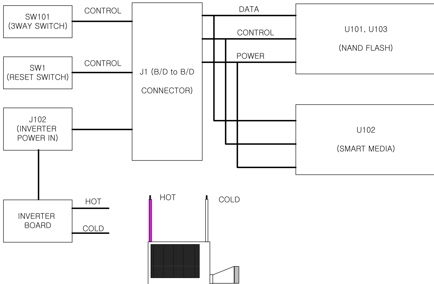
BOTTOM BOARD BLOCK DIAGRAM
