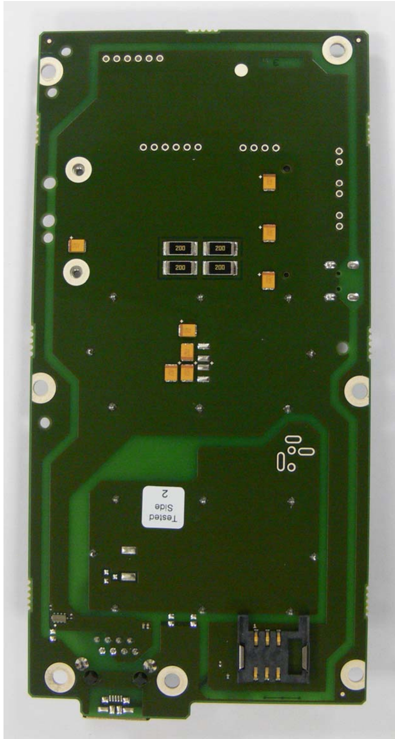
Figure 5: PoE Adapter Board – rear
