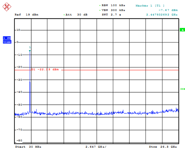
Fig.19 Conducted spurious emission: Ch39, 2480MHz
