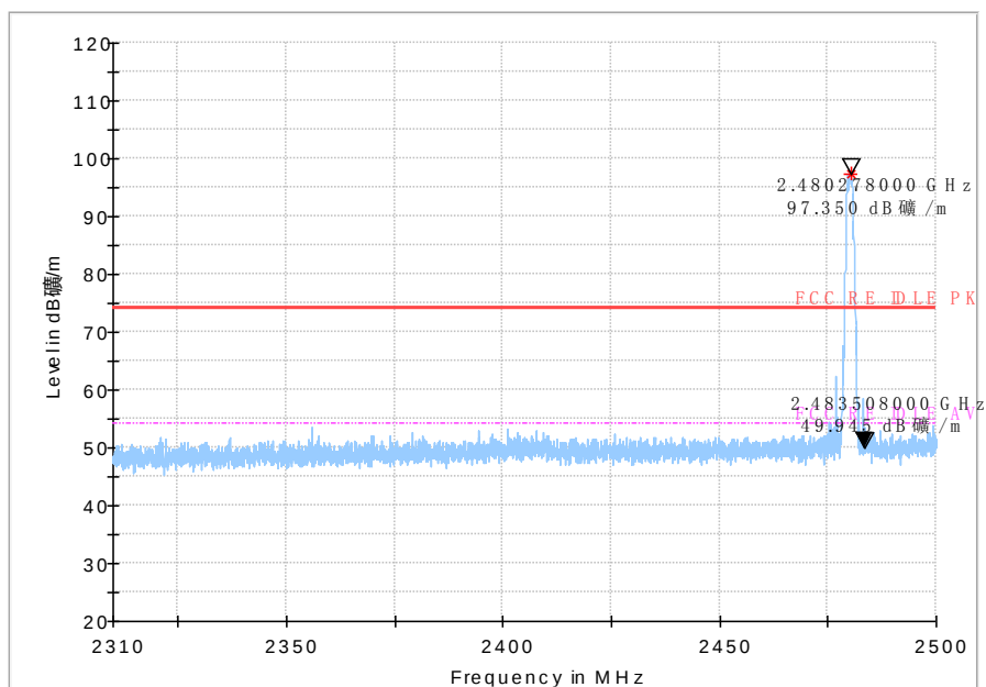
Fig.28 Bandedge:ch39
