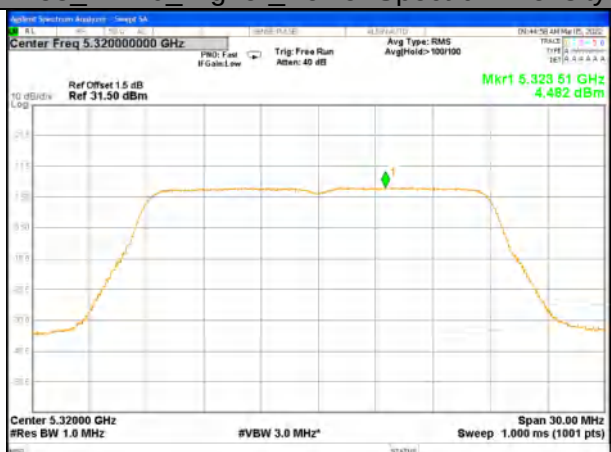
W53_11n20_Higher_Power Spectrum Density
