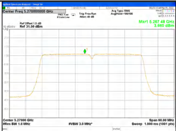
W53_11ac40_Lower_Power Spectrum Density
