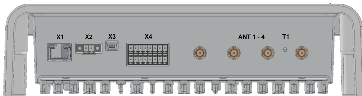
Figure 2: Connection Overview
