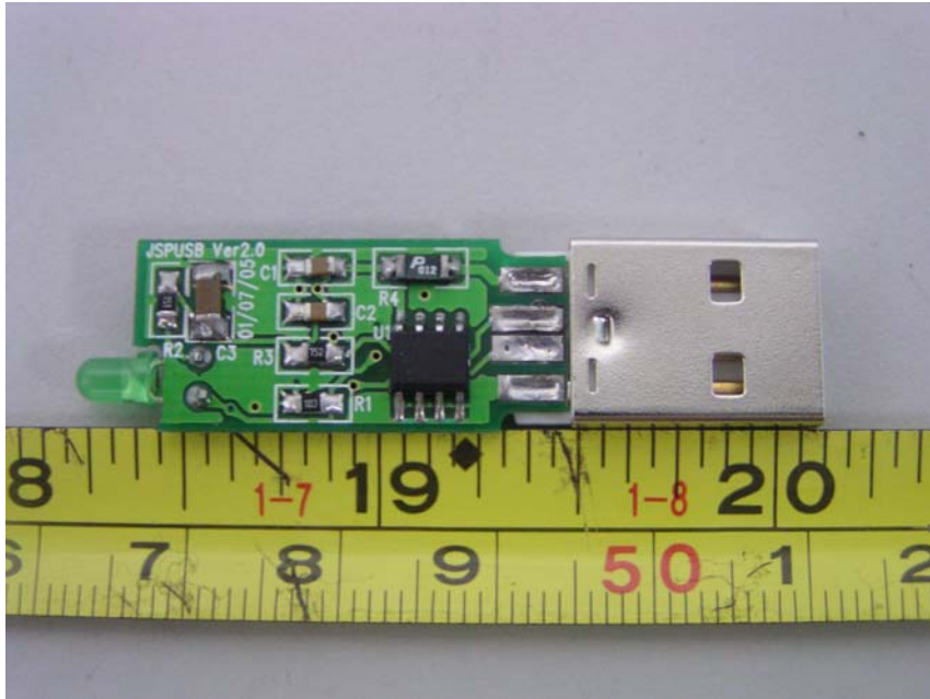
USB Key 1K-PCB View
