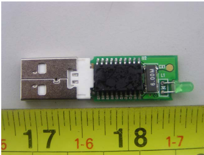
USB Key 8K-PCB View
