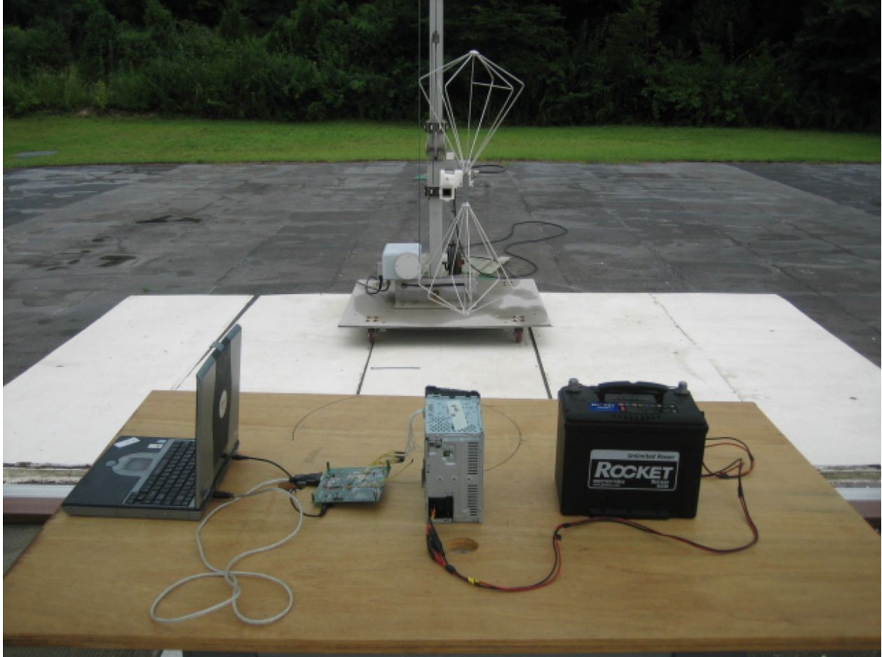
( Open Site Test Setup 1)
