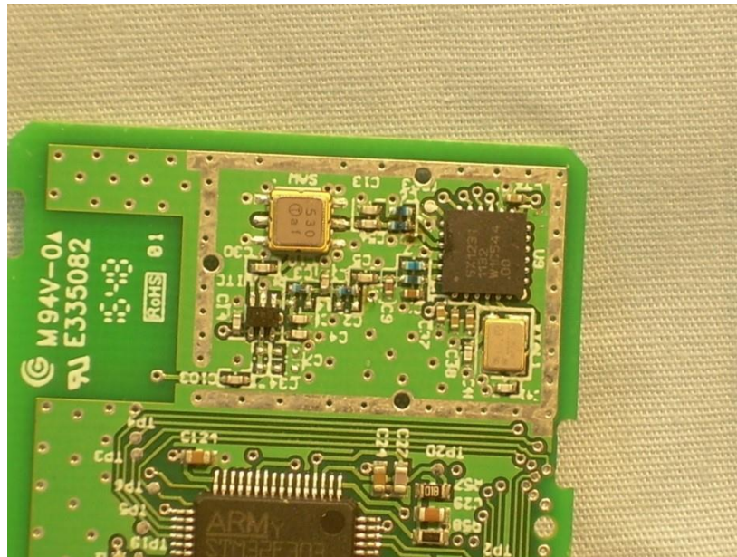
Photograph 3 – View of Circuitry Under RF Shield
