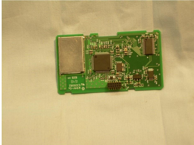
Photograph 1 – View of Component Side of the PCB
