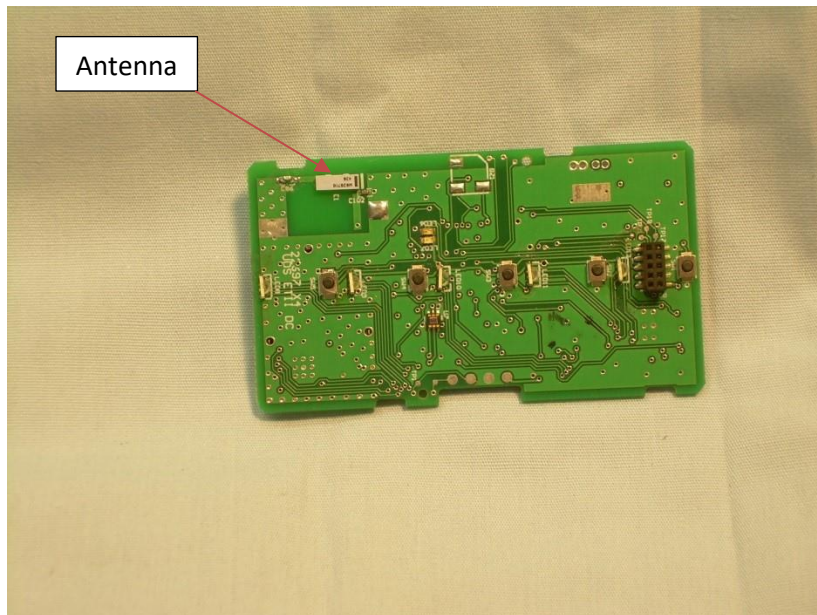
Photograph 2 – View of Trace Side of the PCB
