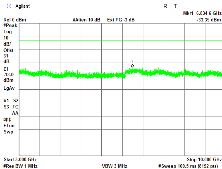
Plot 7.4.18 Spurious emission measurements in 3000 - 10000 MHz at high carrier frequency
