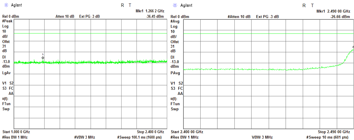
Plot 7.4.10 Spurious emission measurements in 1000 - 2490 MHz range at low carrier frequency
