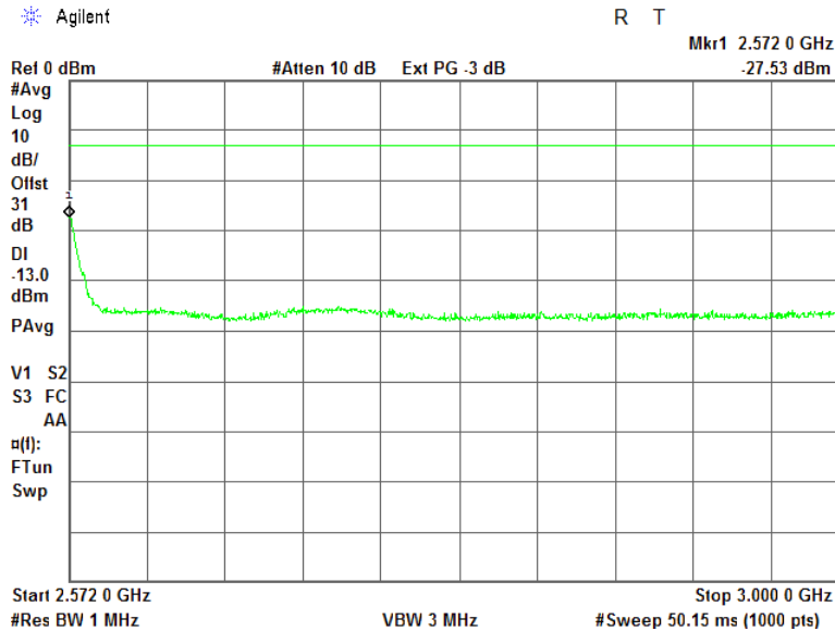
Plot 7.4.15 Spurious emission measurements in 2572 - 3000 MHz at high carrier frequency
