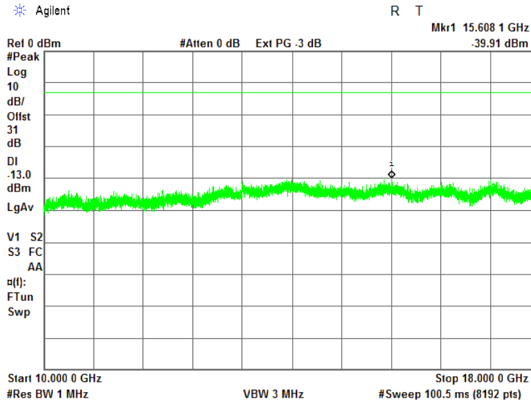
Plot 7.4.21 Spurious emission measurements in 10000 - 18000 MHz at high carrier frequency
