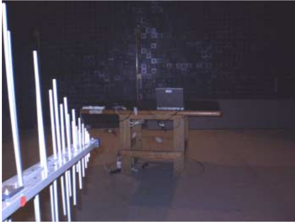
Photograph No.4 Radiated emissions measurement setup in the anechoic chamber in 30 -1000 MHz
