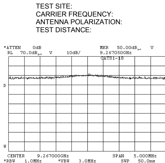
Plot 7.4.21 Radiated emission measurements at the 4 th harmonic
