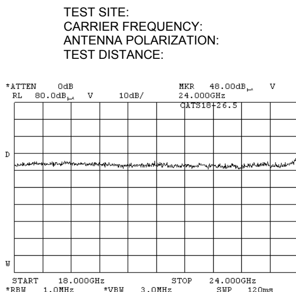
Plot 7.4.18 Radiated emission measurements in 18000 – 24000 MHz range
