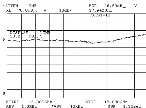
Plot 7.4.16 Radiated emission measurements in 13000 – 18000 MHz range
