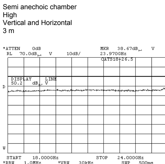
Plot 7.4.18 Radiated emission measurements in 18000 – 24000 MHz range
