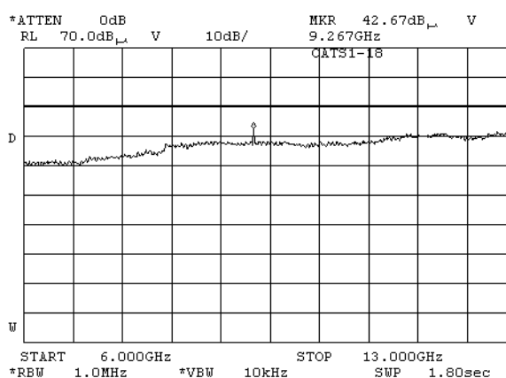
Plot 7.4.14 Radiated emission measurements in 6000 – 13000 MHz range
