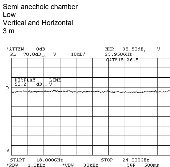
Plot 7.4.17 Radiated emission measurements in 18000 – 24000 MHz range
