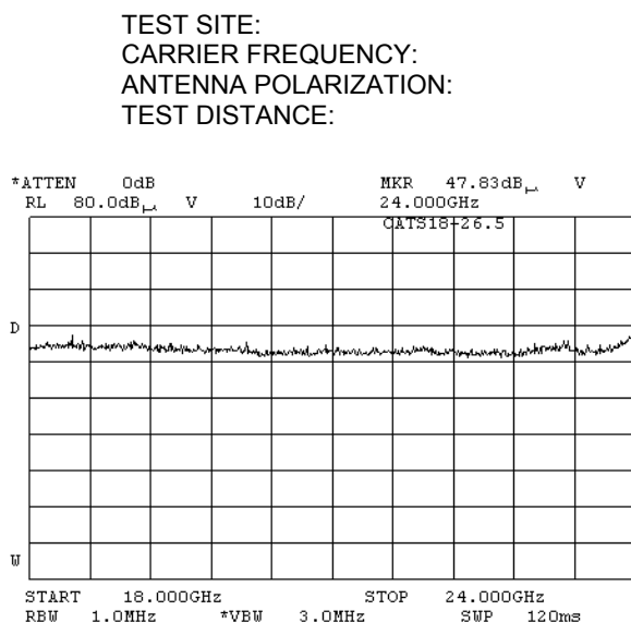
Plot 7.4.17 Radiated emission measurements in 18000 – 24000 MHz range
