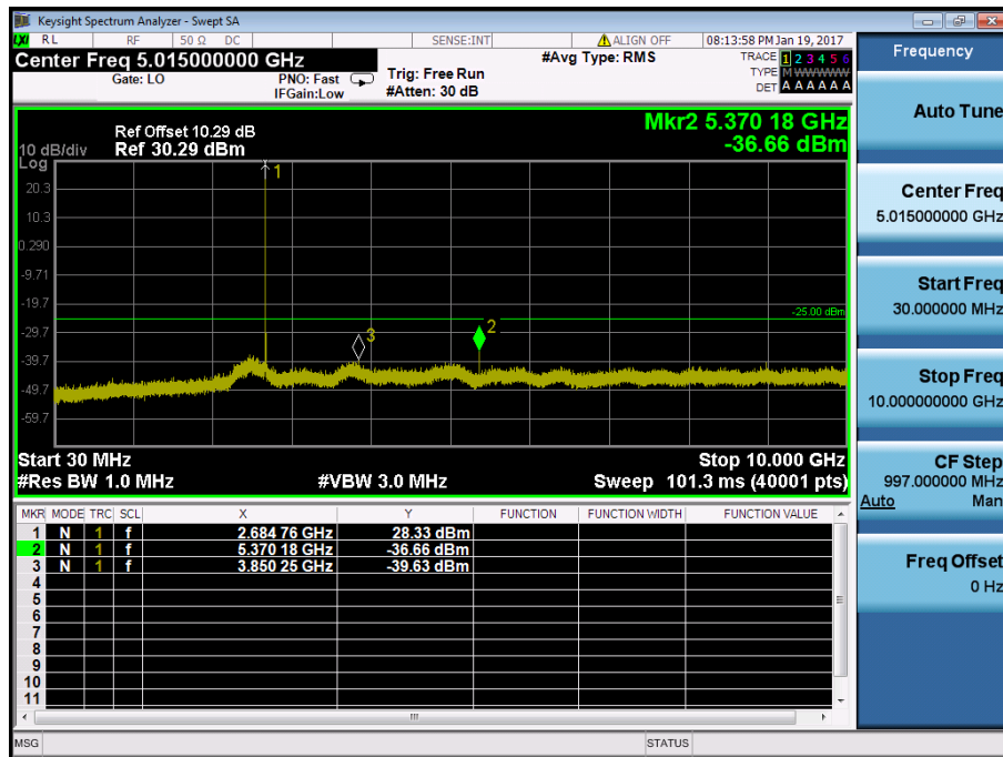
LTE Band 41 / 10MHz / 16QAM - RB Size/Offset (1/25) – High Channel
