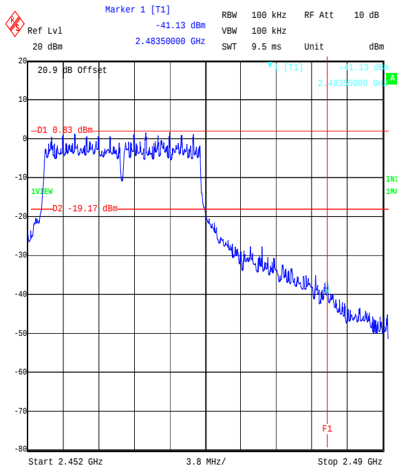
Title: EZURIO 2.4 GHz WLAN Module. FCC Part 15.247 Cond. BandEdge Comment A: 48271JD05 Top Channel OFDM 64QAM Date: 8.SEP.2006 16:40:36
