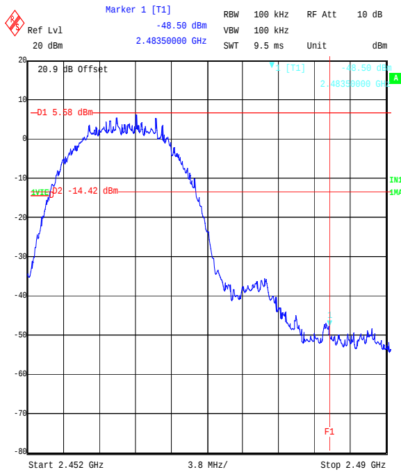
Title: EZURIO 2.4 GHz WLAN Module. FCC Part 15.247 Cond. BandEdge Comment A: 48271JD05 Top Channel DSSS CCK Date: 8.SEP.2006 16:31:00
