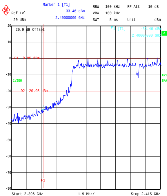
Title: Ezurio 2.4 GHz WLAN module. FCC P15.247 Cond. BandEdge Comment A: 48271JD05 Bottom Channel, BPSK OFDM. Date: 5.SEP.2006 16:53:19
