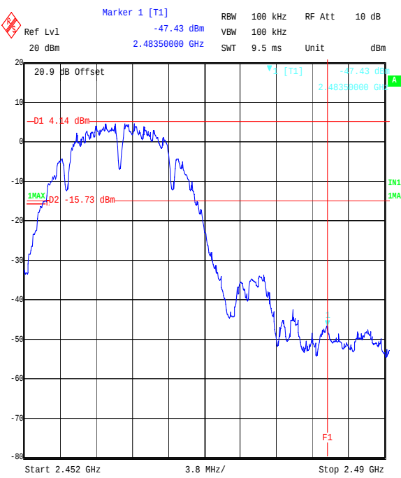
Title: EZURIO 2.4 GHz WLAN Module, FCC Part 15.247 Cond. BandEdge Comment A: 48271JD05 Top Channel DSSS BPSK Date: 8.SEP.2006 16:27:16
