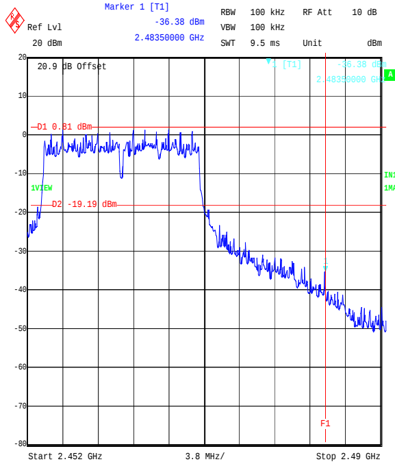
Title: EZURIO 2.4 GHz WLAN Module, FCC Part 15.247 Cond. BandEdge Comment A: 48271JD05 Top Channel OFDM 16QAM Date: 8.SEP.2006 16:38:47
