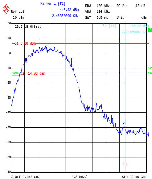
Title: EZURIO 2.4 GHz WLAN Module. FCC Part 15.247 Cond. BandEdge Comment A: 48271JD05 Top Channel DSSS QPSK Date: 8.SEP.2006 16:29:35
