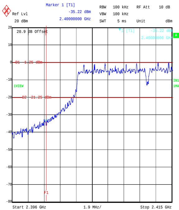
Title: Ezurio 2.4 GHz WLAN module. FCC P15.247 Cond. BandEdge Comment A: 48271JD05 Bottom Channel, QPSK OFDM. Date: 5.SEP.2006 16:54:07
