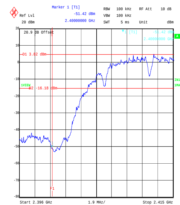
Title: Ezurio 2.4 GHz WLAN module, FCC P15.247 Cond. BandEdge Comment A: 48271JD05 Bottom Channel, BPSK DSSS. Date: 5.SEP.2006 16:47:58
