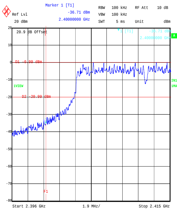
Title: Ezurio 2.4 GHz WLAN module. FCC P15.247 Cond. BandEdge Comment A: 48271JD05 Bottom Channel, 64QAM OFDM. Date: 5.SEP.2006 16:56:05
