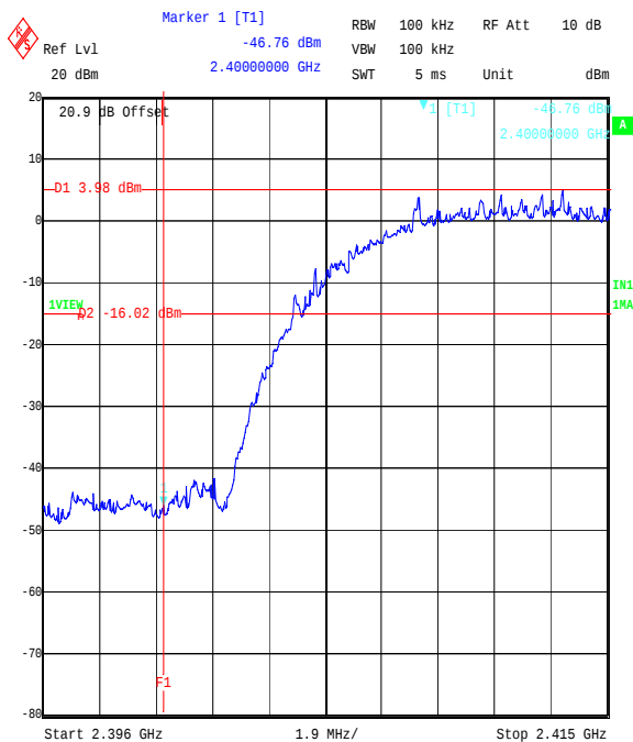
Title: Ezurio 2.4 GHz WLAN module. FCC P15.247 Cond. BandEdge Comment A: 48271JD05 Bottom Channel, CCK DSSS. Date: 5.SEP.2006 16:50:10
