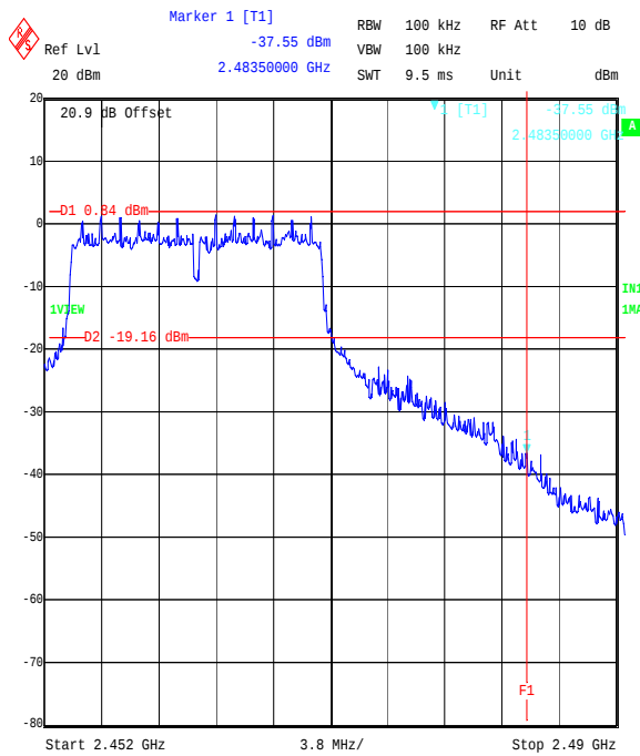
Title: EZURIO 2.4 GHz WLAN Module. FCC Part 15.247 Cond. BandEdge Comment A: 48271JD05 Top Channel OFDM BPSK Date: 8.SEP.2006 16:32:35
