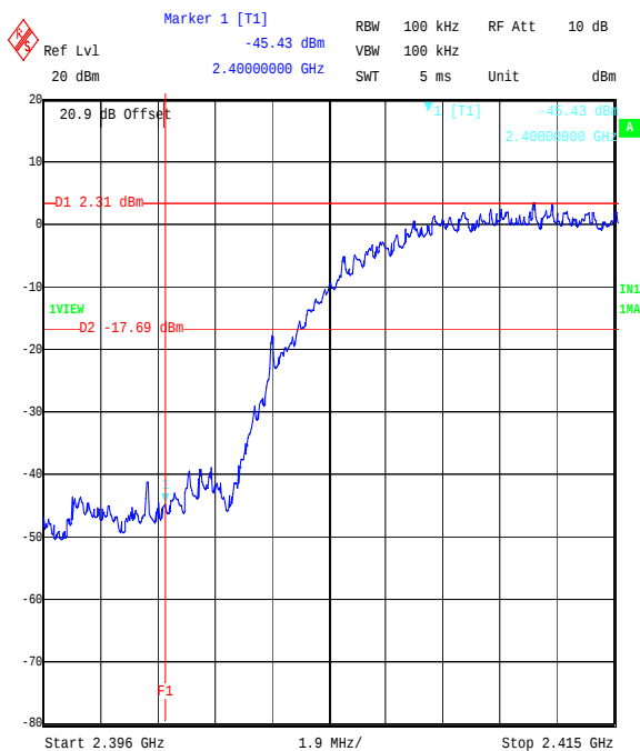
Title: Ezurio 2.4 GHz WLAN module. FCC P15.247 Cond. BandEdge Comment A: 48271JD05 Bottom Channel, QPSK DSSS. Date: 5.SEP.2006 16:49:00
