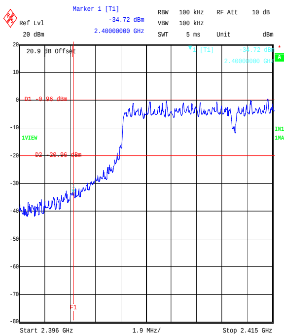
Title: Ezurio 2.4 GHz WLAN module, FCC P15.247 Cond. BandEdge Comment A: 48271JD05 Bottom Channel, 16QAM OFDM. Date: 5.SEP.2006 16:55:08
