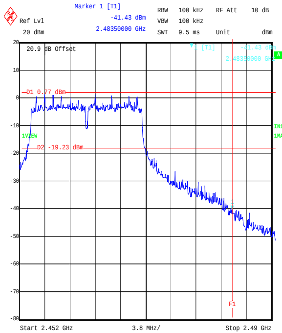
Title: EZURIO 2.4 GHz WLAN Module. FCC Part 15.247 Cond. BandEdge Comment A: 48271JD05 Top Channel OFDM QPSK Date: 8.SEP.2006 16:37:35
