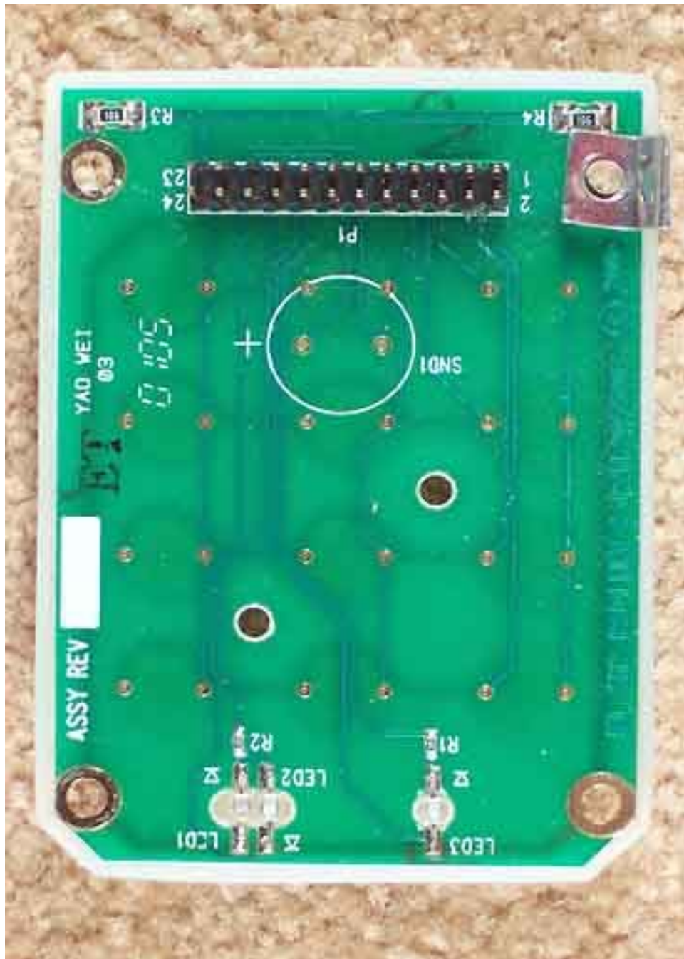
Keypad PCB Back
