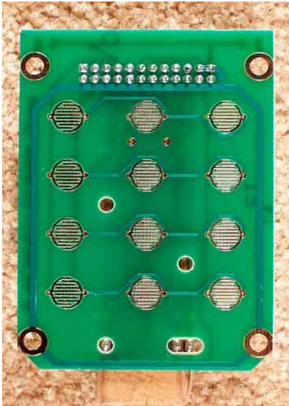
Keypad PCB Front
