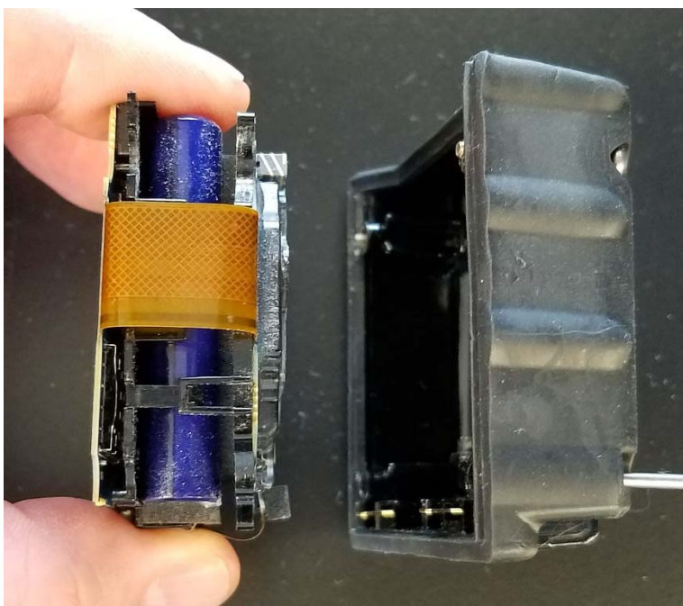
Wi-fi battery pack disassembly
