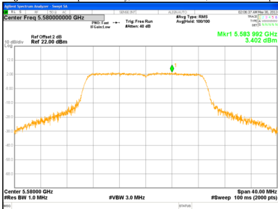
Figure 132: Power Spectral Density, 5580 MHz at 802.11n, Chain 3 – 6.5 Mbps
