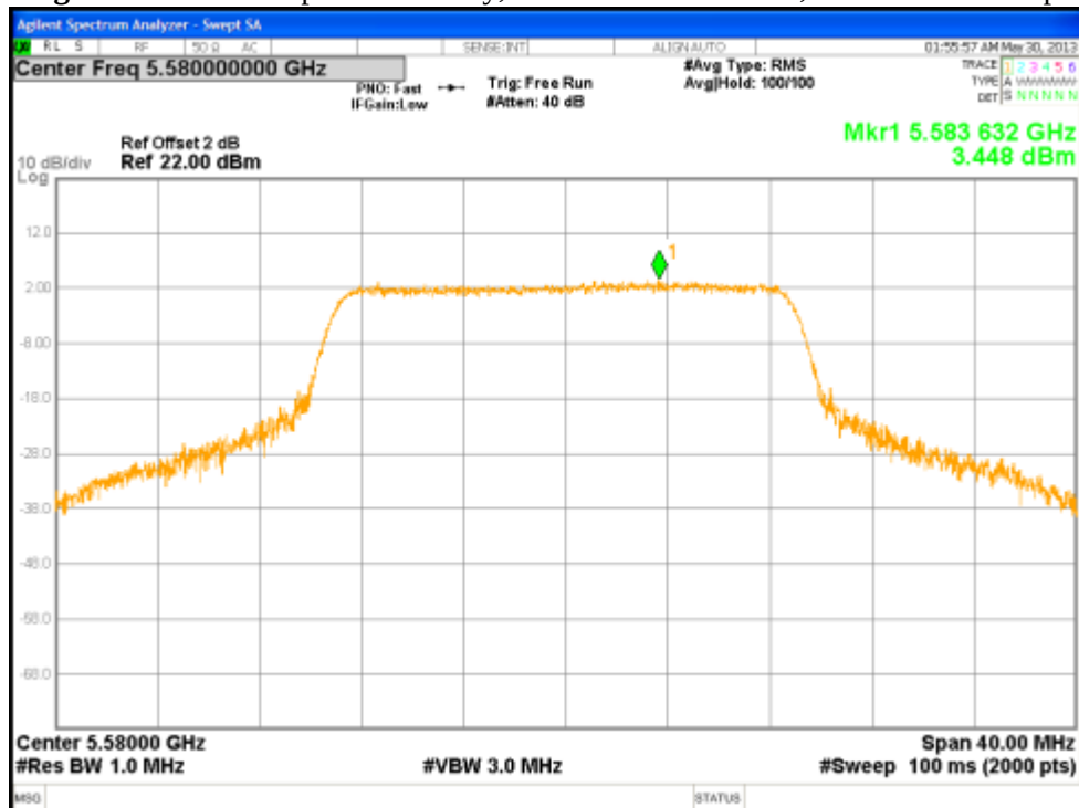
Figure 130: Power Spectral Density, 5580 MHz at 802.11n, Chain 1 – 6.5 Mbps
