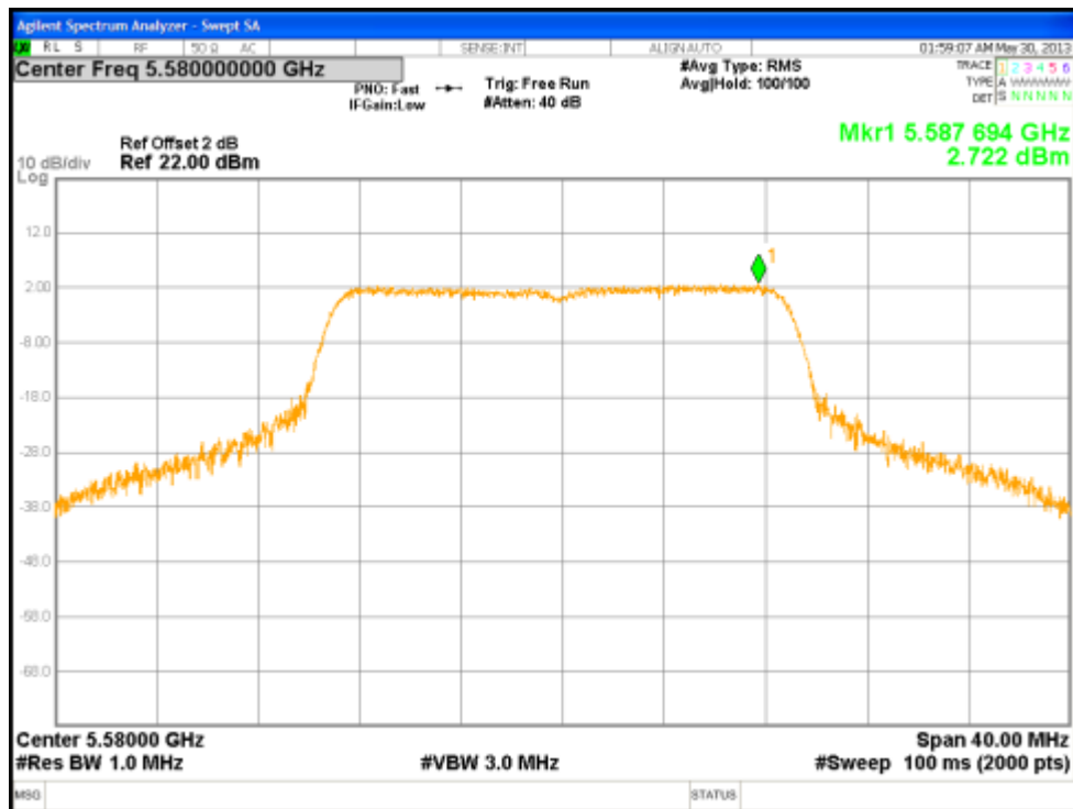
Figure 131: Power Spectral Density, 5580 MHz at 802.11n, Chain 2 – 6.5 Mbps
