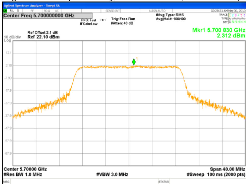
Figure 137: Power Spectral Density, 5700 MHz at 802.11n, Chain 3 – 6.5 Mbps
