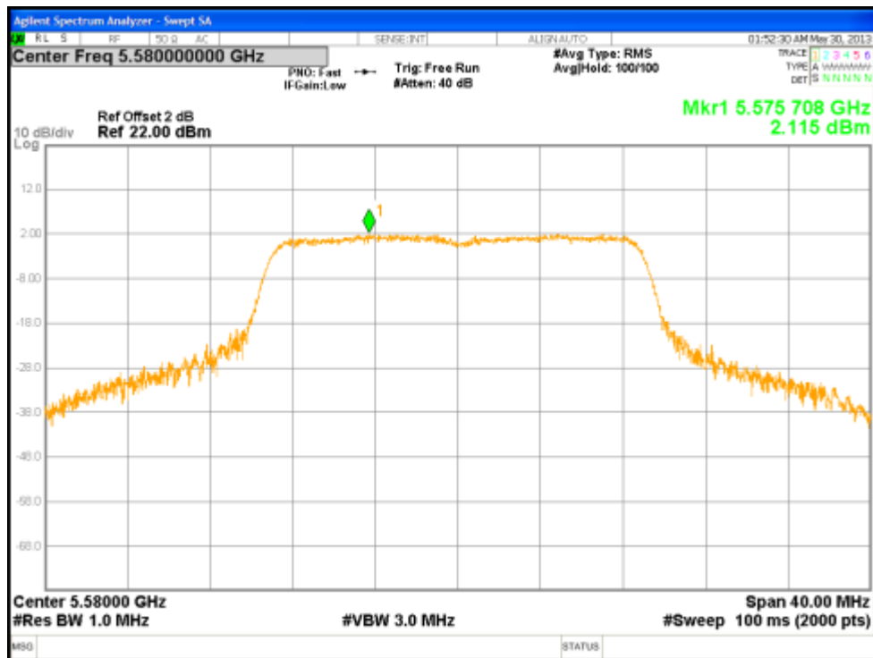
Figure 129: Power Spectral Density, 5580 MHz at 802.11n, Chain 0 – 6.5 Mbps
