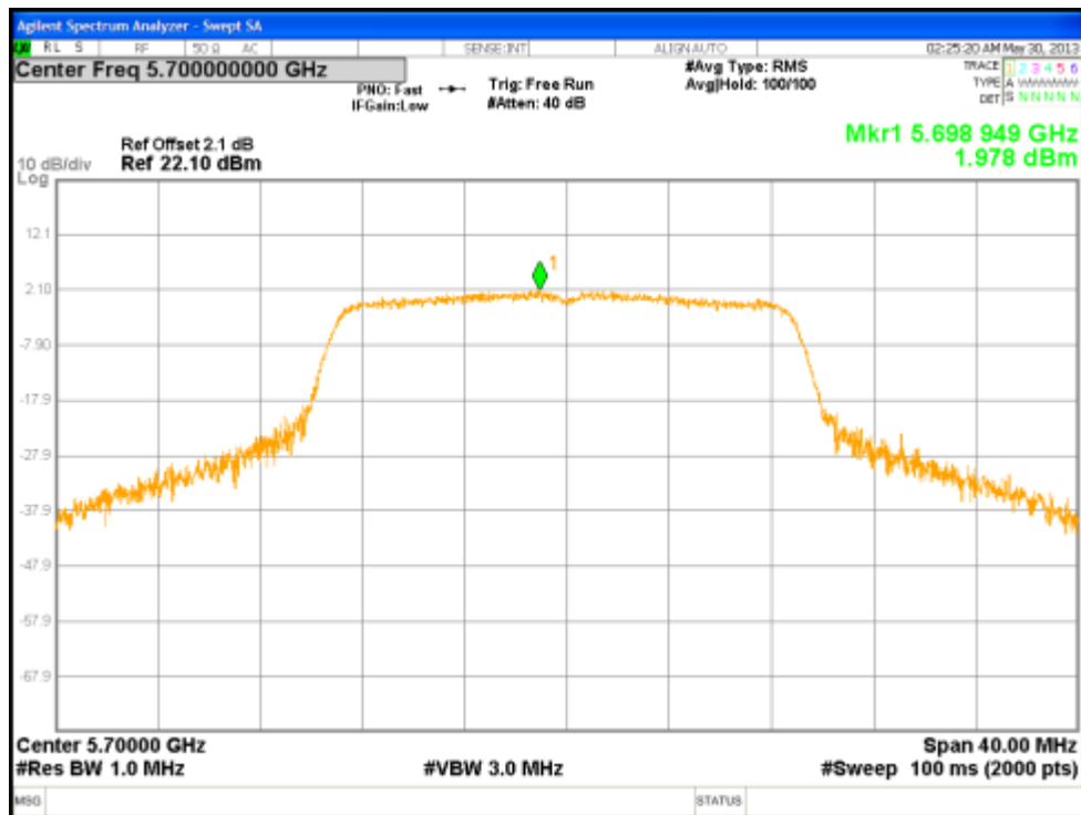
Figure 136: Power Spectral Density, 5700 MHz at 802.11n, Chain 2 – 6.5 Mbps
