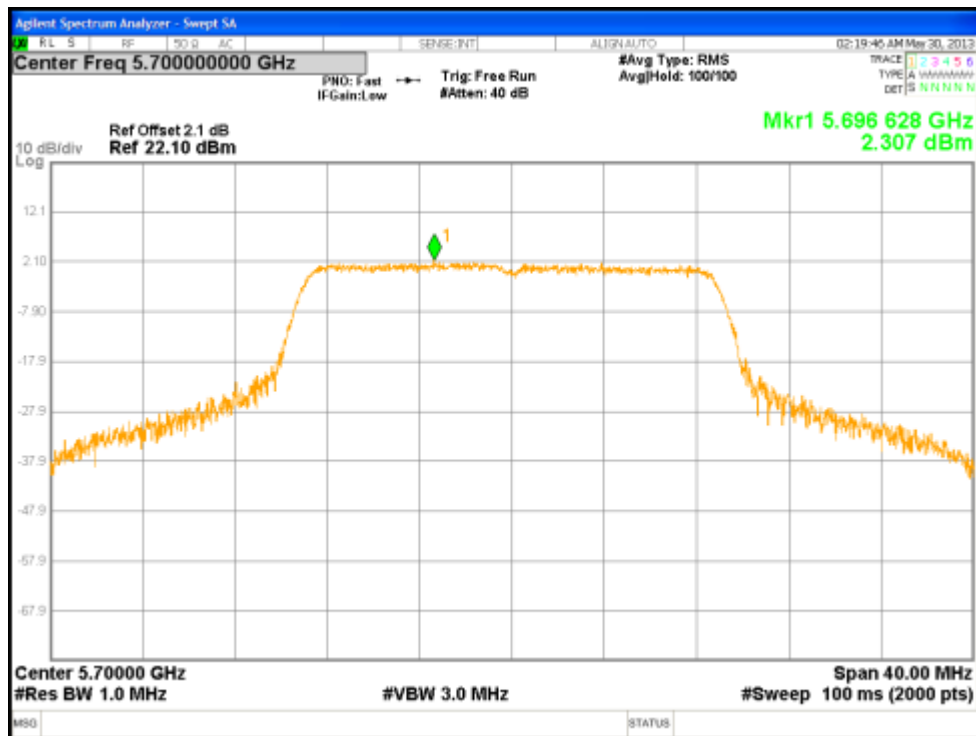
Figure 134: Power Spectral Density, 5700 MHz at 802.11n, Chain 0 – 6.5 Mbps
