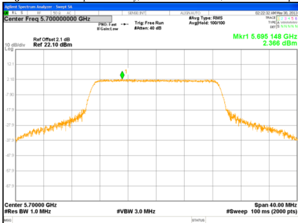
Figure 135: Power Spectral Density, 5700 MHz at 802.11n, Chain 1 – 6.5 Mbps
