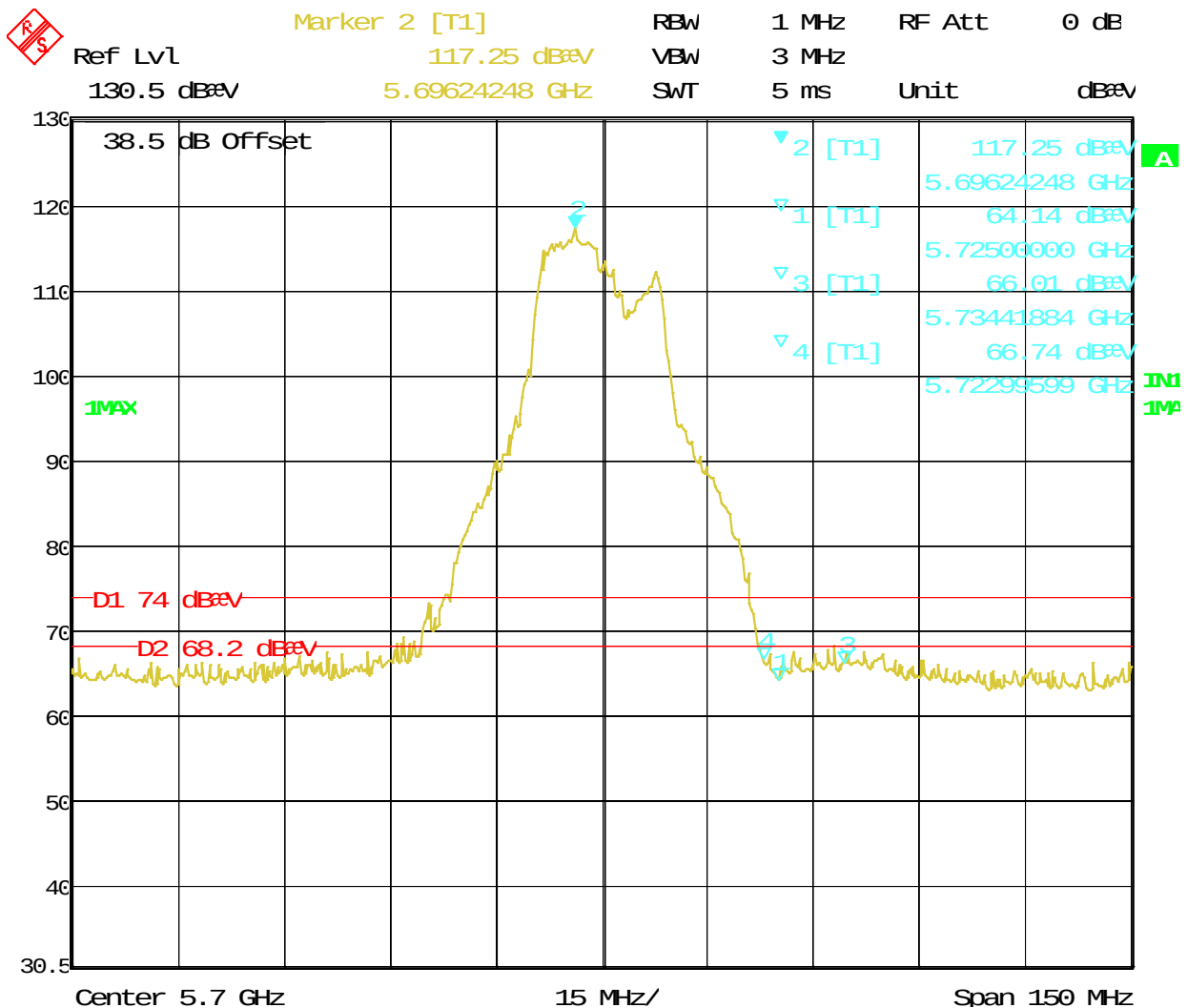
Figure 166: Radiated Emission at the Edge for Channel 5700 MHz at 6.5Mbps – Horiz. (Peak)
