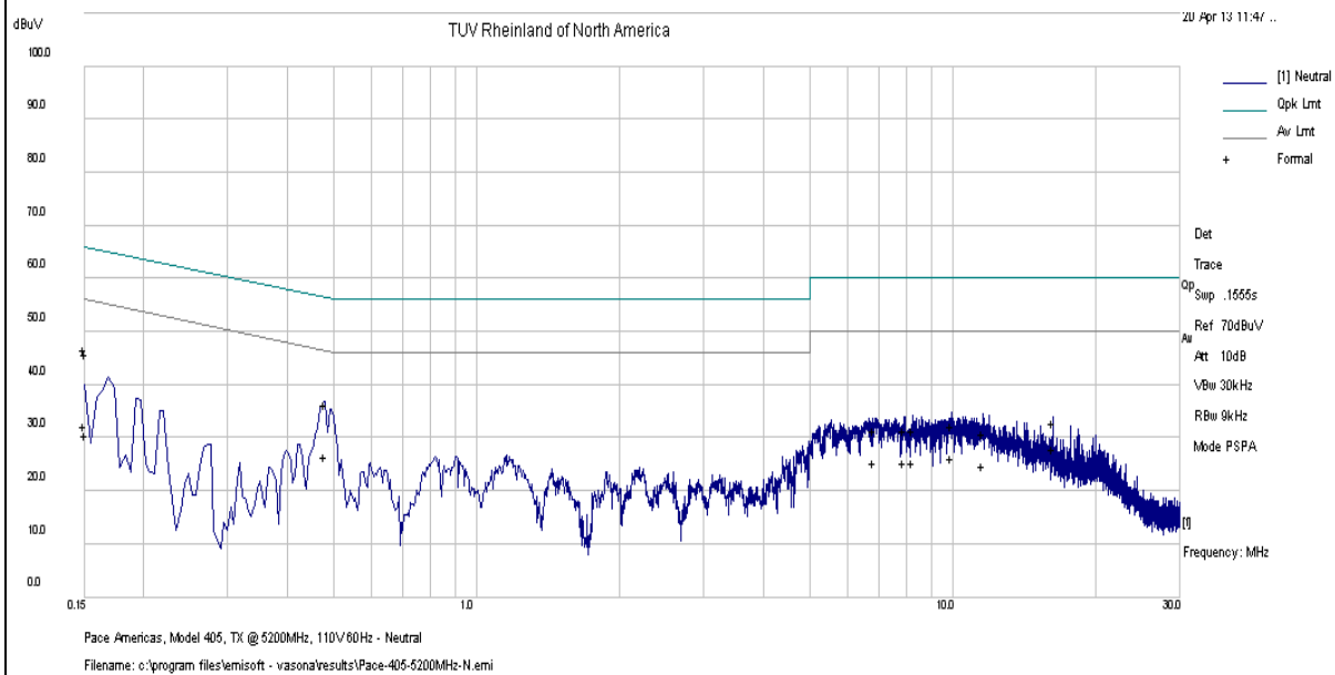
150 kHz to 30 MHz Plot for Line 2 (Neutral)
