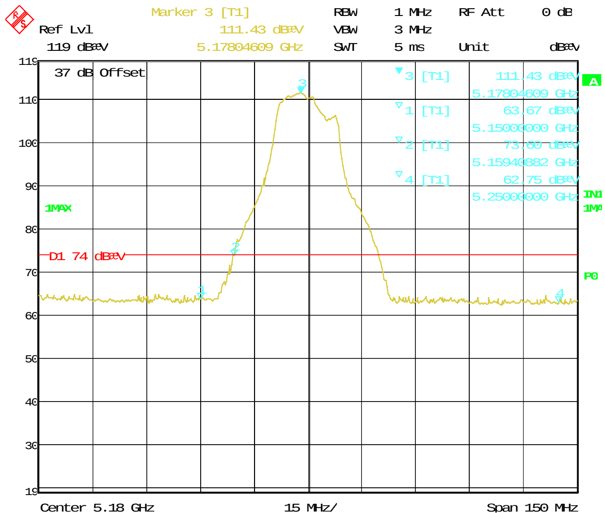
Figure 143: Radiated Emission at the Edge for Channel 5180 MHz at 6.5Mbps – Horiz. (Peak)
