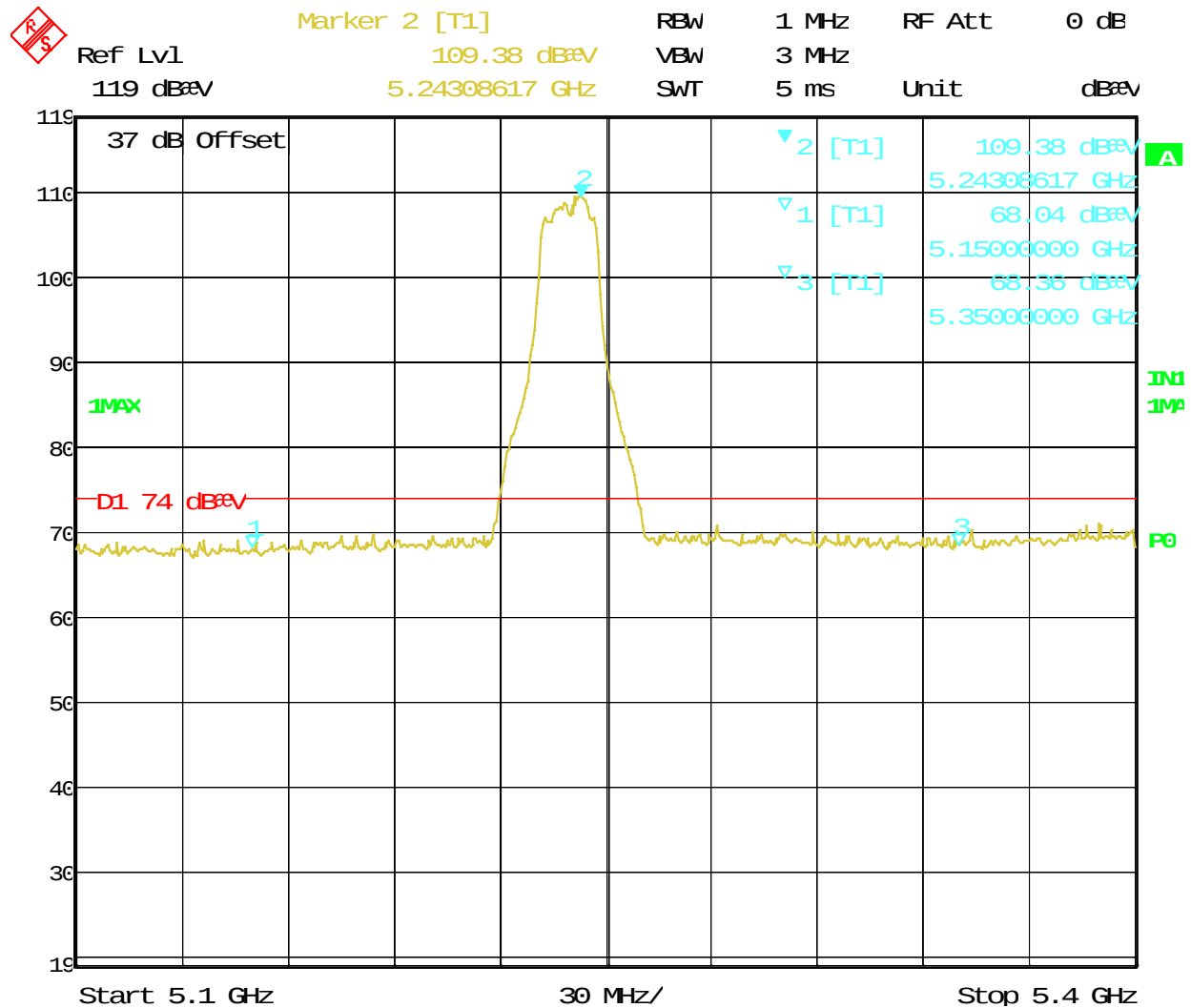
Figure 139: Radiated Emission at the Edge for Channel 5240 MHz at 6 Mbps – Horiz. (Peak)
