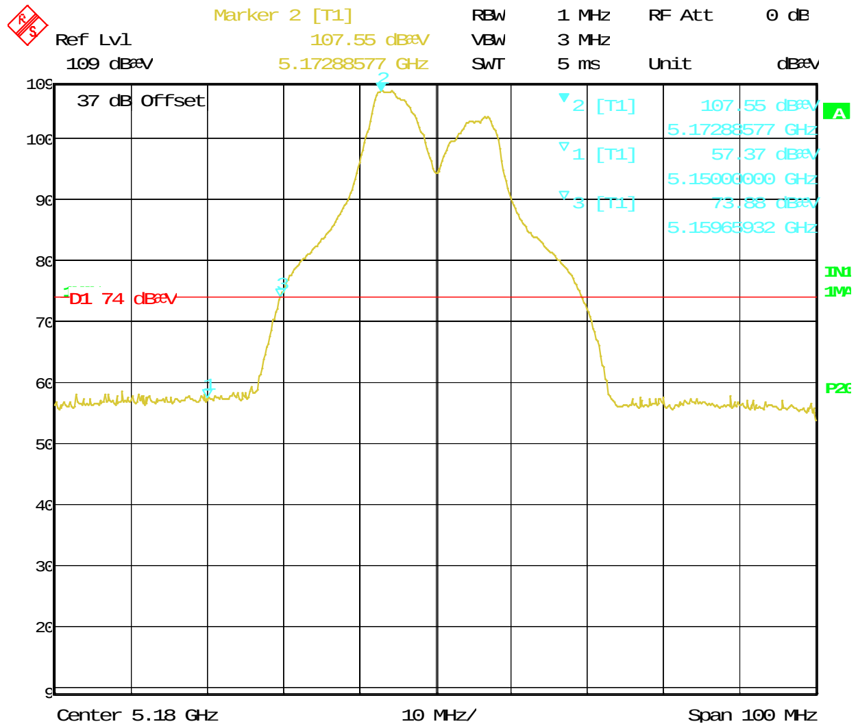
Figure 135: Radiated Emission at the Edge for Channel 5180 MHz at 6 Mbps – Horiz. (Peak)
