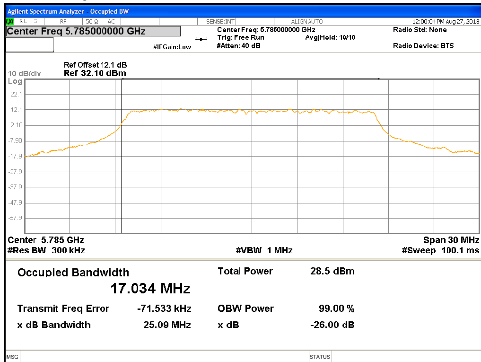
Figure 44: 99% Bandwidth at 5785 MHz, 802.11A, Chain 1
