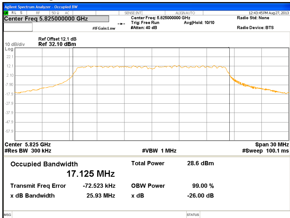
Figure 56: 99% Bandwidth at 5825 MHz, 802.11A, Chain 3
