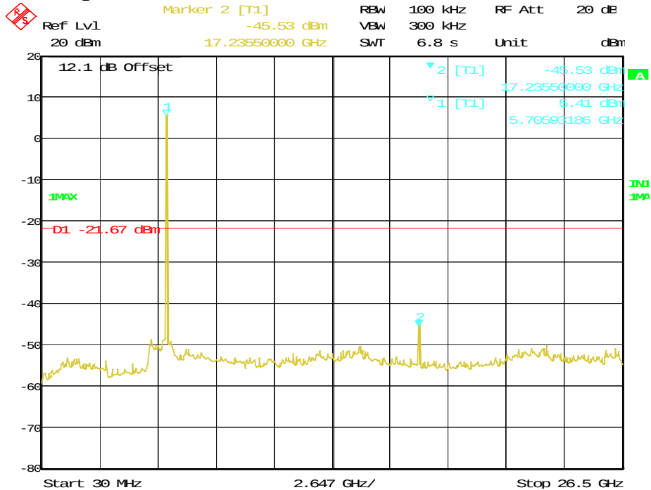
Figure 103: Reference Level for 802.11A at 5745 MHz, Chain 2
