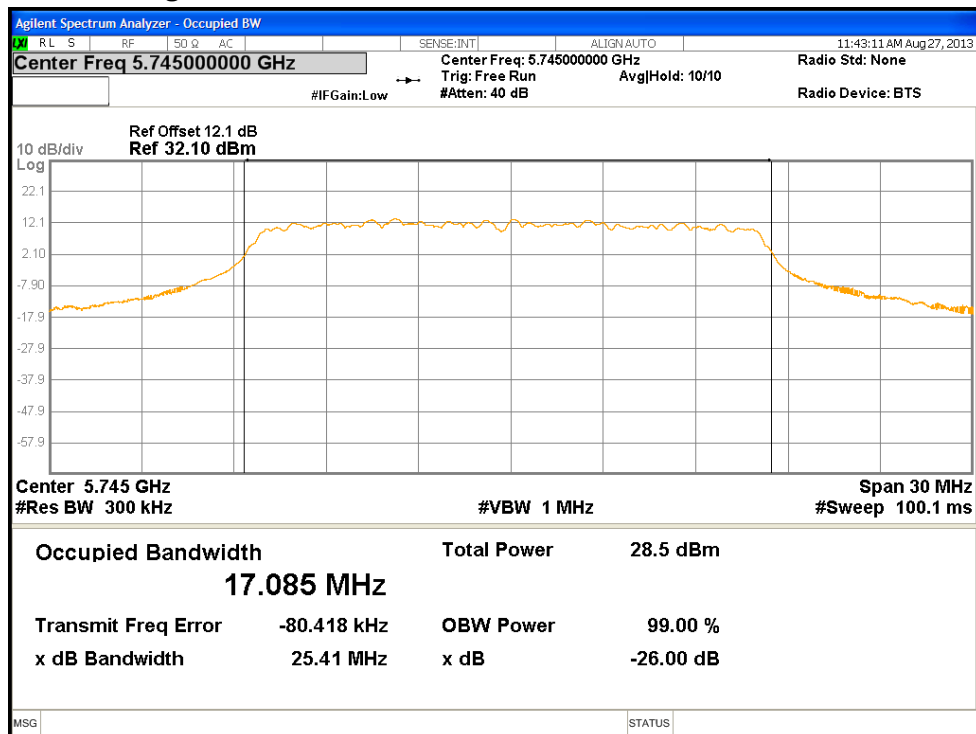
Figure 38: 99% Bandwidth at 5745 MHz, 802.11A, Chain 2
