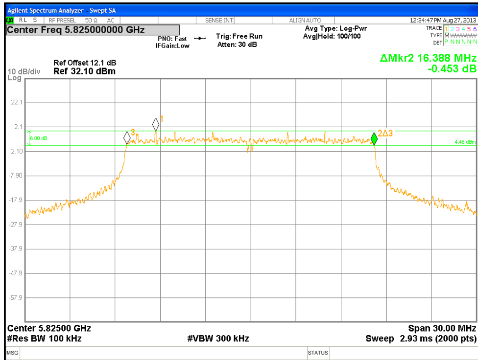
Figure 51: DTS Bandwidth at 5825 MHz, 802.11A, Chain 1
