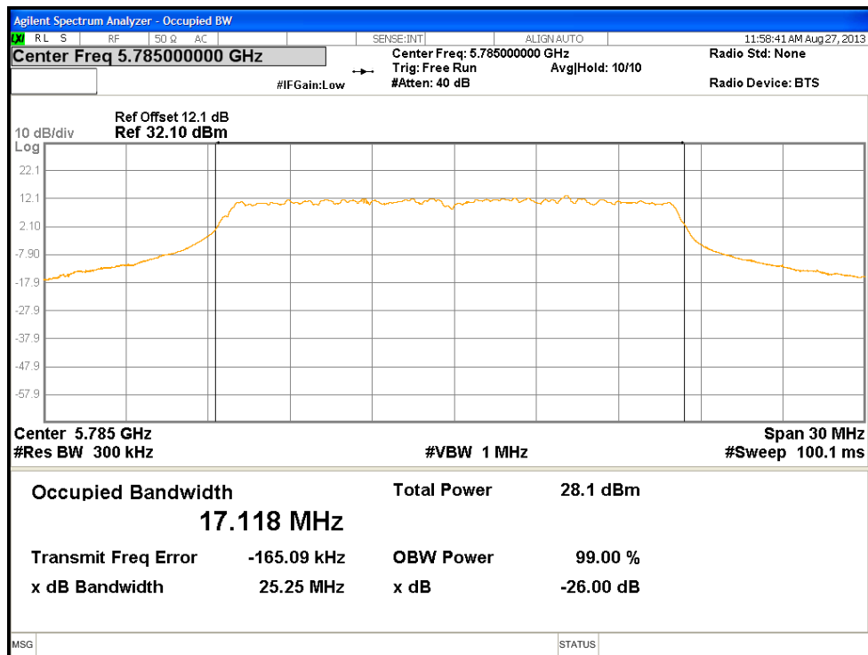
Figure 42: 99% Bandwidth at 5785 MHz, 802.11A, Chain 0
