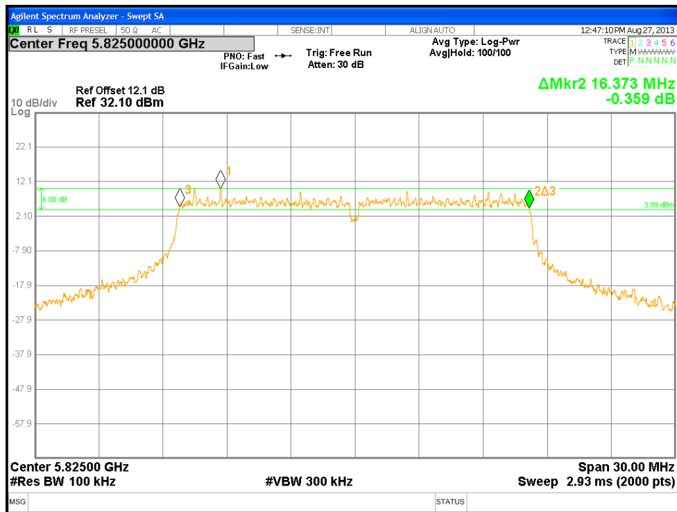
Figure 55: DTS Bandwidth at 5825 MHz, 802.11A, Chain 3
