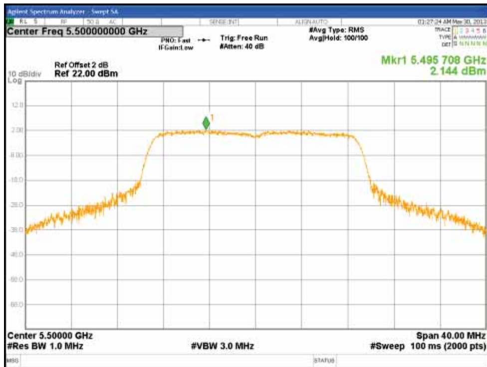
Figure 73: Power Spectral Density, 5500 MHz at 802.11n, Chain 0 – 6.5Mbps
