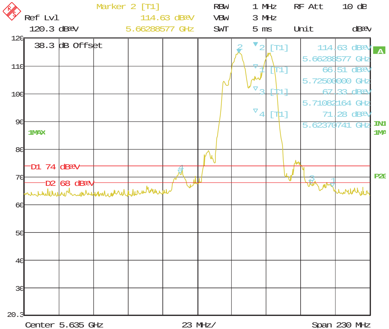
Figure 117: Radiated Emission at the Edge for Channel 5670 MHz at 13.5Mbps – Vert (Peak)
