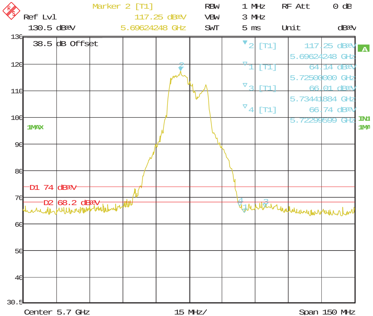
Figure 107: Radiated Emission at the Edge for Channel 5700 MHz at 6.5Mbps – Horiz. (Peak)
