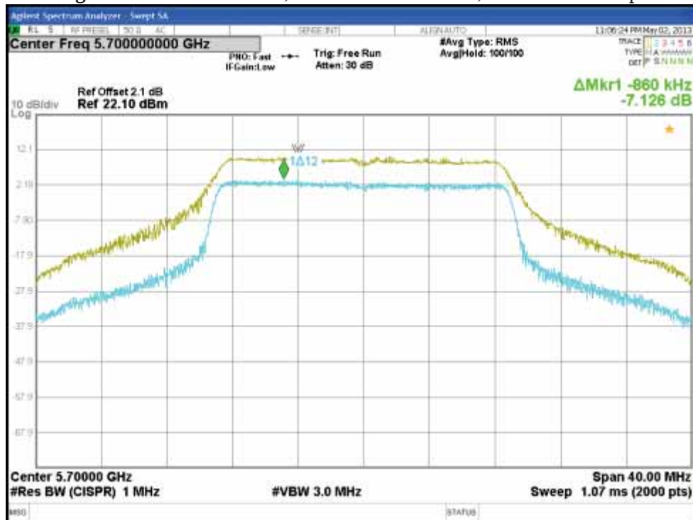
Figure 58: Peak Excursion, 5700 MHz at 802.11n, Chain 1 – 6.5Mbps
