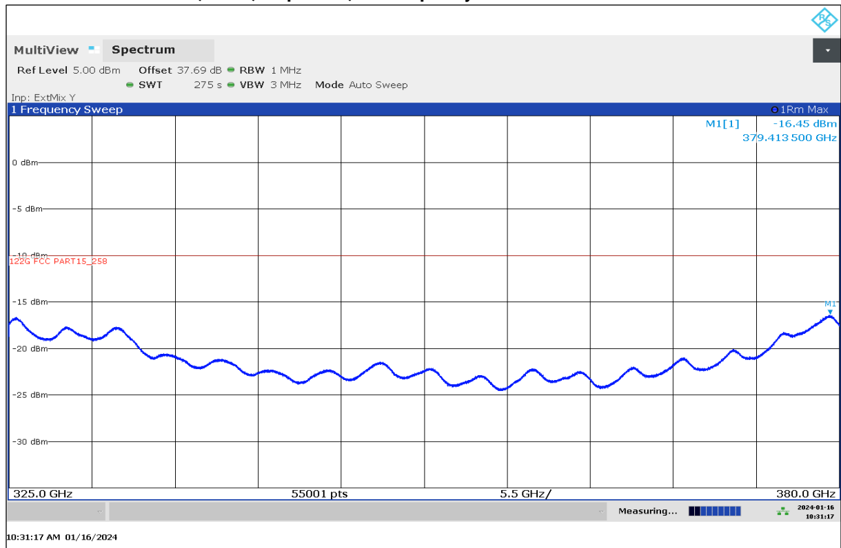
Plot 62: 325 GHz – 380 GHz, EUT8, stop mode, low frequency
