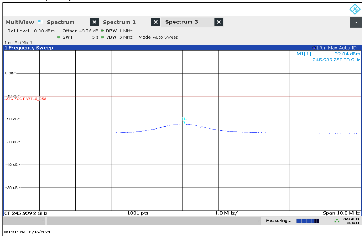
Plot 18: 245 GHz, EUT7, normal mode
