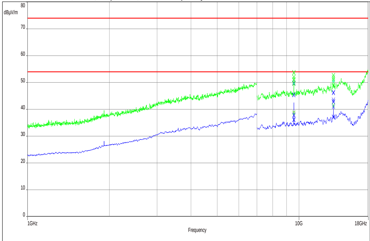
Plot 27: 1GHz – 18 GHz, EUT9, stop mode, middle frequency
