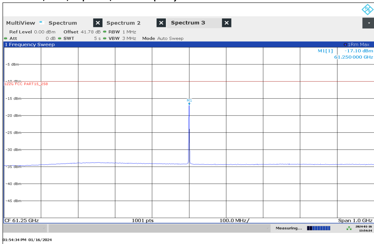
Plot 41: 61 GHz, EUT9, stop mode, middle frequency
