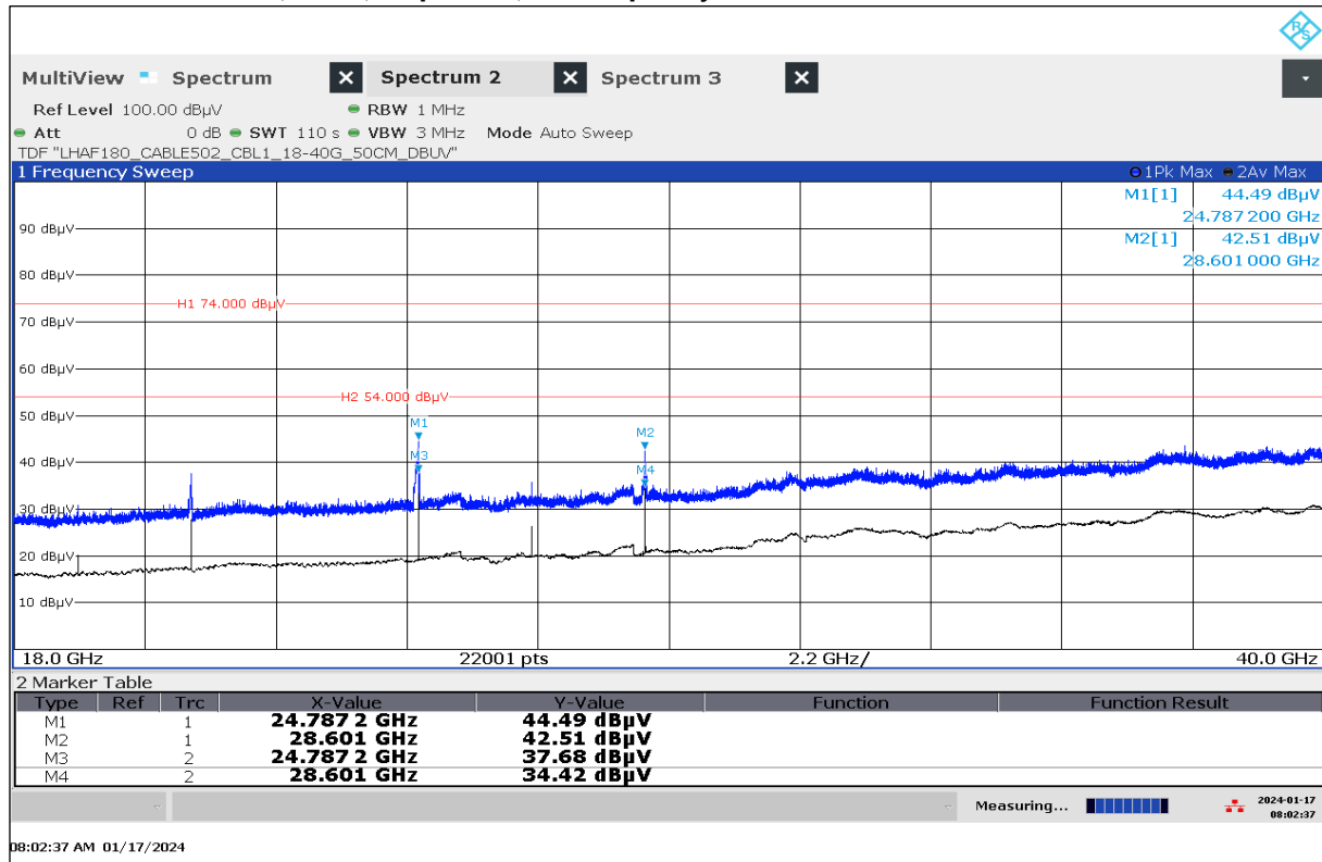
Plot 29: 18 GHz – 40 GHz, EUT8, stop mode, low frequency
