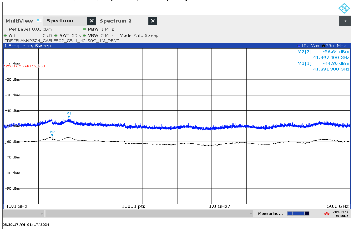
Plot 32: 40 GHz – 50 GHz, EUT8, stop mode, low frequency
