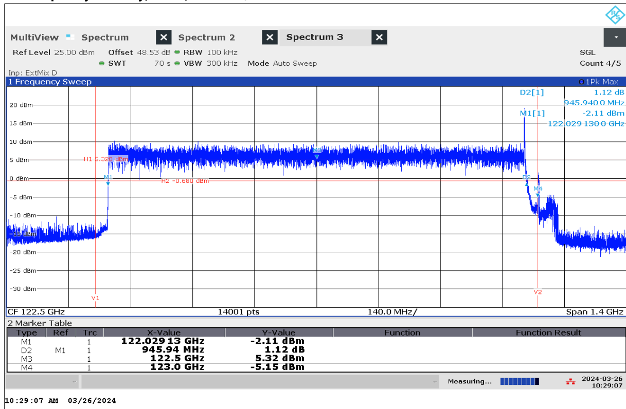
Plot 67: Frequency Stability, EUT7, 0 °C / V_{nom}
