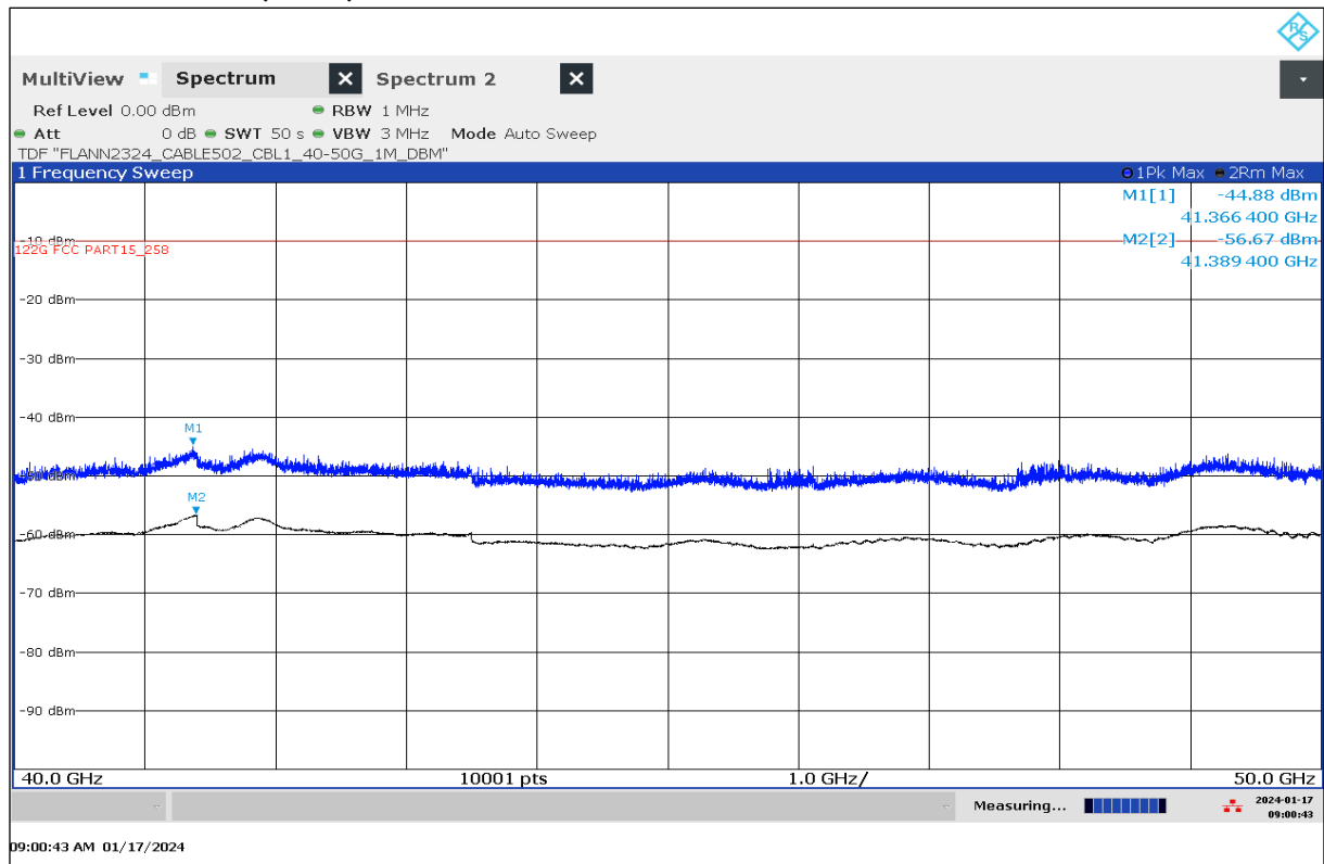
Plot 9: 40 GHz – 50 GHz, EUT7, normal mode
