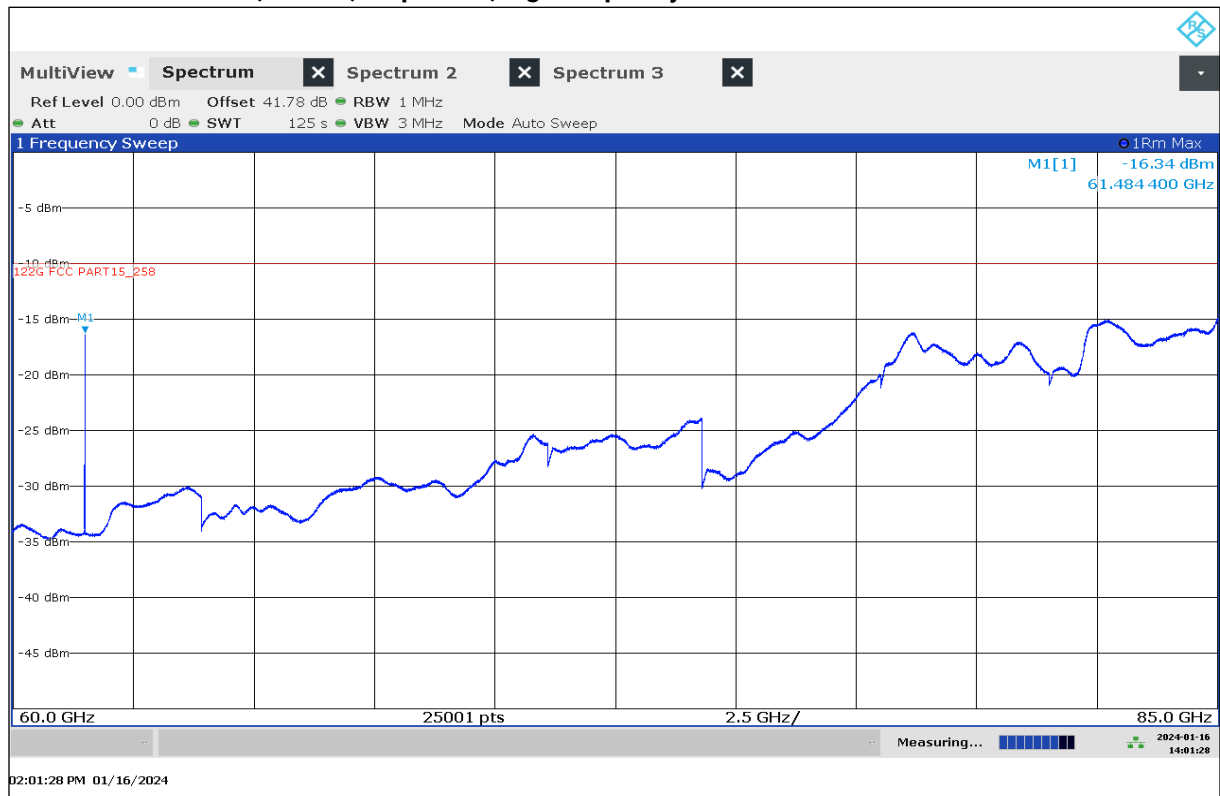
Plot 42: 60 GHz – 85 GHz, EUT10, stop mode, high frequency
