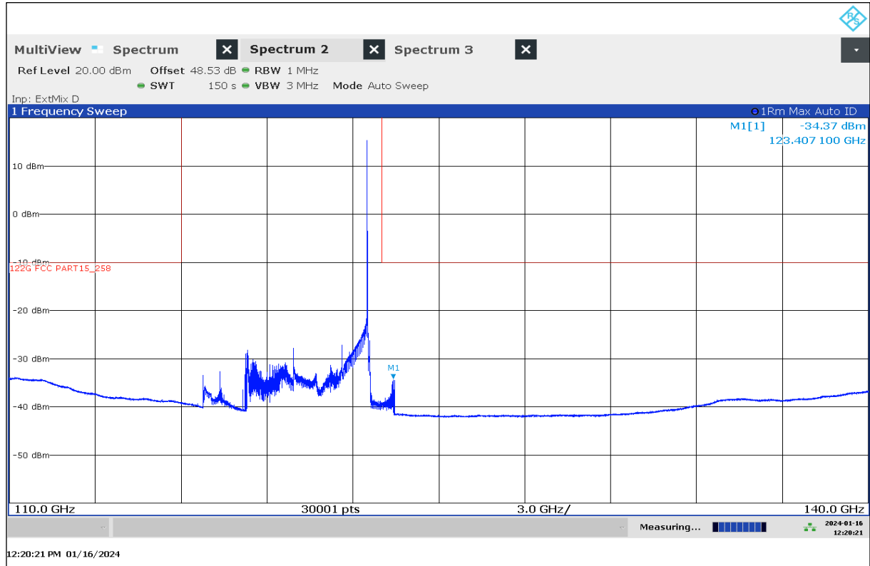
Plot 51: 110 GHz – 140 GHz, EUT9, stop mode, middle frequency
