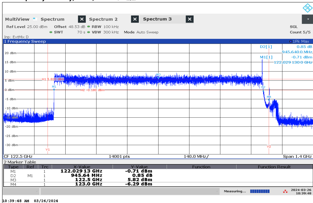
Plot 68: Frequency Stability, EUT7, +10 °C / V_{nom}
