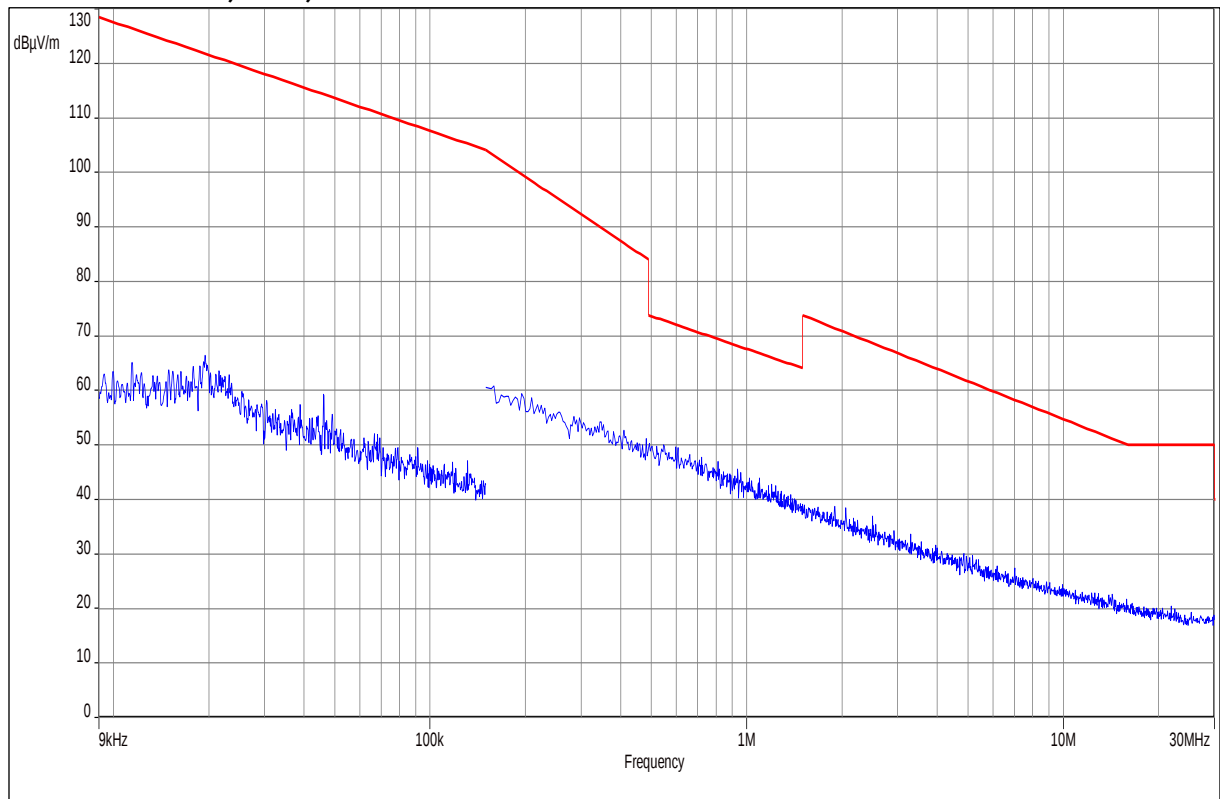
Plot 5: 9 kHz – 30 MHz, EUT7, normal mode
