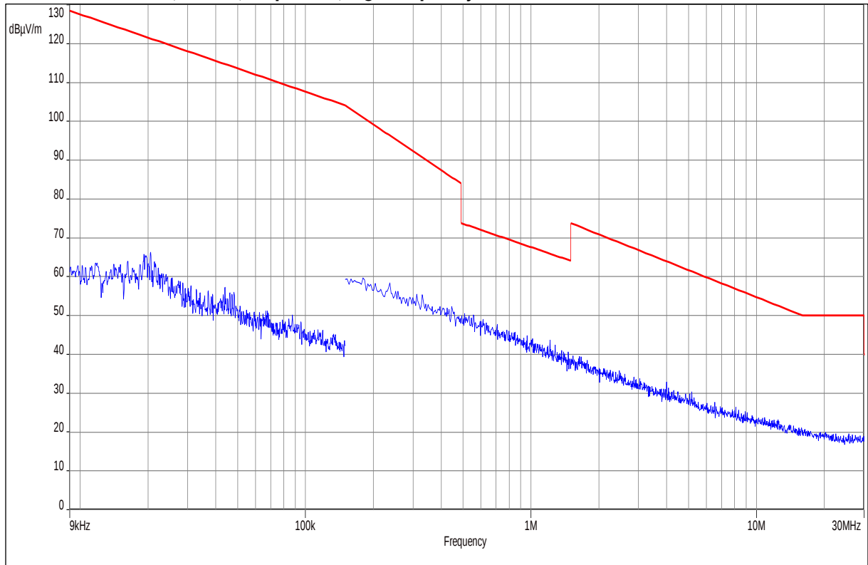
Plot 22: 9 kHz – 30 MHz, EUT10, stop mode, high frequency
