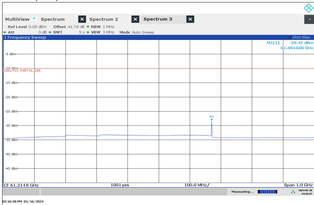
Plot 12: 61 GHz, EUT7, normal mode
