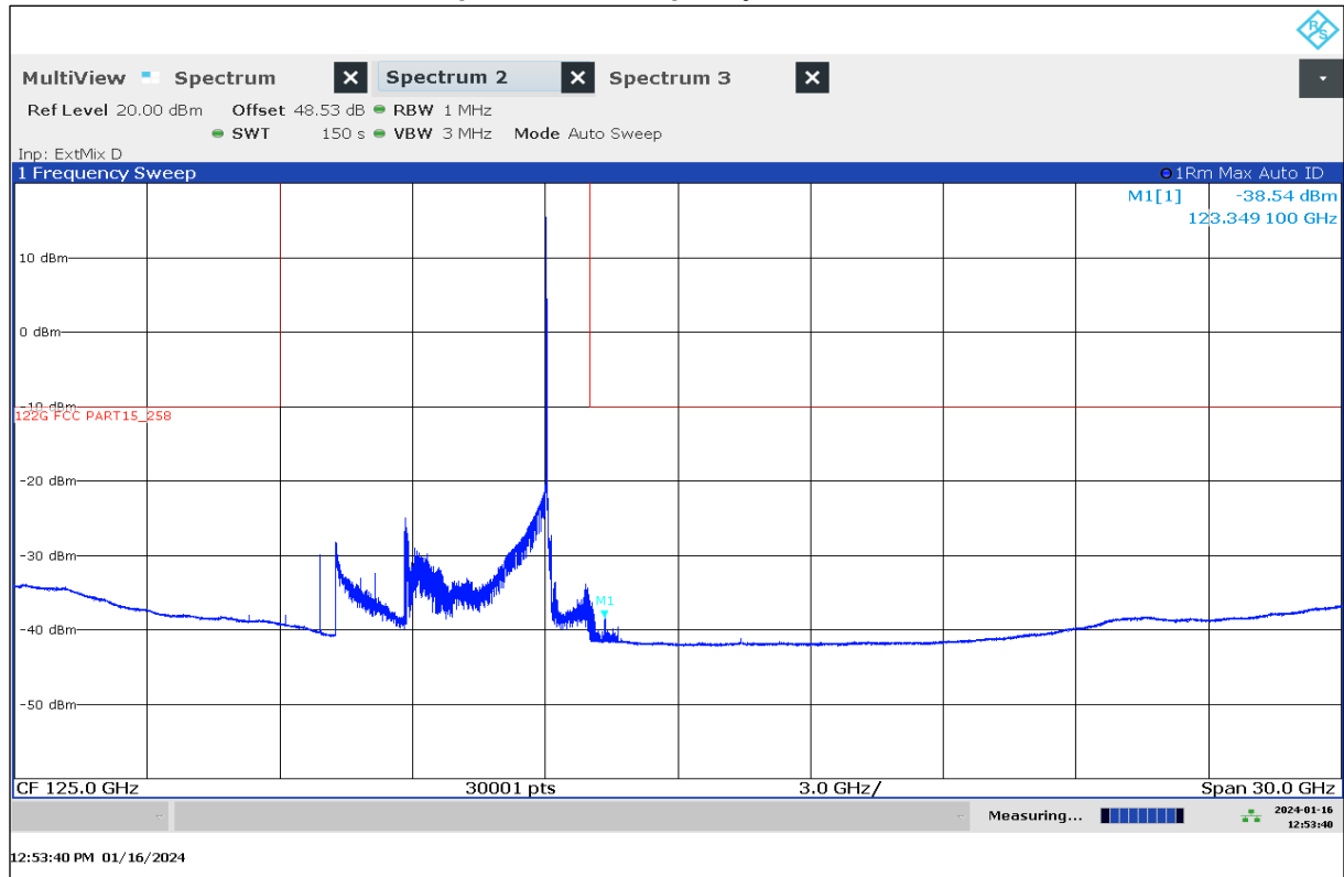
Plot 50: 110 GHz – 140 GHz, EUT8, stop mode, low frequency
