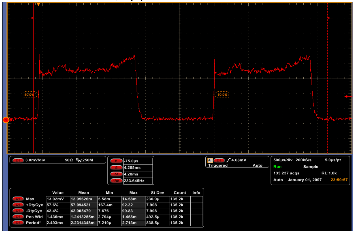
Plot 3: Normal mode, EUT 7 emission, duty cycle
