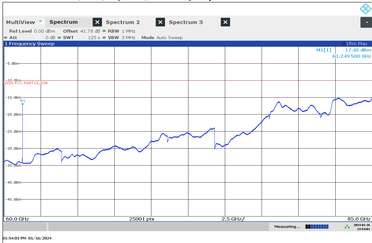
Plot 40: 60 GHz – 85 GHz, EUT9, stop mode, middle frequency
