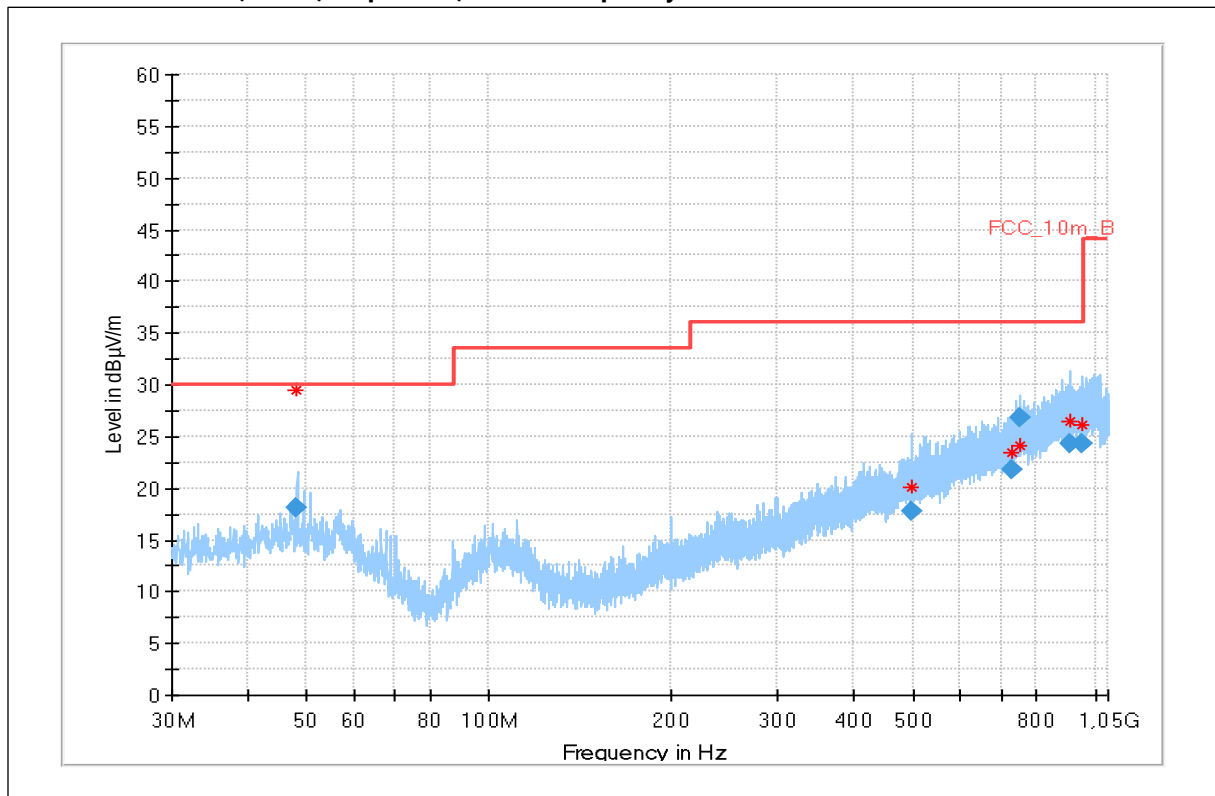
Plot 24: 30 MHz – 1GHz, EUT9, stop mode, middle frequency
