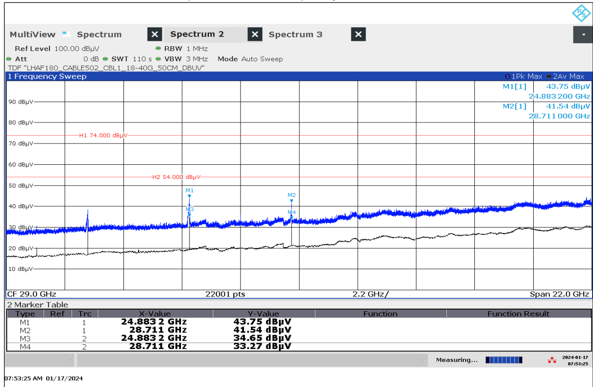
Plot 30: 18 GHz – 40 GHz, EUT9, stop mode, middle frequency
