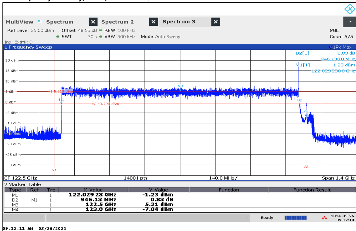
Plot 70: Frequency Stability, EUT7, +20 °C / V_{\text{nom}}
