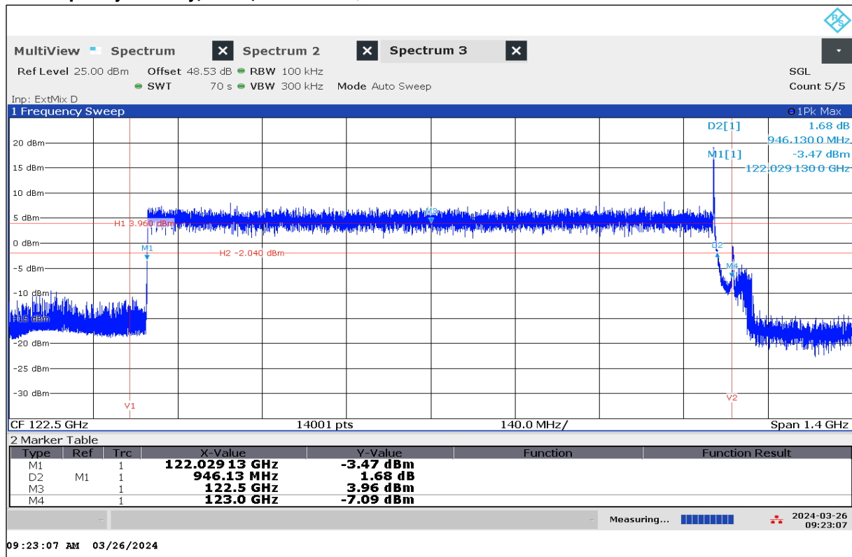
Plot 71: Frequency Stability, EUT7, +20 °C / V_{\max}
