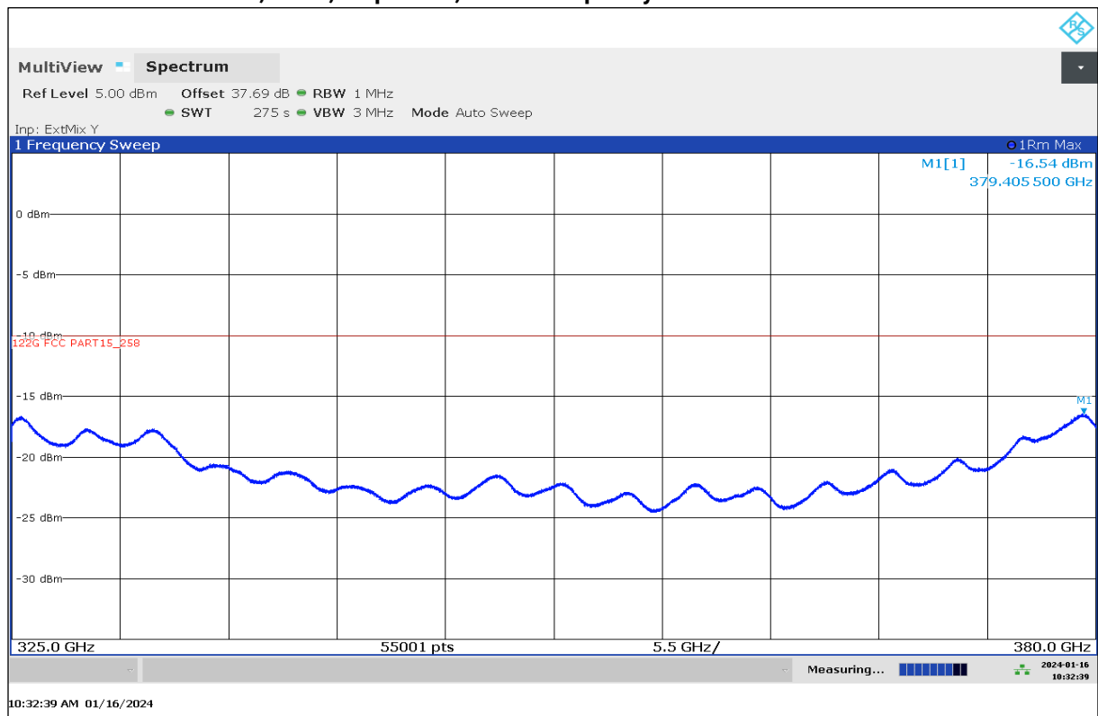
Plot 63: 325 GHz – 380 GHz, EUT9, stop mode, middle frequency
