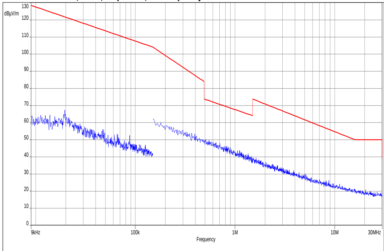
Plot 20: 9 kHz – 30 MHz, EUT8, stop mode, low frequency
