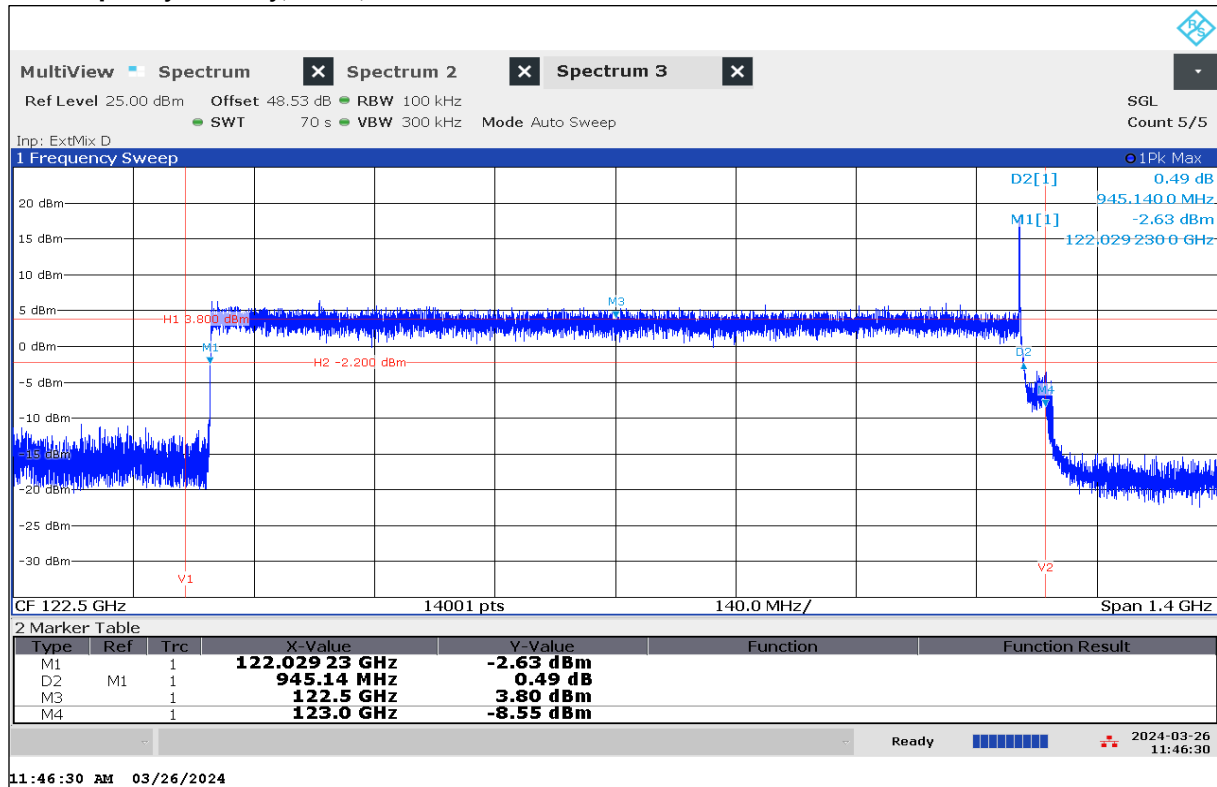
Plot 74: Frequency Stability, EUT7, +50 °C / V_{nom}
