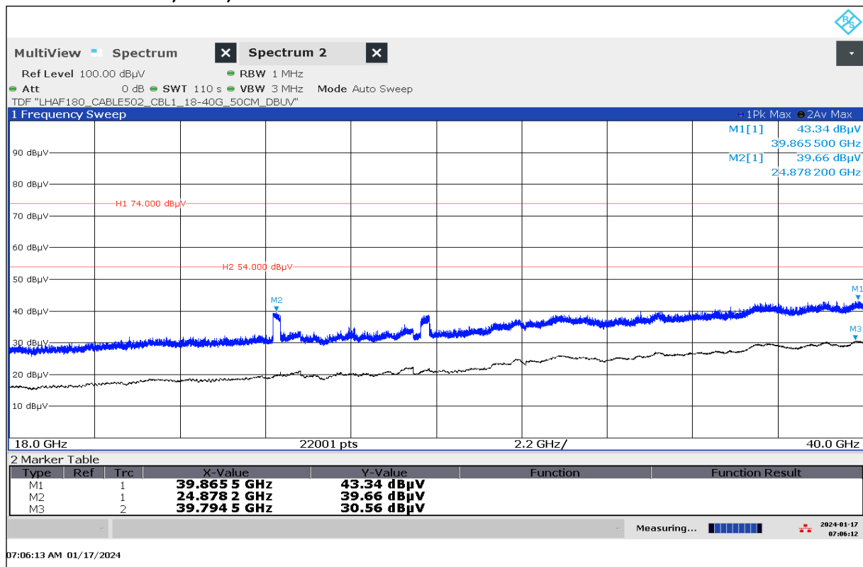
Plot 8: 18 GHz – 40 GHz, EUT7, normal mode
