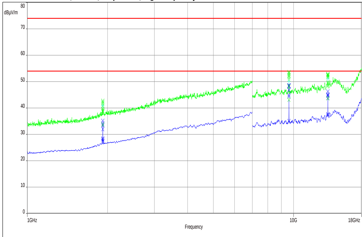
Plot 28: 1GHz – 18 GHz, EUT10, stop mode, high frequency
