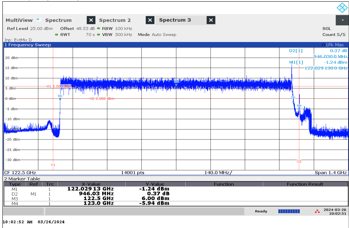
Plot 65: Frequency Stability, EUT7, -20 °C / V nom
