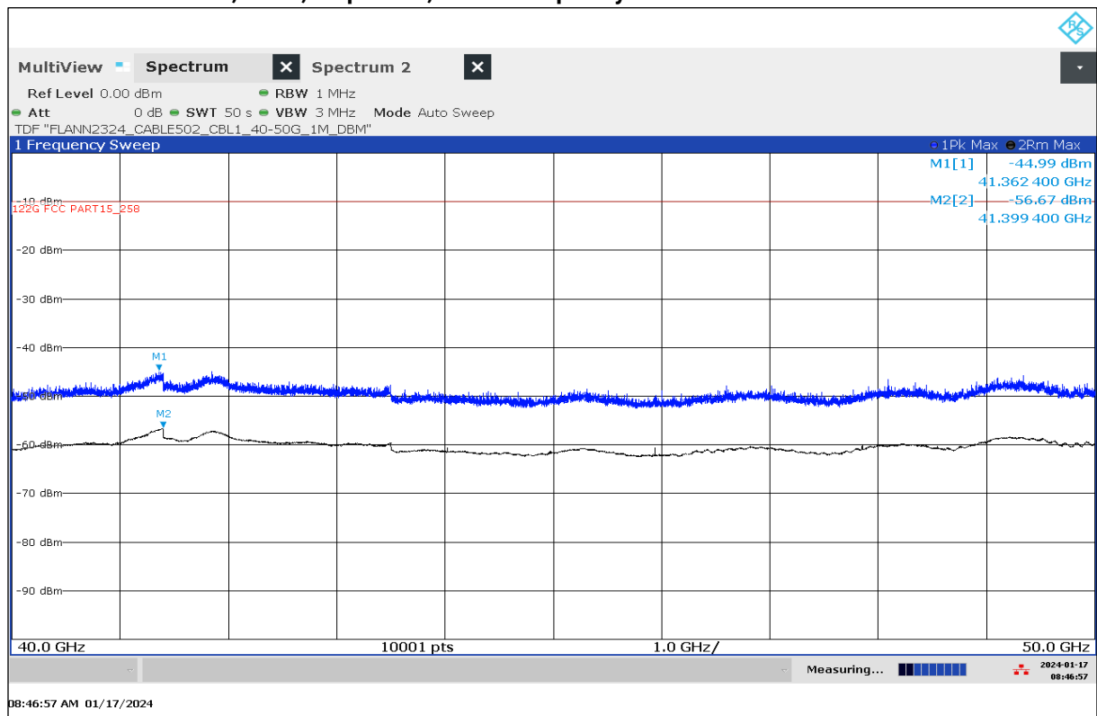
Plot 33: 40 GHz – 50 GHz, EUT9, stop mode, middle frequency
