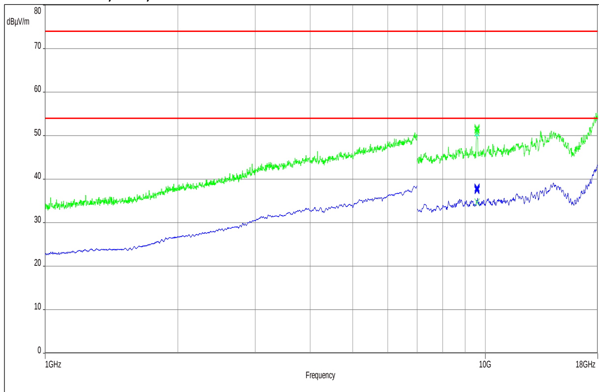
Plot 7: 1GHz – 18 GHz, EUT7, normal mode
