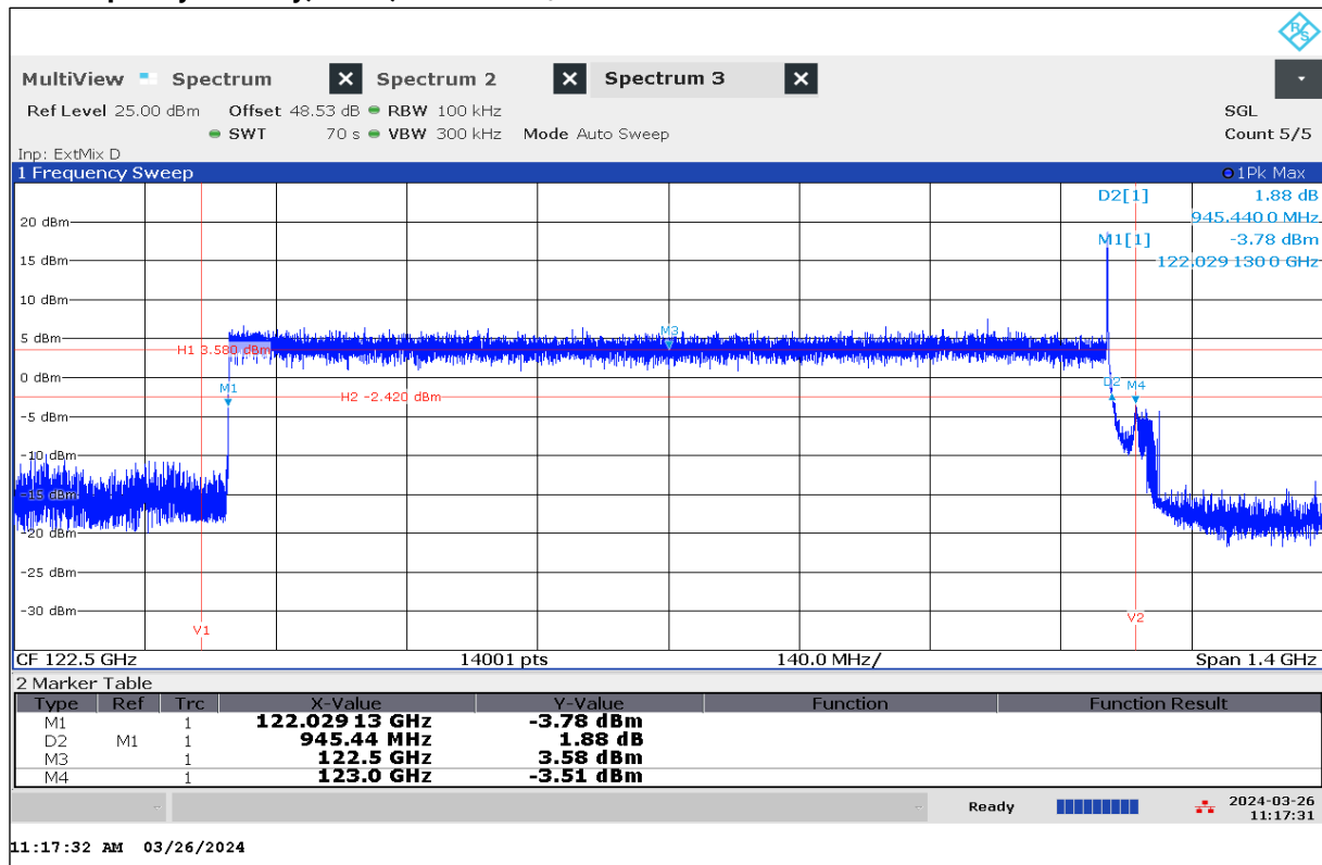
Plot 73: Frequency Stability, EUT7, +40 °C / V_{nom}
