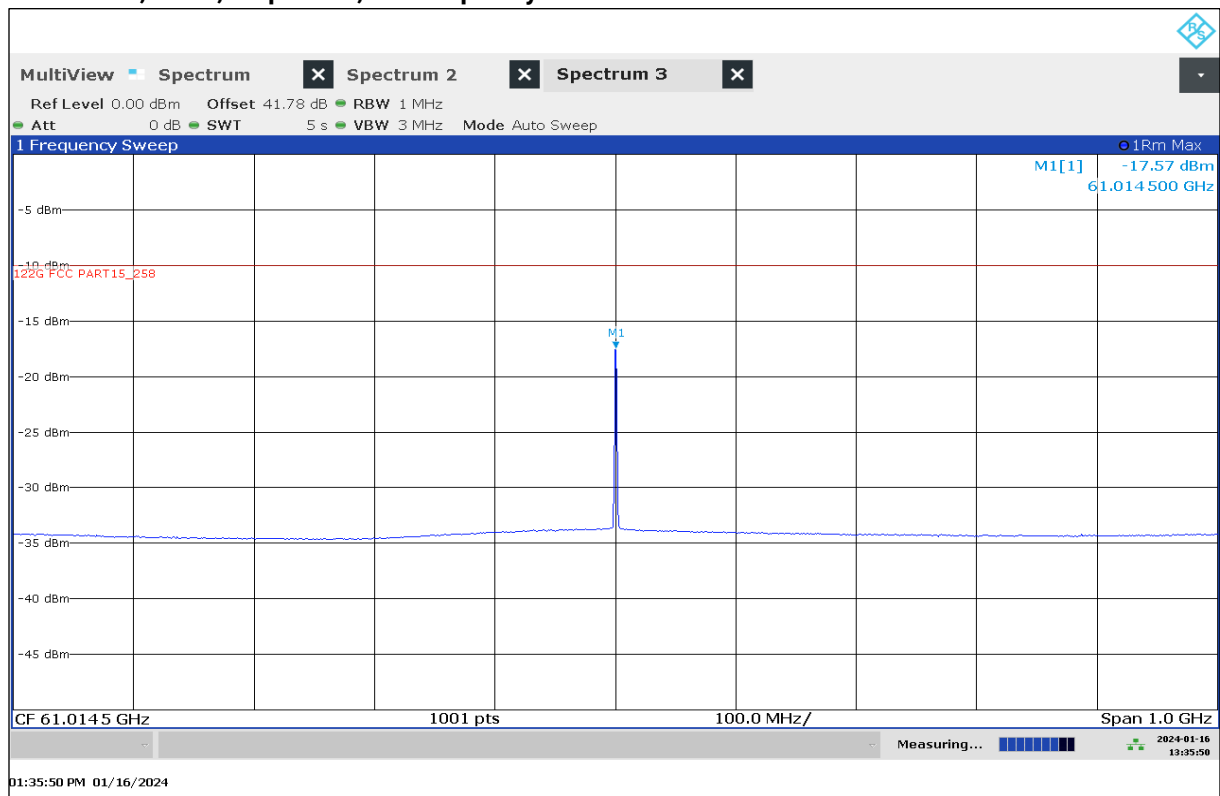
Plot 39: 61 GHz, EUT8, stop mode, low frequency
