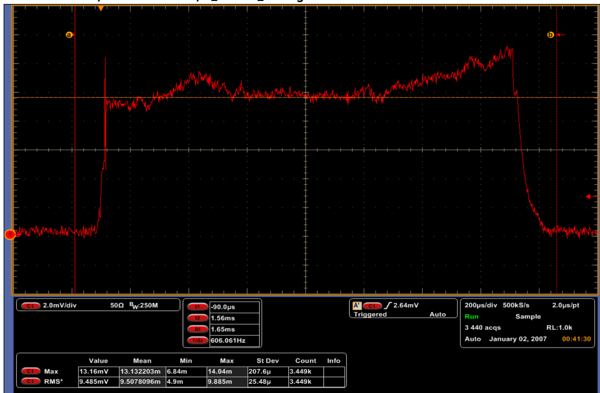
Plot 4: Normal mode, EUT 7 emission, V_max V_average
