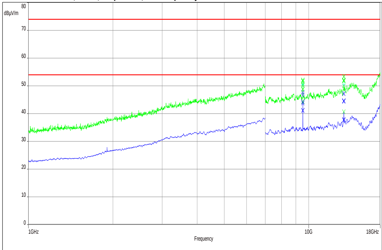
Plot 26: 1GHz – 18 GHz, EUT8, stop mode, low frequency
