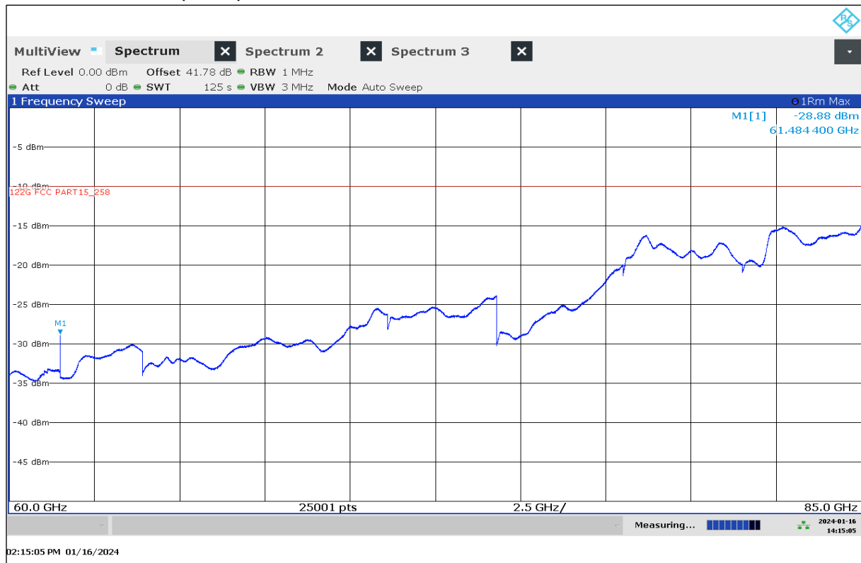
Plot 11: 60 GHz – 85 GHz, EUT7, normal mode
