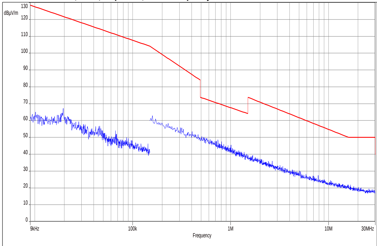
Plot 21: 9 kHz – 30 MHz, EUT9, stop mode, middle frequency
