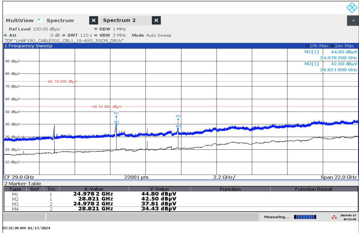
Plot 31: 18 GHz – 40 GHz, EUT10, stop mode, high frequency
