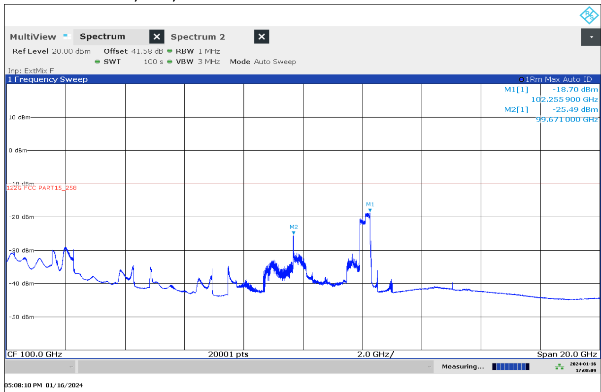
Plot 14: 90 GHz – 110 GHz, EUT7, normal mode
