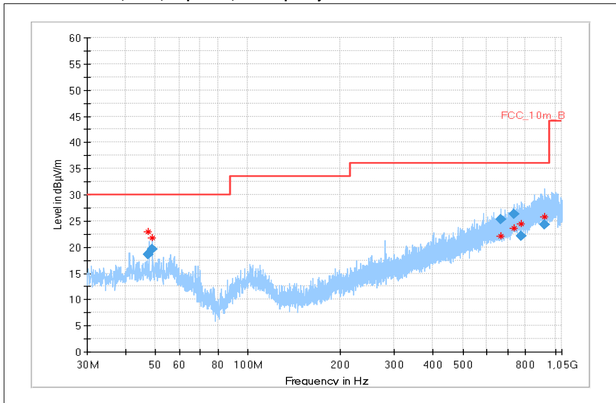
Plot 23: 30 MHz – 1GHz, EUT8, stop mode, low frequency
