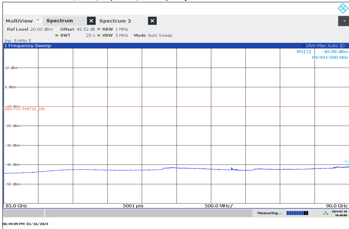
Plot 44: 85 GHz – 90 GHz, EUT8, stop mode, low frequency
