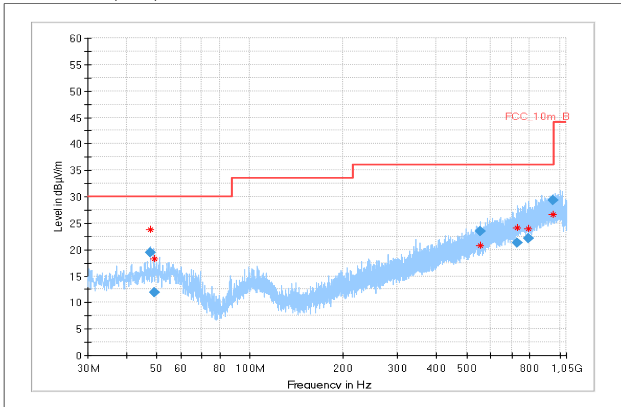
Plot 6: 30 MHz – 1GHz, EUT7, normal mode
