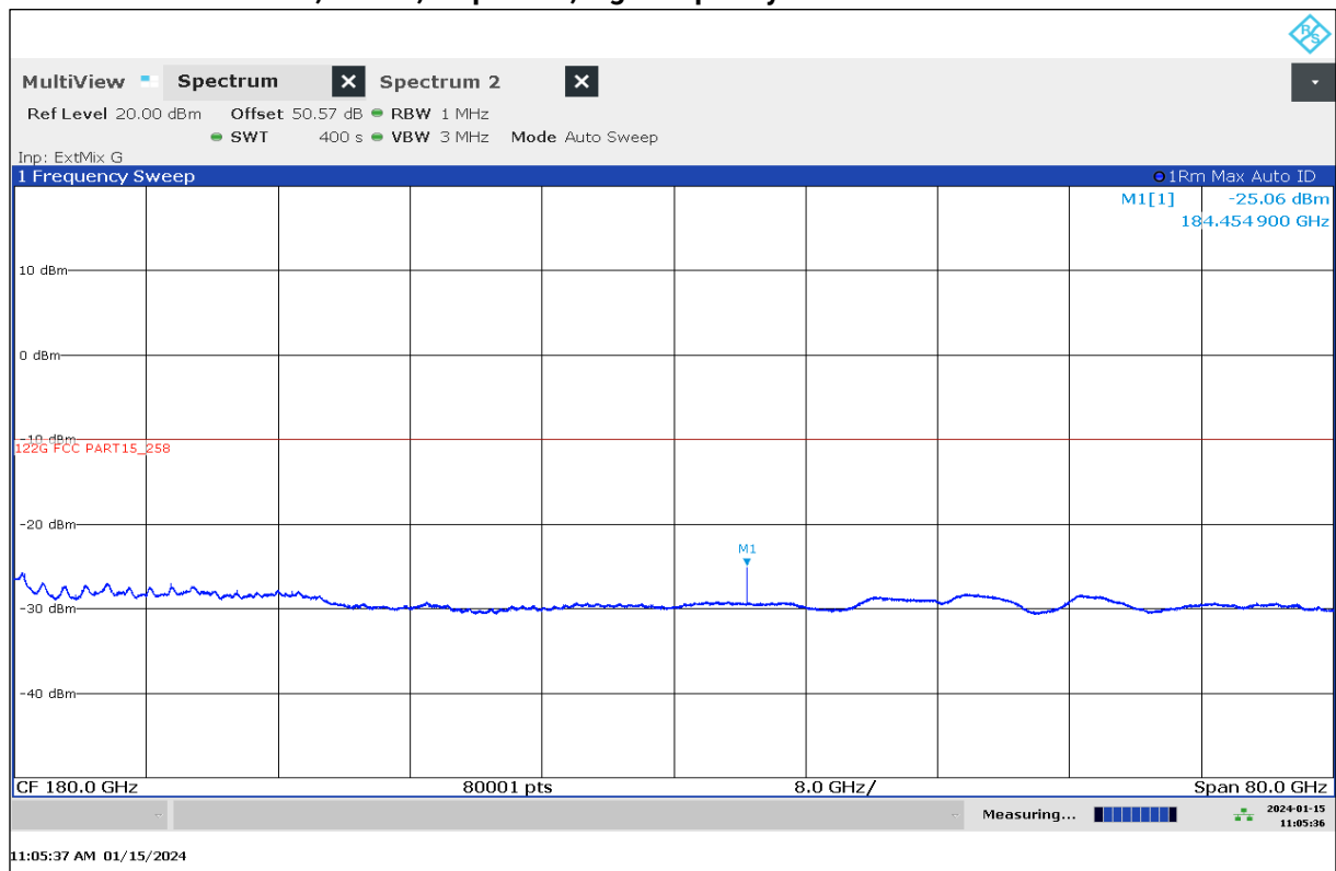
Plot 55: 140 GHz – 220 GHz, EUT10, stop mode, high frequency
