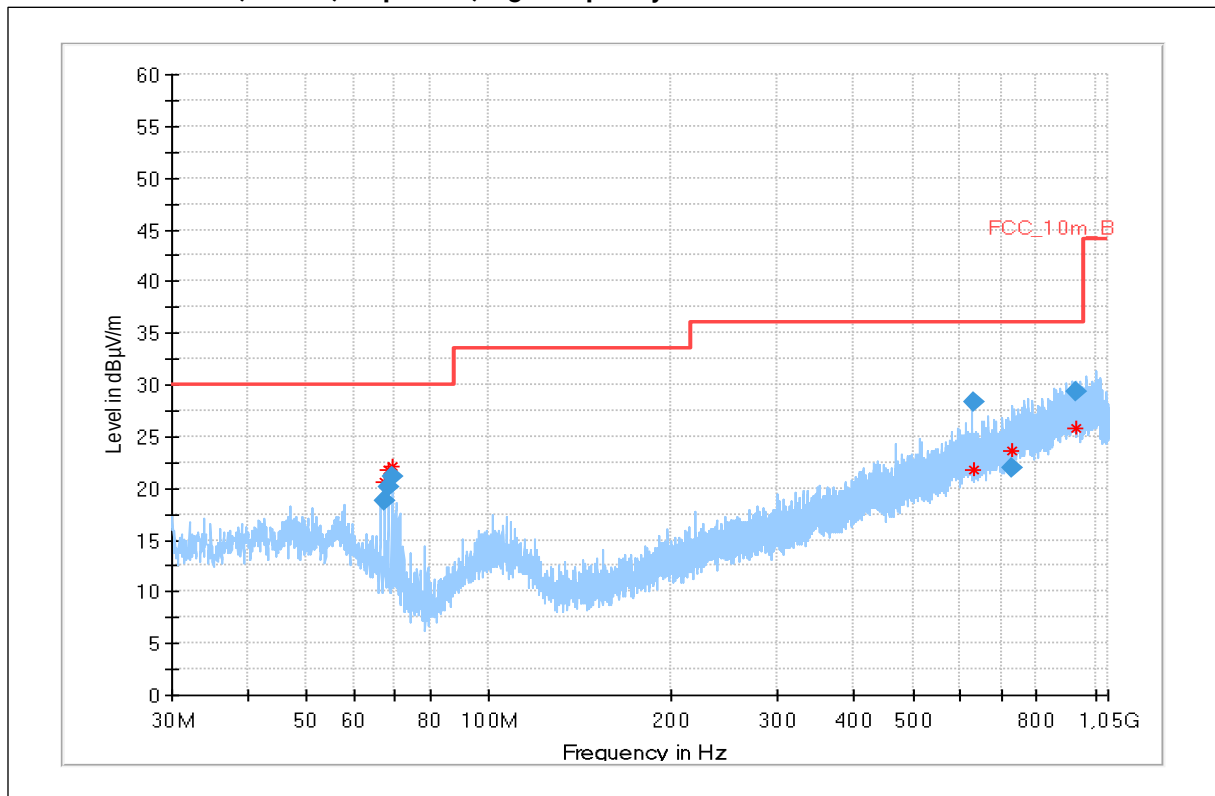
Plot 25: 30 MHz – 1GHz, EUT10, stop mode, high frequency
