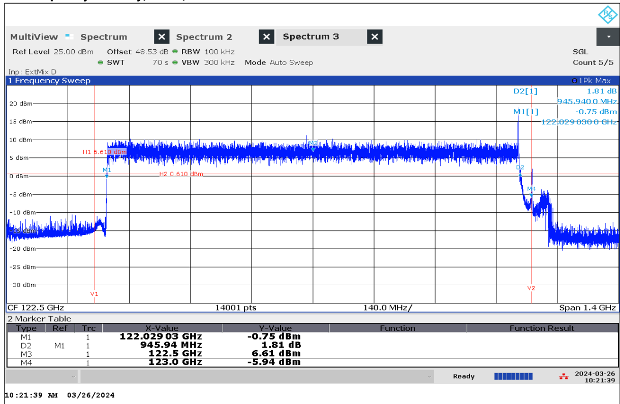
Plot 66: Frequency Stability, EUT7, -10 °C / V nom
