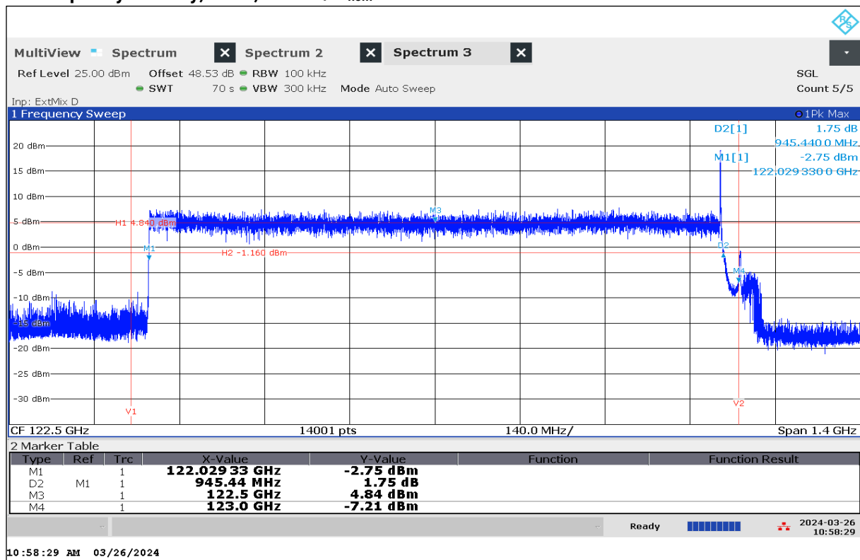
Plot 72: Frequency Stability, EUT7, +30 °C / V_{\text{nom}}
