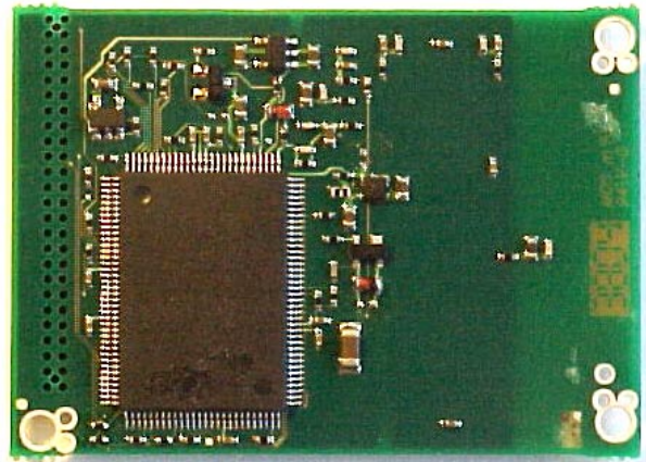
Module bottom view
