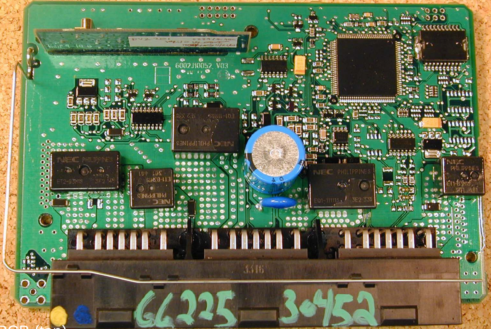
PCB (top)
