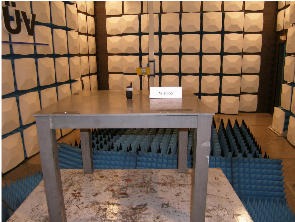
Photograph 4: Set-up for Spurious Radiation Emission Measurement above 1GHz
