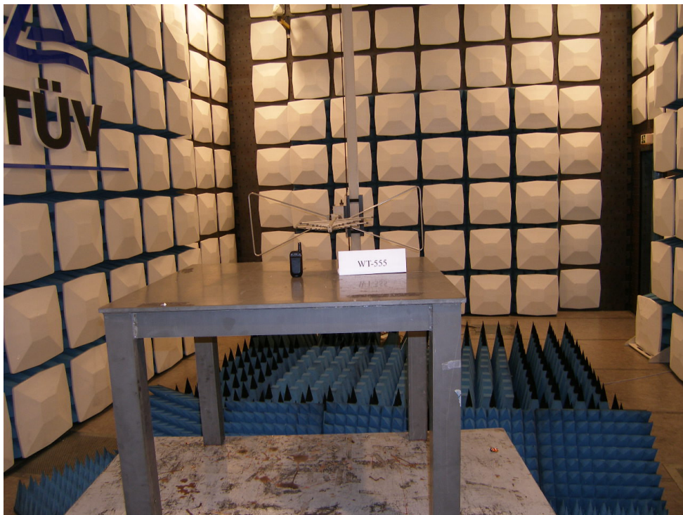
Photograph 3: Set-up for Spurious Radiation Emission Measurement below 1GHz
