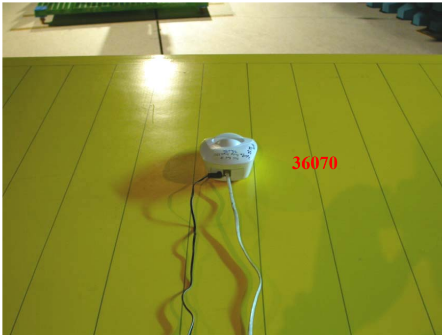
Photo 2: Radiated Emission Test Set-up photo (Base)
