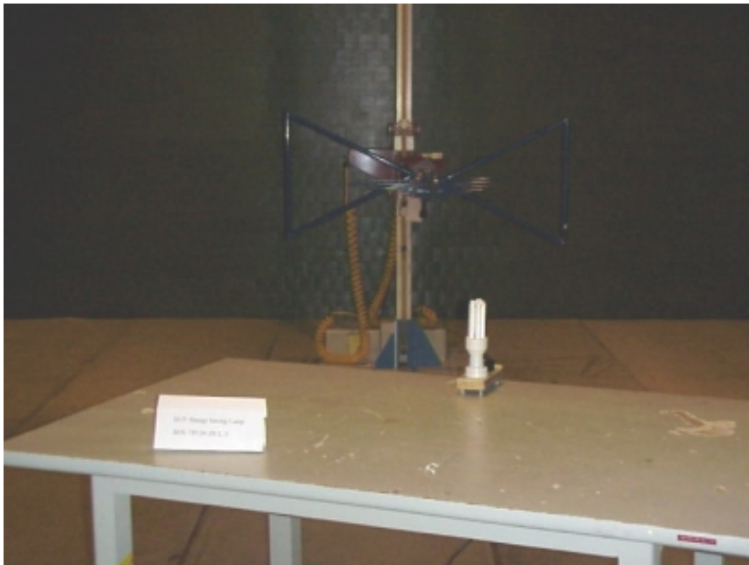
HORIZONTAL (M/N: TP120-20UL/3)
