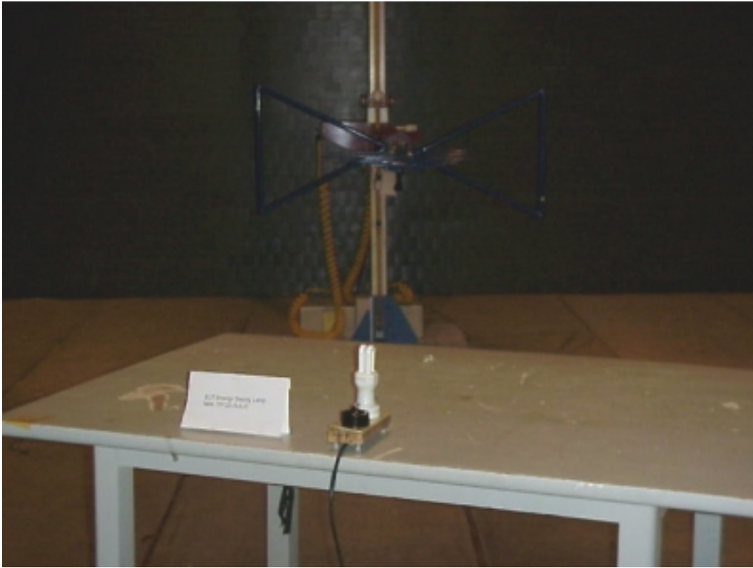
HORIZONTAL (M/N: TP120-5UL/2)
