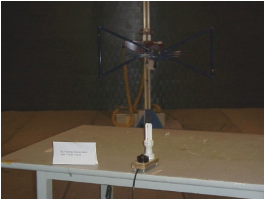
HORIZONTAL (M/N: TP120-11UL/2)
