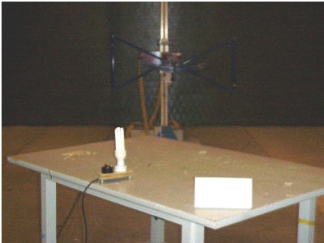
HORIZONTAL (M/N: TP120-25UL/3)
