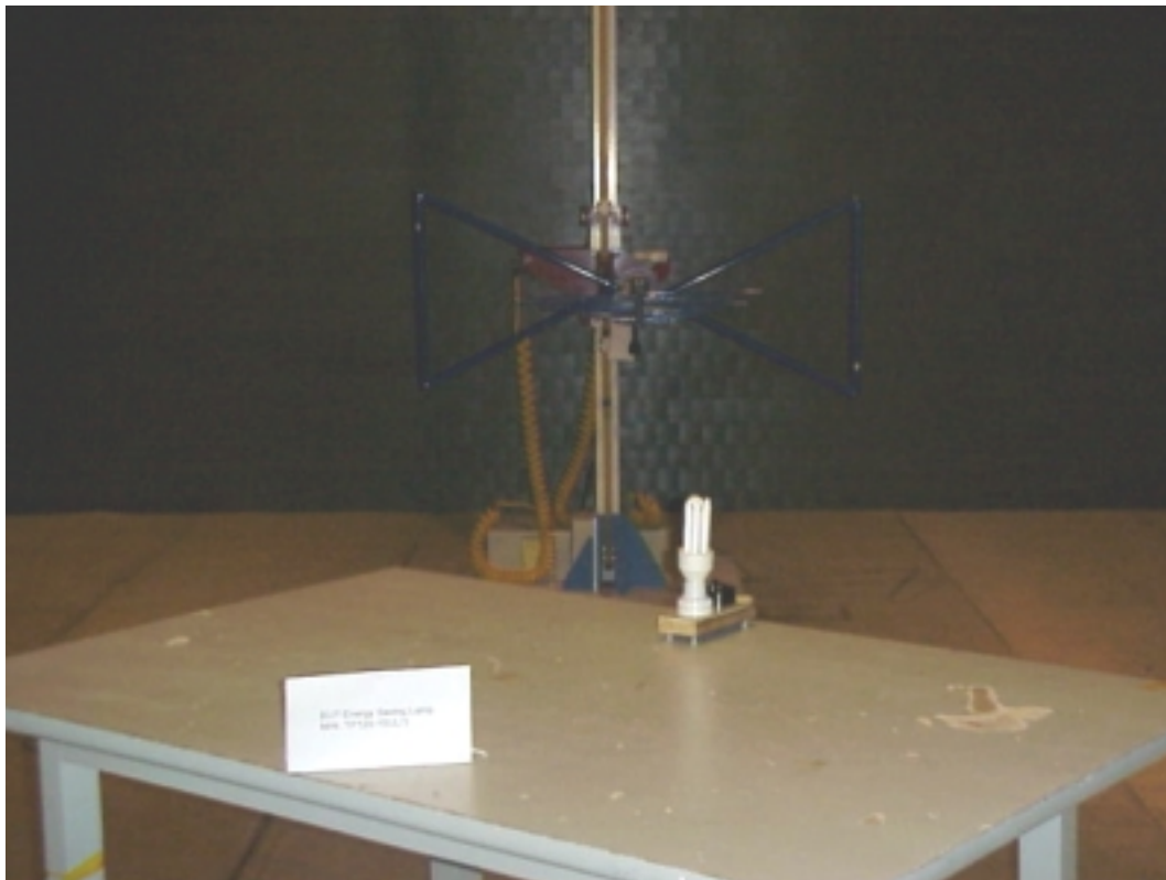
HORIZONTAL (M/N: TP120-15UL/3)
