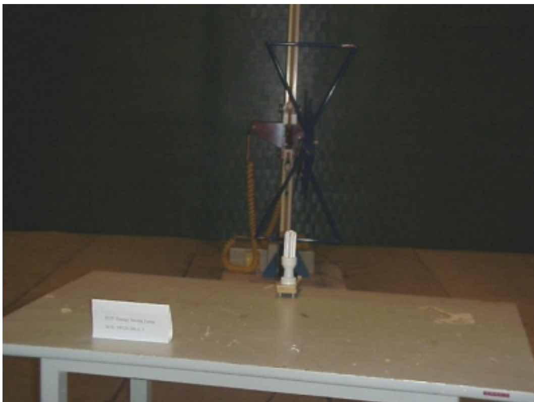
VERTICAL (M/N: TP120-20UL/3)
