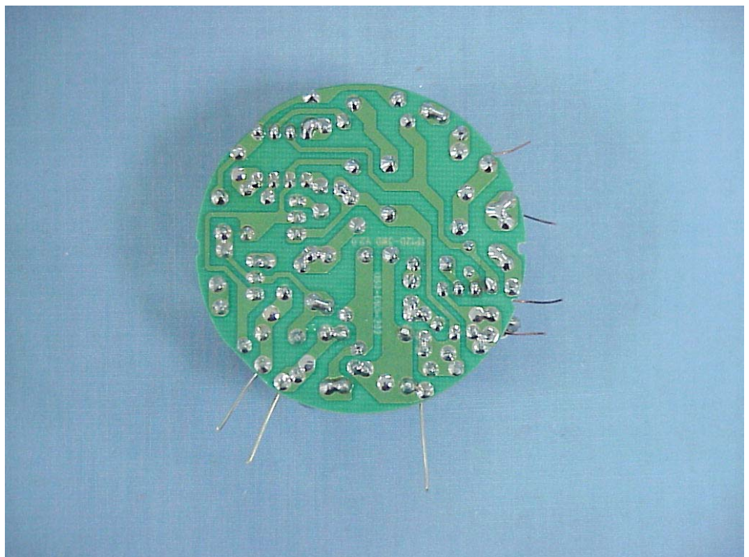
FIGURE 3 COMPACT FLUORESCENT LAMP (M/N: TP 120-25/20/13) MAIN BOARD (SOLDERED SIDE)
