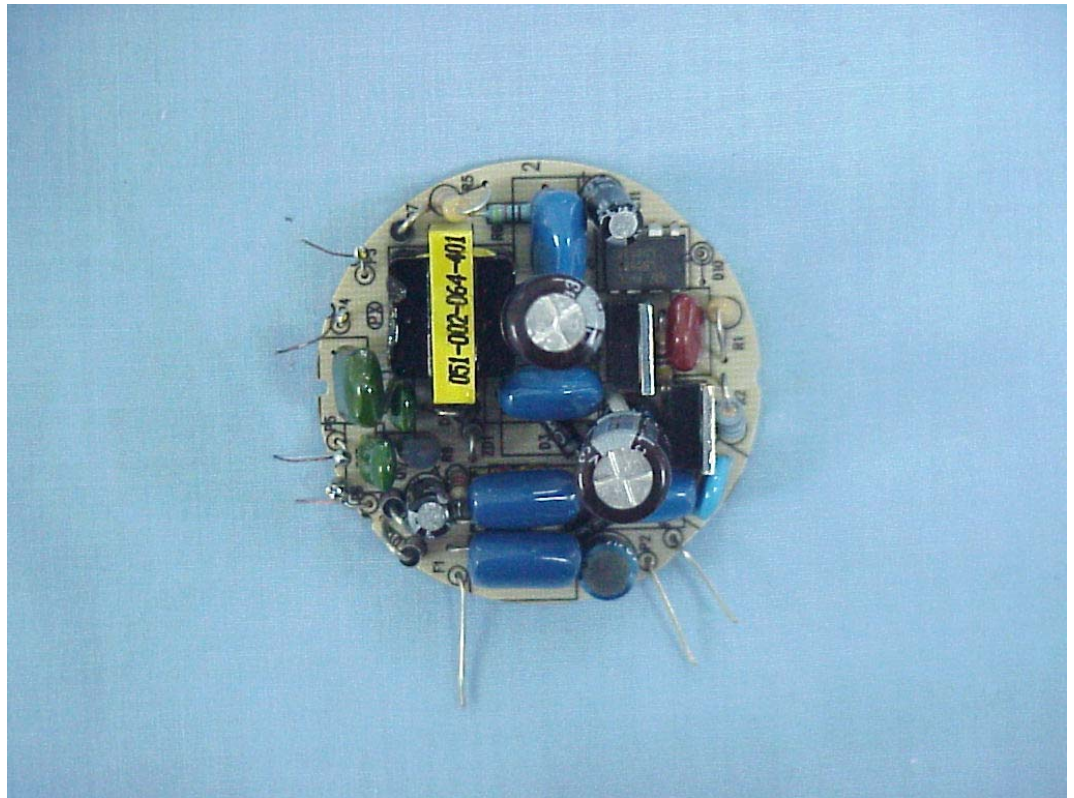
FIGURE 2 COMPACT FLUORESCENT LAMP (M/N: TP 120-25/20/13) MAIN BOARD (COMPONENT SIDE)
