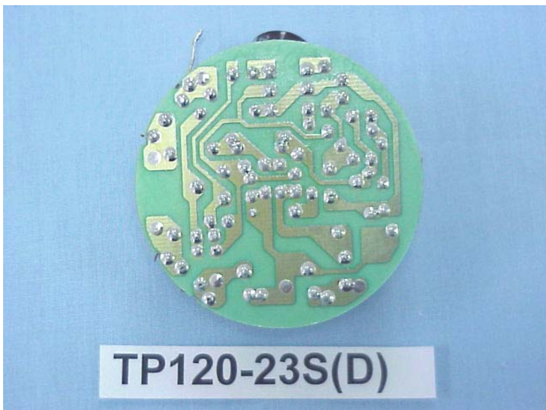
FIGURE 21 COMPACT FLUORESCENT LAMP (M/N: TP120-23S(D)) MAIN BOARD (SOLDERED SIDE)
