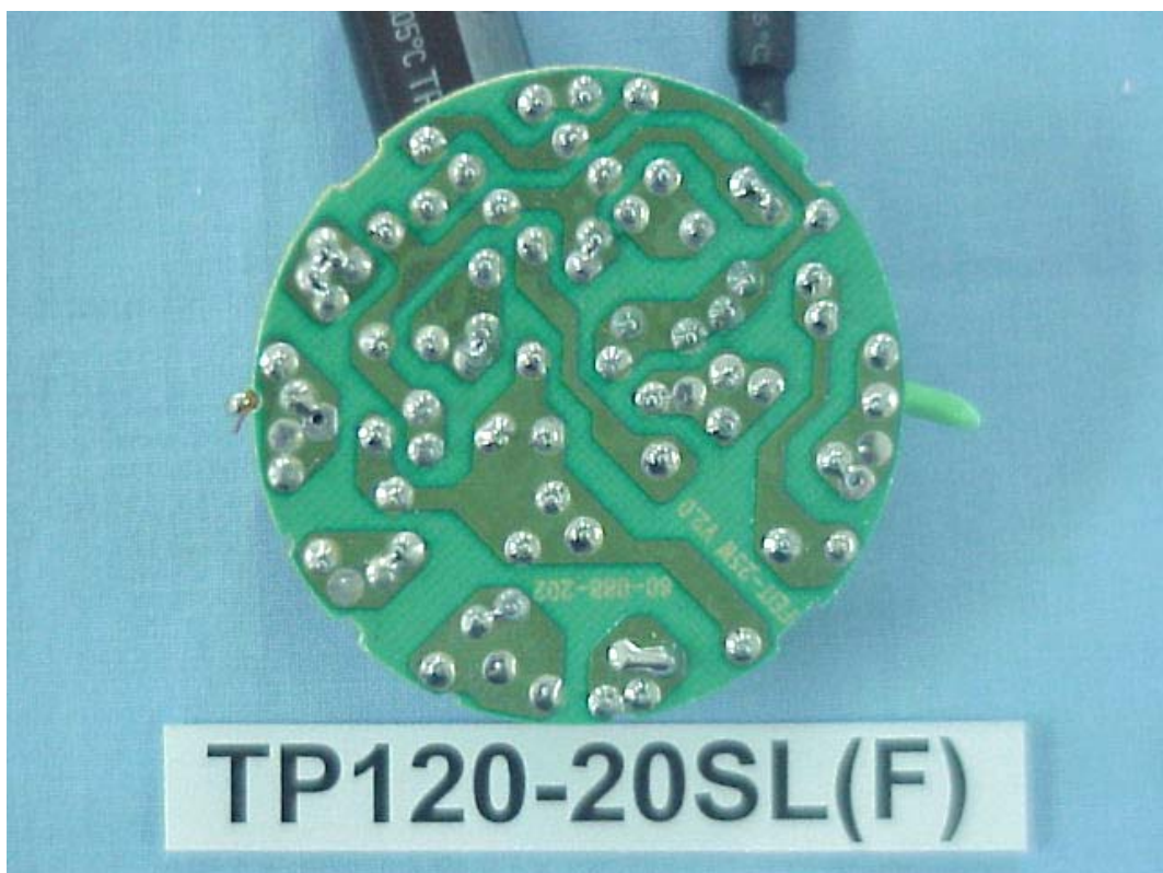
FIGURE 6 COMPACT FLUORESCENT LAMP (M/N: TP120-20SL(F)) MAIN BOARD (SOLDERED SIDE)
