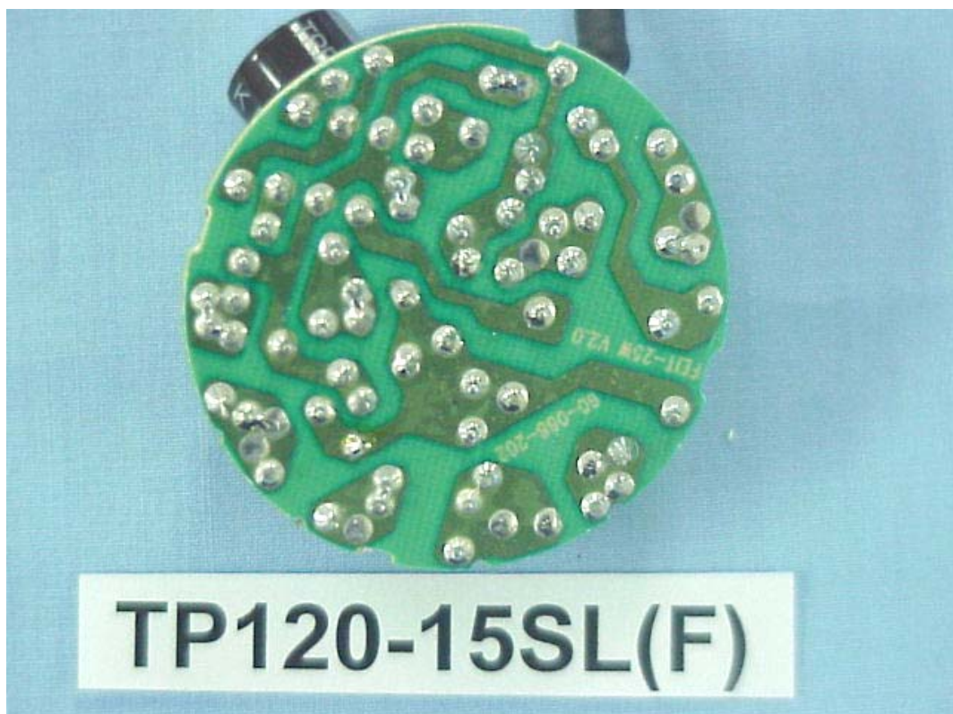
FIGURE 3 COMPACT FLUORESCENT LAMP (M/N: TP120-15SL) MAIN BOARD (SOLDERED SIDE)
