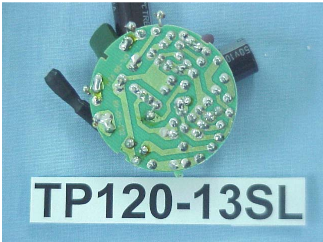
FIGURE 24 COMPACT FLUORESCENT LAMP (M/N: TP120-13SL) MAIN BOARD (SOLDERED SIDE)
