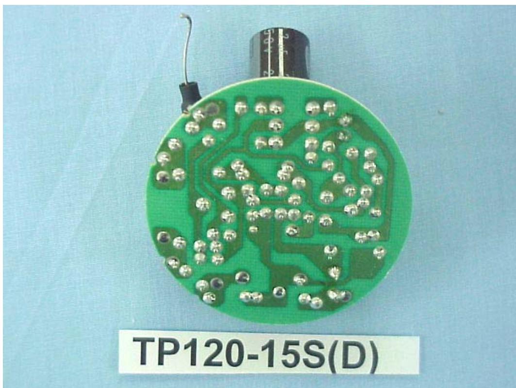
FIGURE 15 COMPACT FLUORESCENT LAMP (M/N: TP120-15S(D)) MAIN BOARD (SOLDERED SIDE)
