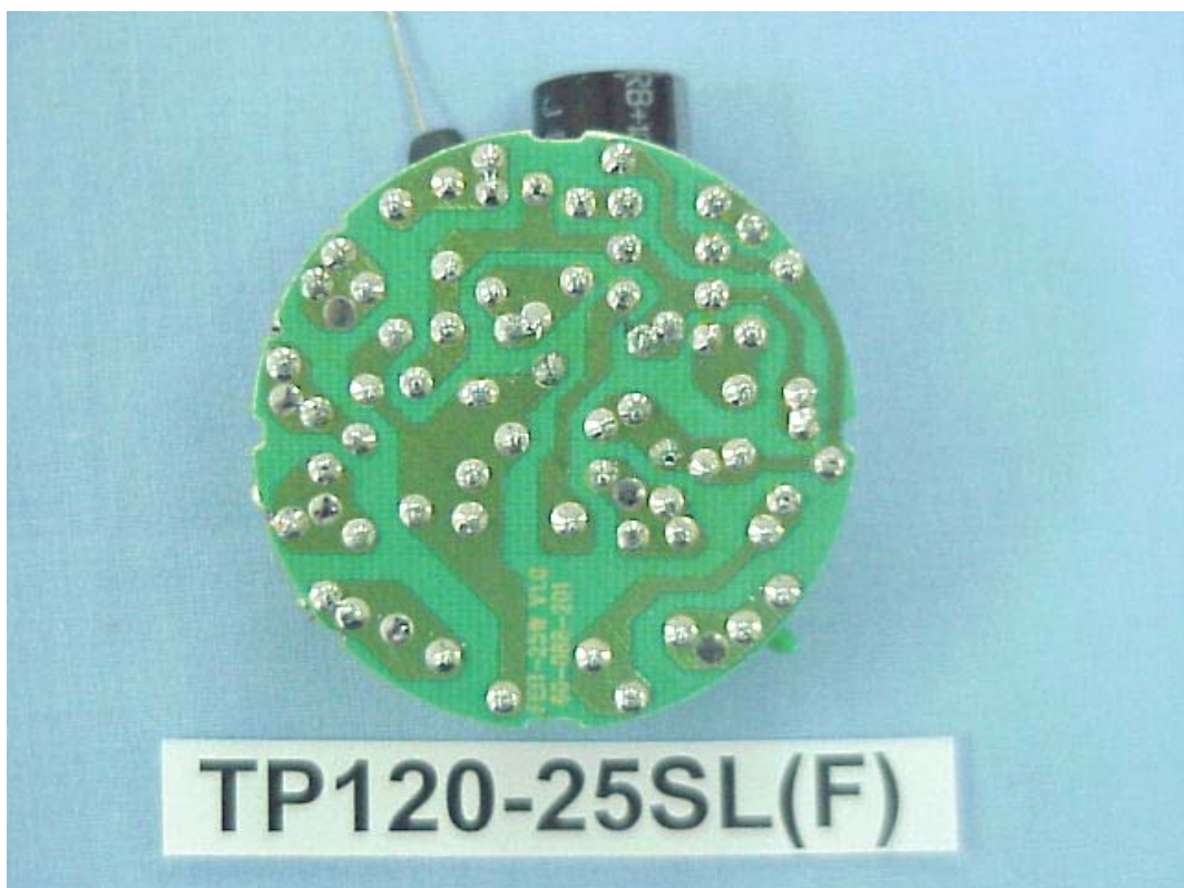
FIGURE 12 COMPACT FLUORESCENT LAMP (M/N: TP120-25SL(F)) MAIN BOARD (SOLDERED SIDE)
