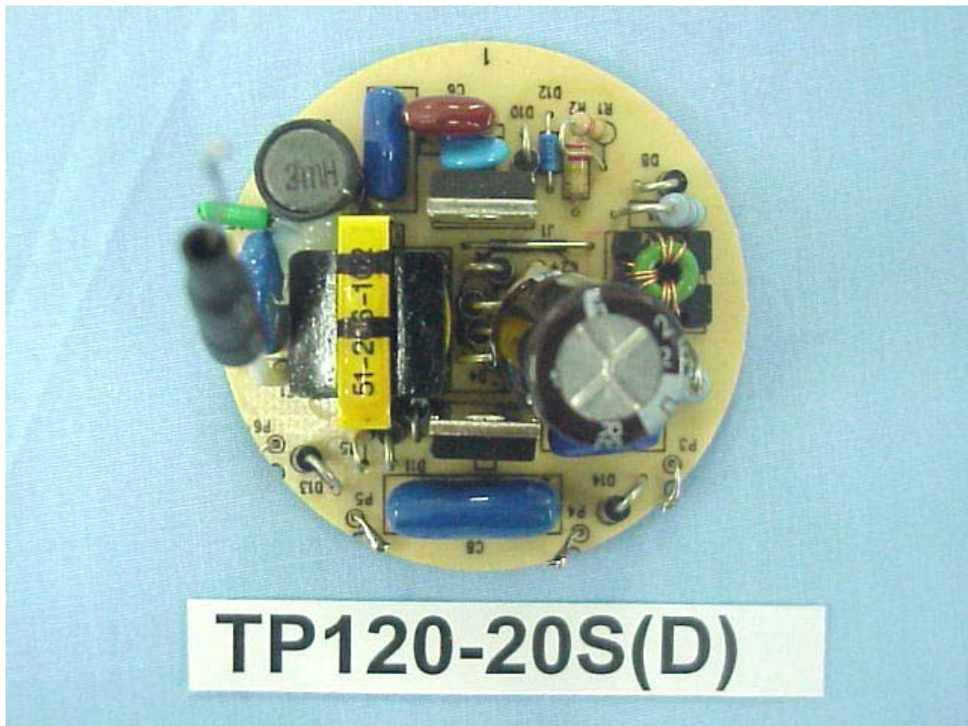
FIGURE 17 COMPACT FLUORESCENT LAMP (M/N: TP120-20S(D)) MAIN BOARD (COMPONENT SIDE)
