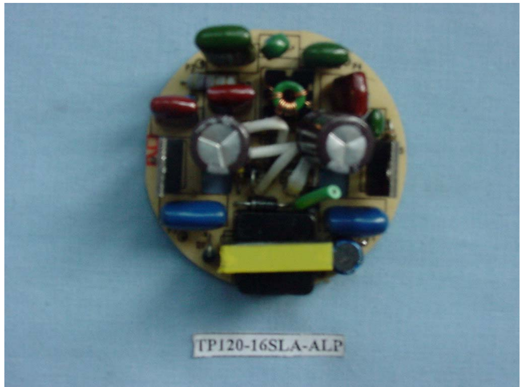
FIGURE 5 ENERGY SAVING LAMP (M/N: TP120-16SLA-ALP) MAIN BOARD (COMPONENT SIDE)
