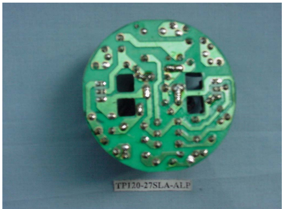
FIGURE 15 ENERGY SAVING LAMP (M/N: TP120-27SLA-ALP) MAIN BOARD (SOLDERED SIDE)
