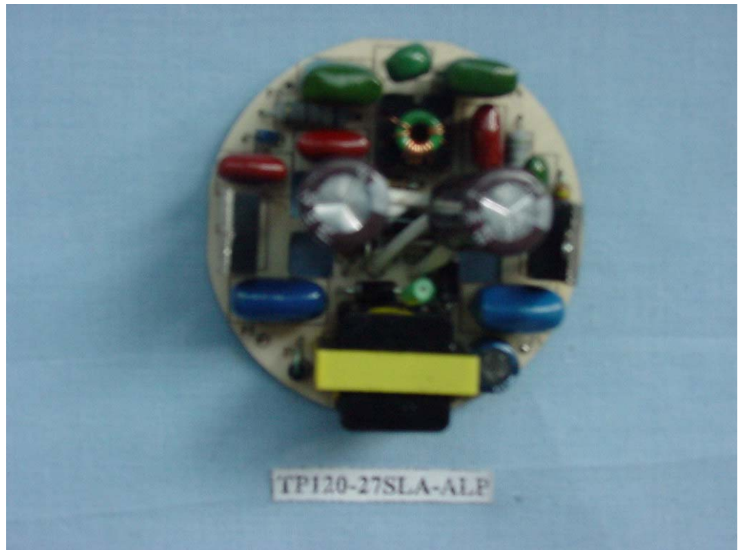
FIGURE 14 ENERGY SAVING LAMP (M/N: TP120-27SLA-ALP) MAIN BOARD (COMPONENT SIDE)
