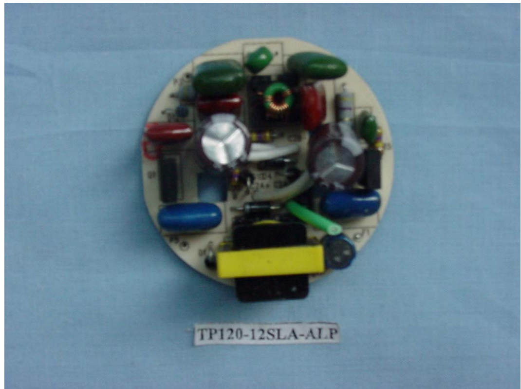
FIGURE 2 ENERGY SAVING LAMP (M/N: TP120-12SLA-ALP) MAIN BOARD (COMPONENT SIDE)
