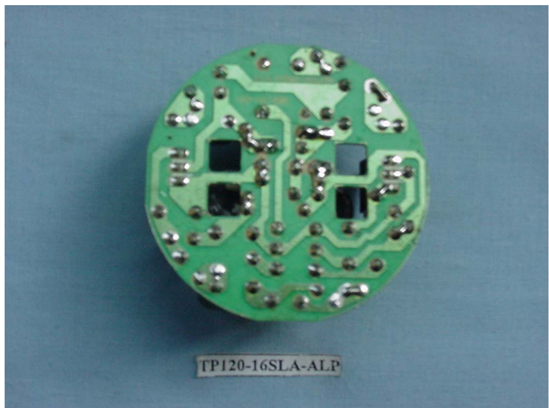
FIGURE 6 ENERGY SAVING LAMP (M/N: TP120-16SLA-ALP) MAIN BOARD (SOLDERED SIDE)
