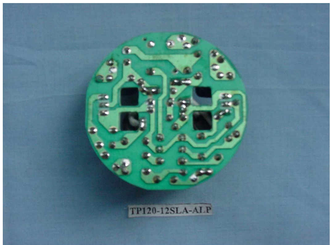
FIGURE 3 ENERGY SAVING LAMP (M/N: TP120-12SLA-ALP) MAIN BOARD (SOLDERED SIDE)
