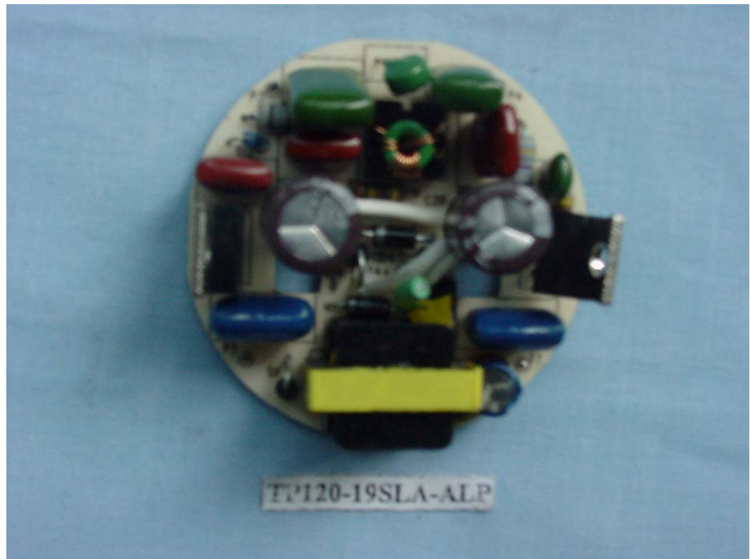
FIGURE 8 ENERGY SAVING LAMP (M/N: TP120-19SLA-ALP) MAIN BOARD (COMPONENT SIDE)
