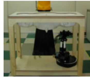
Figure 8. SAM Phantom
