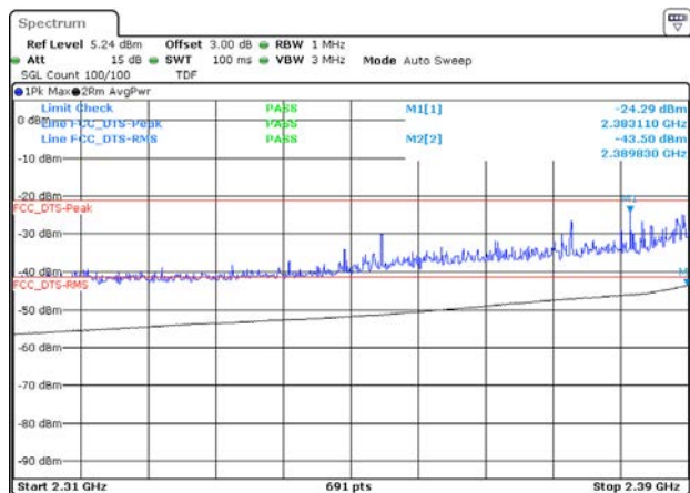
BE-R-LOW, SISO-B, 802.11ax20-HE0, Ch1
