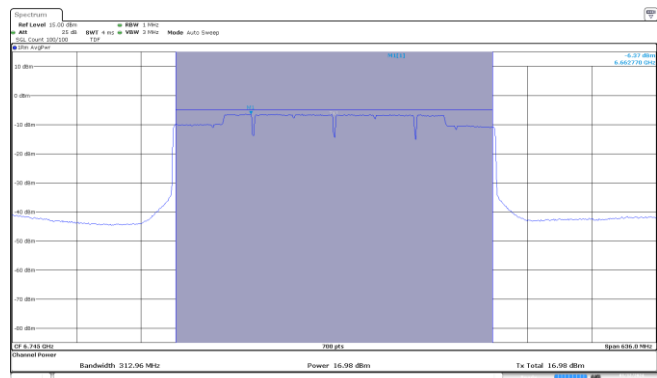
SISO A-802.11ax/be-320MHz-Ch159-6745MHz-MCS0
