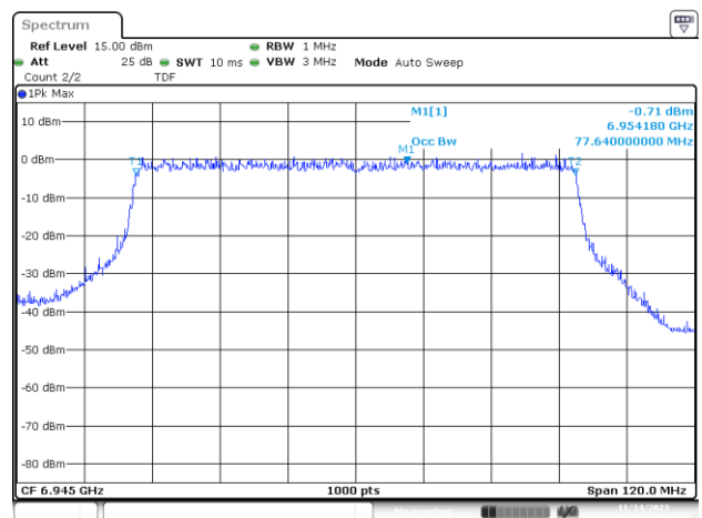
UNII8 MIMO B 802.11ax/be80 ch1799 6945MHz 99%
