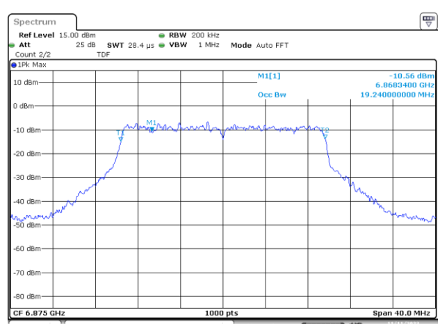
UNII8 MIMO A 802.11ax/be20 ch181 6875MHz 99%
