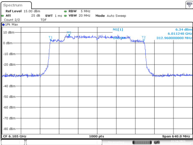
UNII5 MIMO B 802.11be320 ch31 6105MHz 99%
