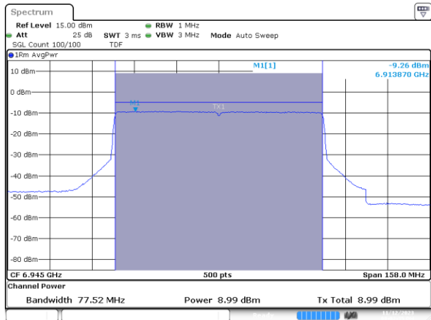
MIMO A-802.11ax/be-80MHz-Ch199-6945MHz-MCS0
