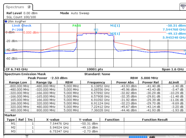
MIMO B-802.11ax/be-320MHz-Ch159-6745MHz-MCS0
