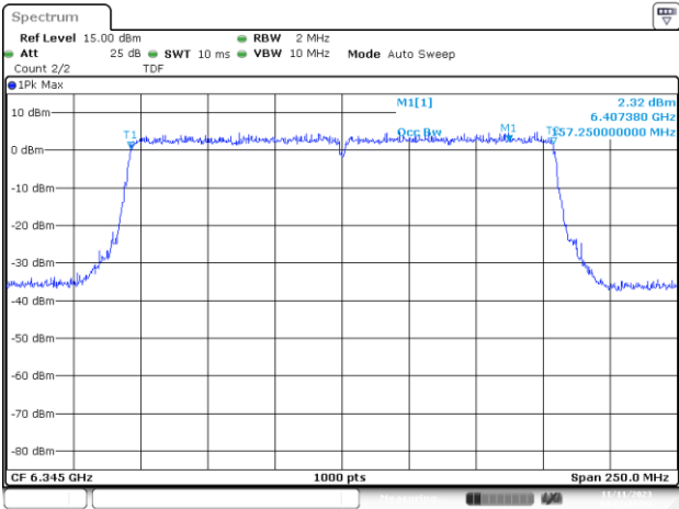
UNII5 MIMO A 802.11ax/be160 ch79 6345MHz 99%
