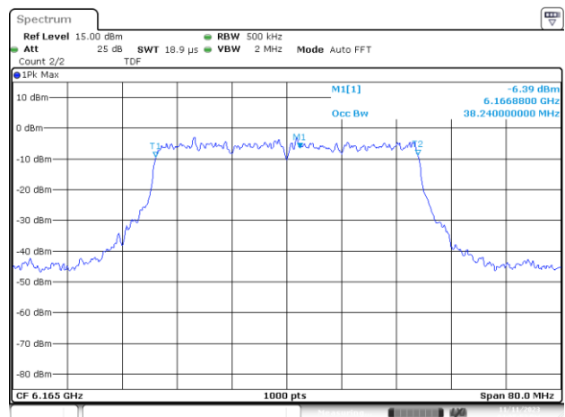
UNII5 MIMO A 802.11ax/be40 ch43 6165MHz 99%
