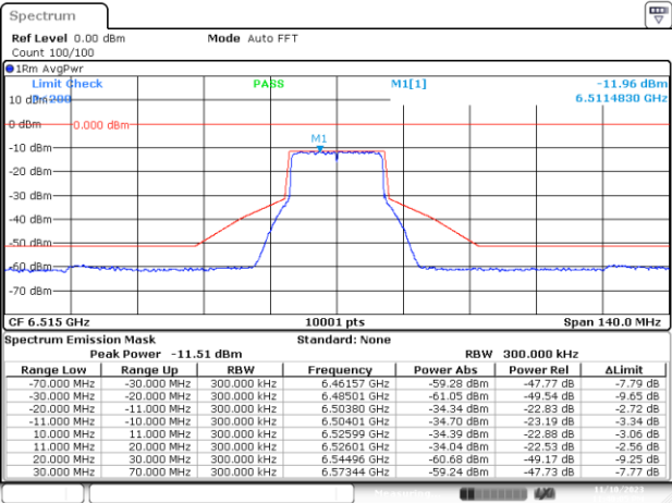
SISO A-802.11ax/be-20MHz-Ch113-6515MHz-MCS0
