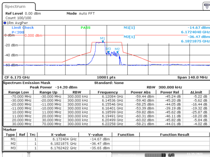
MIMO-B, 802.11ax/be20-MCS0, Ch45-6m-70
