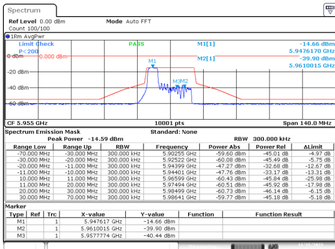
MIMO-B, 802.11ax/be20-MCS0, Ch1-4m-37
