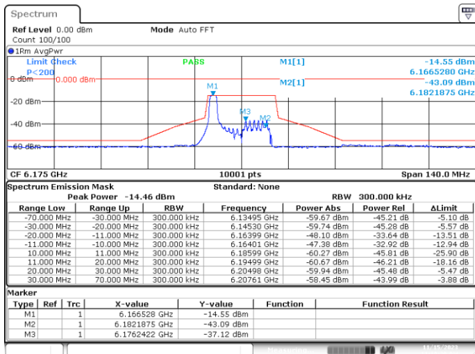
MIMO-B, 802.11ax/be20-MCS0, Ch45-2m-0
