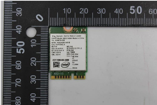
Adaptor Front
