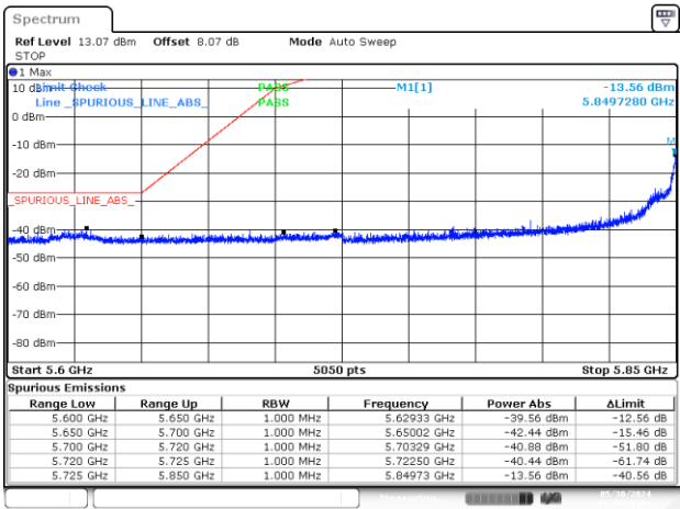
BE-NR-LOW, SISO-B, 802.11ax/be20-MCS0, Ch173
