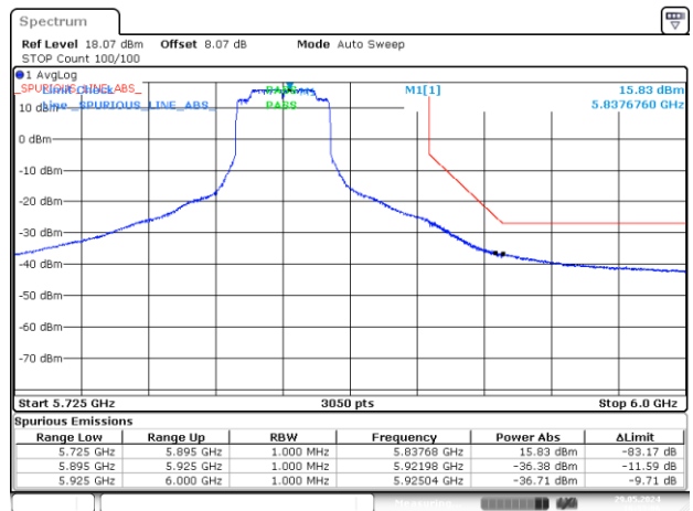
BE-NR-HIGH, SISO-A, 802.11ax/be40-MCS0, Ch167
