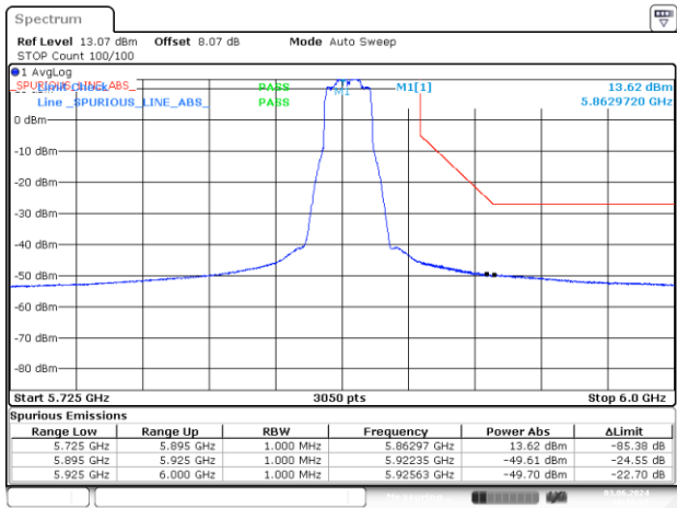
BE-NR-HIGH, SISO-A, 802.11ax/be20-MCS0, Ch173
