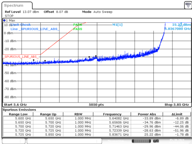
BE-NR-LOW, SISO-B, 802.11ax/be40-MCS0, Ch167
