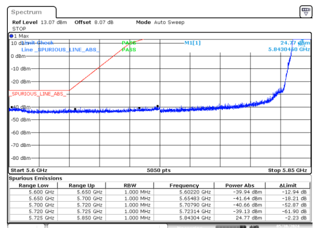
BE-NR-LOW, SISO-B, 802.11ax/be20-MCS0, Ch169
