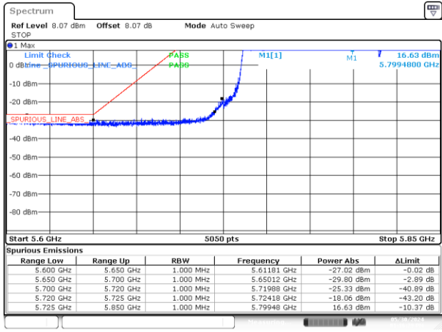
BE-NR-LOW, SISO-A, 802.11ax/be160-MCS0, Ch163
