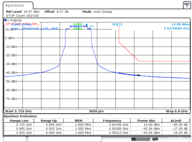
BE-NR-HIGH, SISO-B, 802.11ax/be40-MCS0, Ch167
