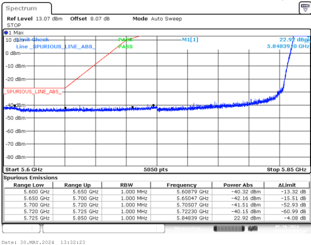
BE-NR-LOW, SISO-B, 802.11a20-6Mbps, Ch169
