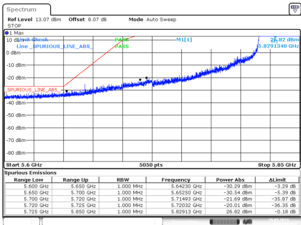
BE-NR-HIGH-PEAK, SISO-A, 802.11ax/be20-MCS0, Ch177
