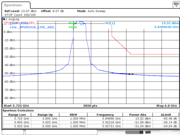
BE-NR-HIGH, SISO-B, 802.11ax/be20-MCS0, Ch169
