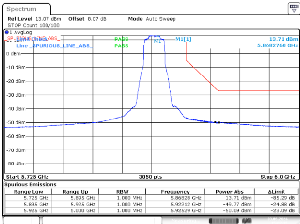
BE-NR-HIGH, SISO-B, 802.11ax/be20-MCS0, Ch173
