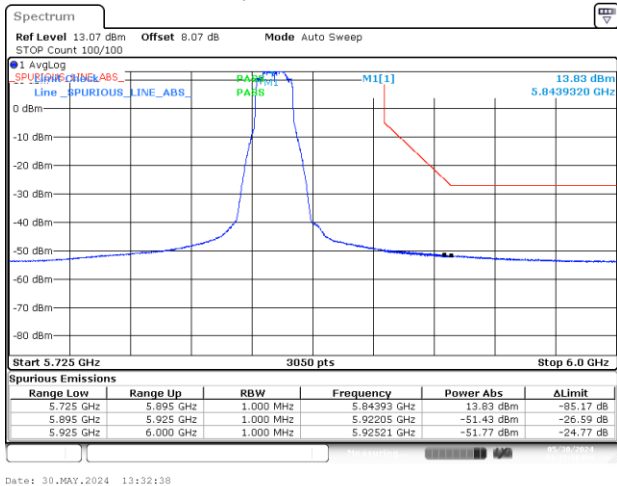
BE-NR-HIGH, SISO-B, 802.11a20-6Mbps, Ch169
