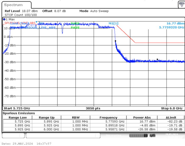
BE-NR-HIGH-PEAK, SISO-A, 802.11ax/be160-MCS0, Ch163
