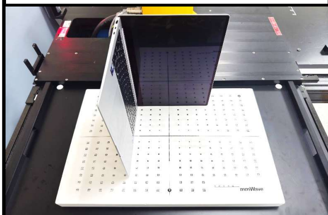
Left Side of Panel Tested at 25 mm
