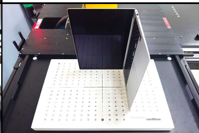
Right Side of Panel Tested at 25 mm
