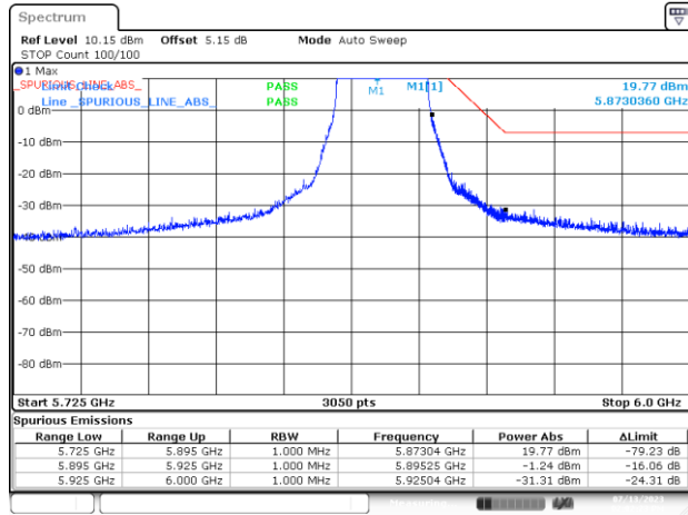
BE-NR-HIGH-PEAK, MIMO-A, 802.11n40-HT8, Ch175
