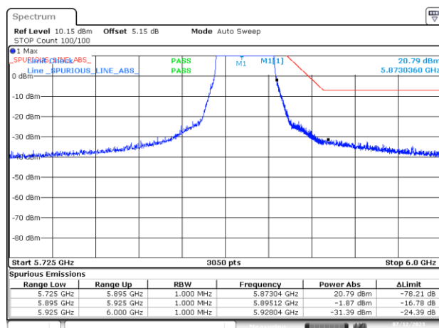
BE-NR-HIGH-PEAK, MIMO-B, 802.11n40-HT8, Ch175
