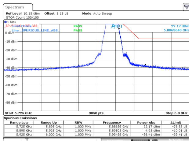
BE-NR-HIGH-PEAK, SISO-B, 802.11n20-HT0, Ch177
