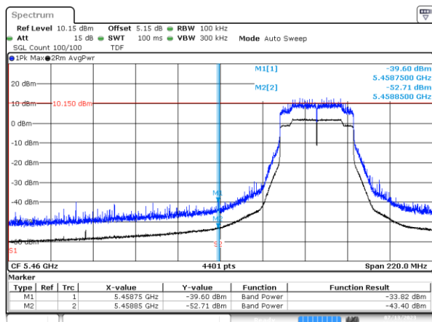
BE-R-LOW, SISO-A, 802.11ax/be40-MCS0, Ch102
