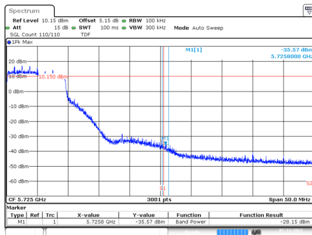
BE-NR-HIGH, SISO-A, 802.11ax/be20-MCS0, Ch140
