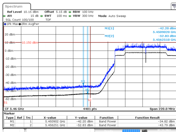
BE-R-LOW, SISO-A, 802.11ax/be80-MCS0, Ch106
