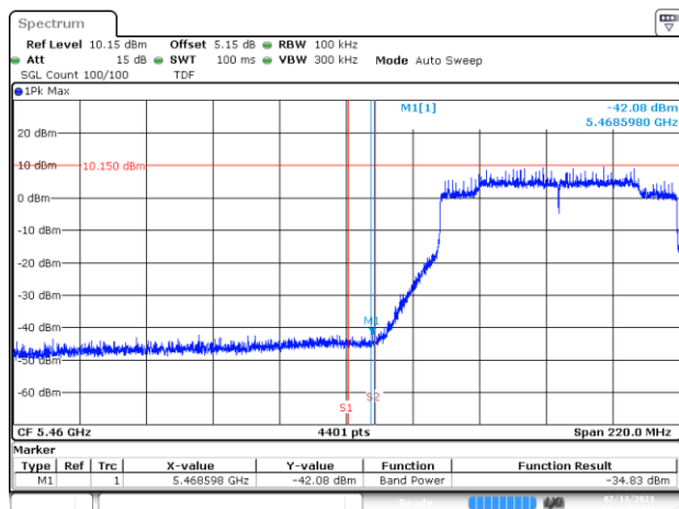
BE-NR-LOW, SISO-A, 802.11ax/be80-MCS0, Ch106
