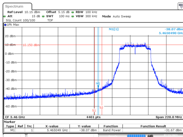
BE-NR-LOW, SISO-A, 802.11ax/be40-MCS0, Ch102
