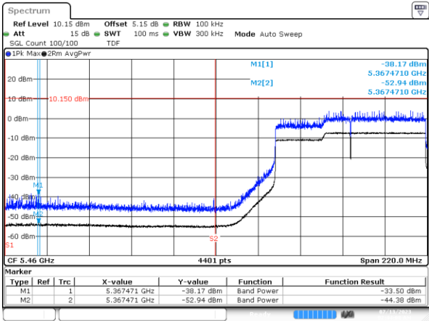
BE-R-LOW, SISO-A, 802.11ax/be160-MCS0, Ch114
