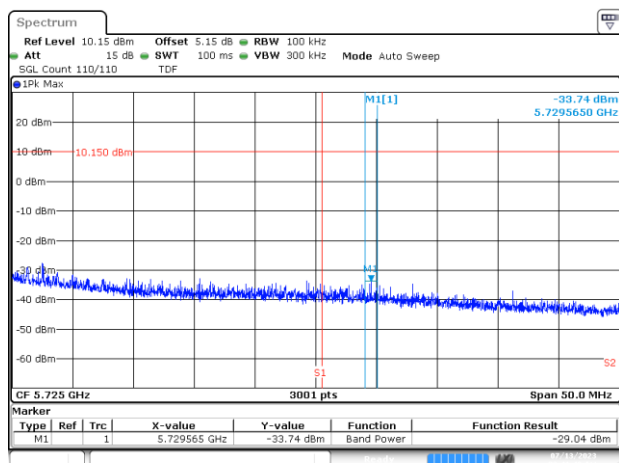
BE-NR-HIGH, SISO-A, 802.11ax/be40-MCS0, Ch134
