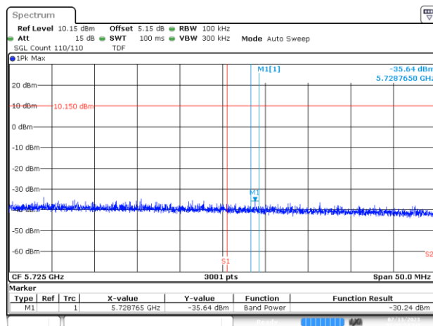
BE-NR-HIGH, SISO-A, 802.11ax/be80-MCS0, Ch122
