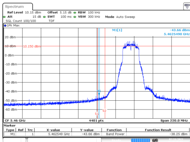
BE-NR-LOW, SISO-A, 802.11ax/be20-MCS0, Ch100
