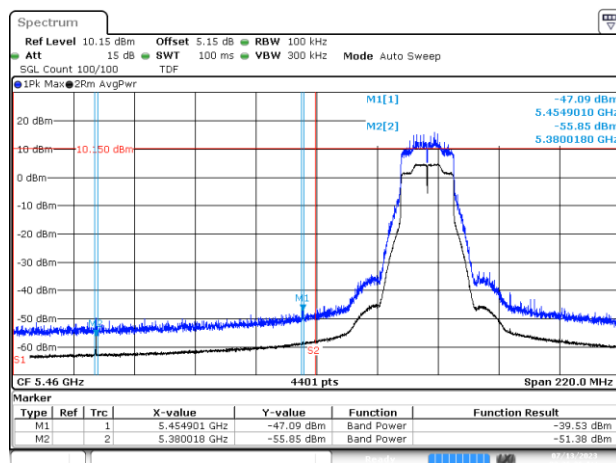
BE-R-LOW, SISO-A, 802.11ax/be20-MCS0, Ch100
