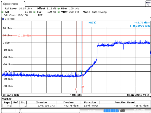
BE-NR-LOW, SISO-A, 802.11ax/be160-MCS0, Ch114
