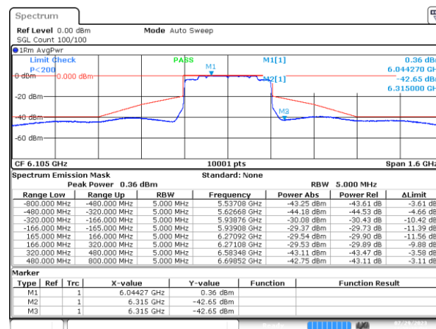
MIMO A-802.11be-320MHz-Ch31-6105MHz-MCS0
