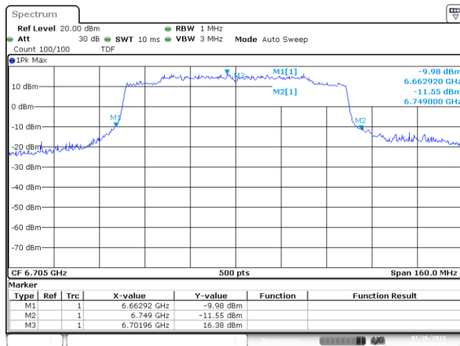
UNII7 SISO A 802.11ax/be80 ch151 6705MHz 26dB
