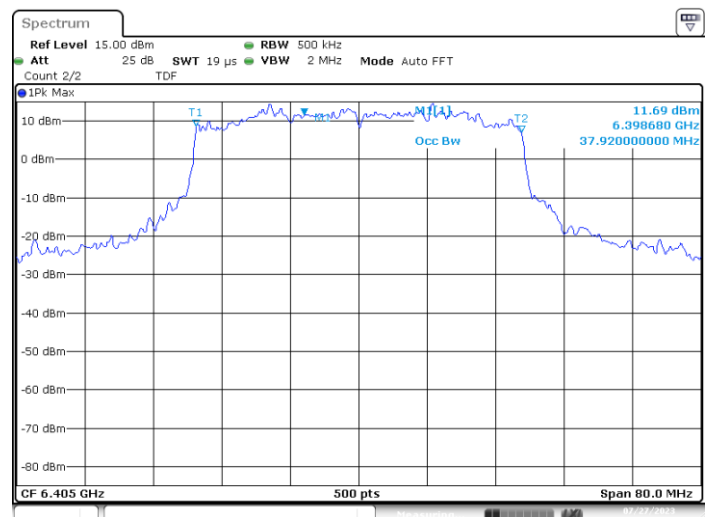
UNII5 MIMO A 802.11ax/be40 ch91 6405MHz 99%
