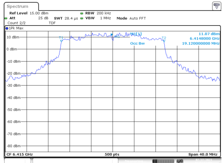
UNII5 SISO A 802.11ax/be20 ch93 6415MHz 99%
