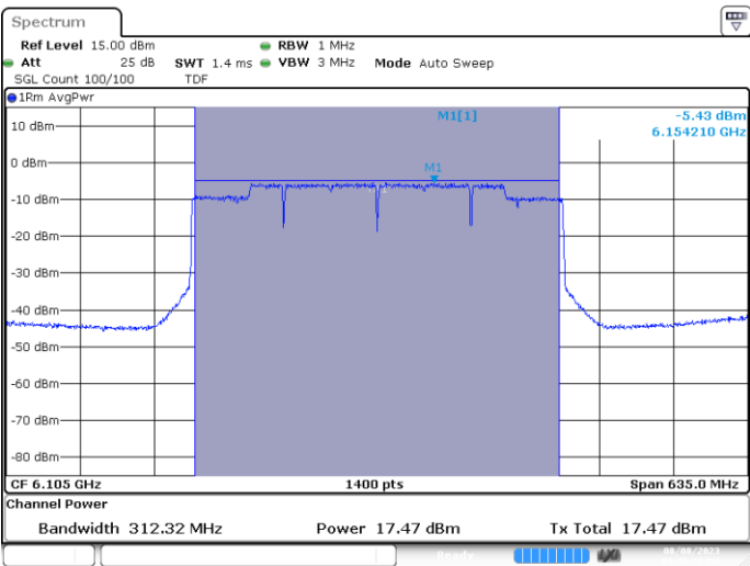
MIMO A-802.11be-320MHz-Ch31-6105MHz-MCS0
