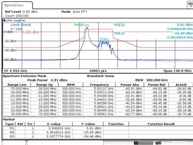
SISO-B, 802.11ax/be20-MCS0, Ch1-2m-0
