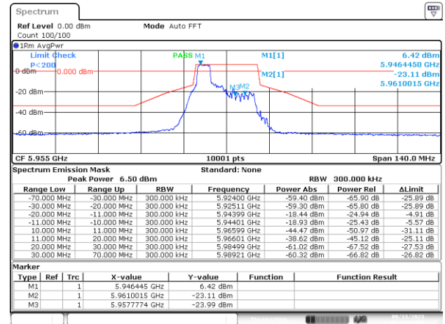
SISO-B, 802.11ax/be20-MCS0, Ch1-4m-37
