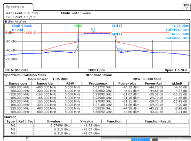
MIMO A-802.11be-320MHz-Ch31-6105MHz-MCS0
