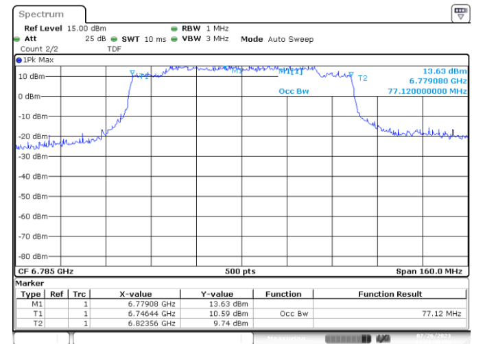
UNII7 SISO A 802.11ax/be80 ch67 6785MHz 99%
