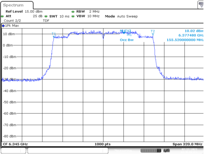
UNII5 MIMO A 802.11ax/be160 ch79 6345MHz 99%
