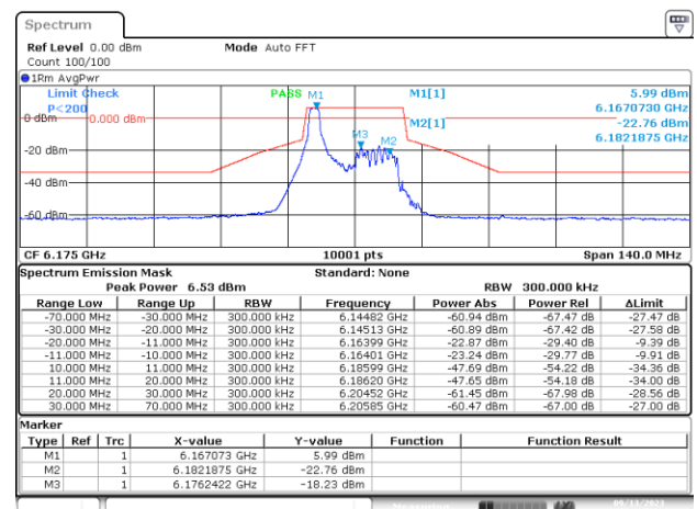
SISO-B, 802.11ax/be20-MCS0, Ch45-2m-0
