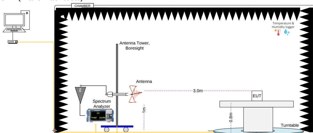
Radiated Setup 30MHz - 1GHz (Transmitter tests)
