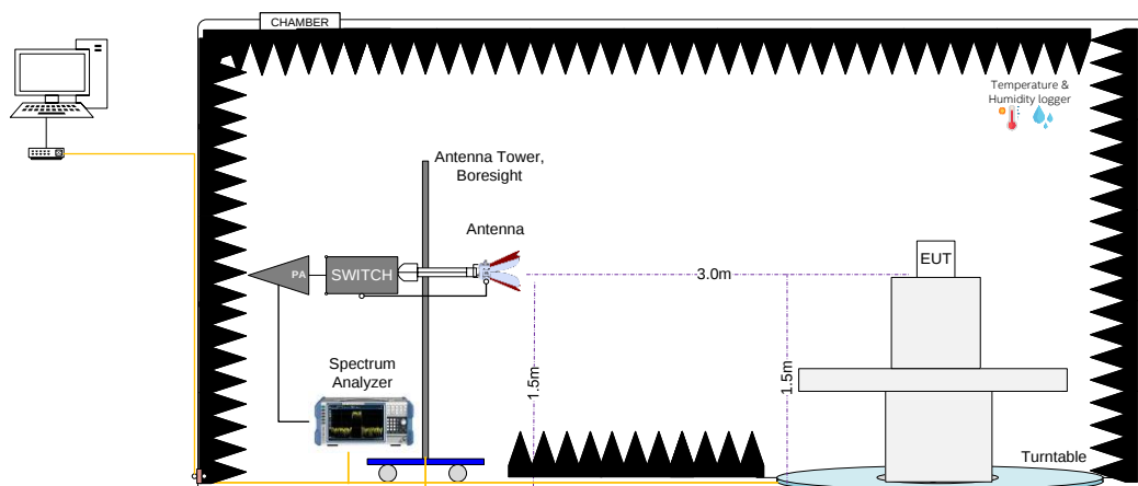
Radiated Setup 1GHz – 11GHz (Transmitter tests)
